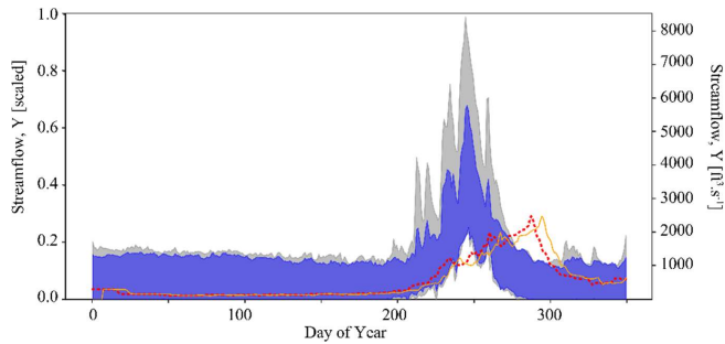
1160 Figure E1. Time series comparing the observed streamflow for water year 1995 (red) with the persistence baseline (orange), posterior predictive check from standalone SBI (blue), and simulations drawn from the full parameter space (gray).
