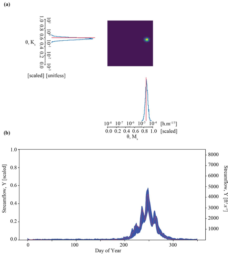
Figure 6. Results of parameter inference and posterior predictive check on synthetic observation Y_{\text{Obs\_ParFlow\_A}} in Experiment 3 ('boosted' case). Subplots (a) and (b) show accurate parameter inference that is somewhat less precise, resulting in a wider but still well-constrained posterior predictive check.
