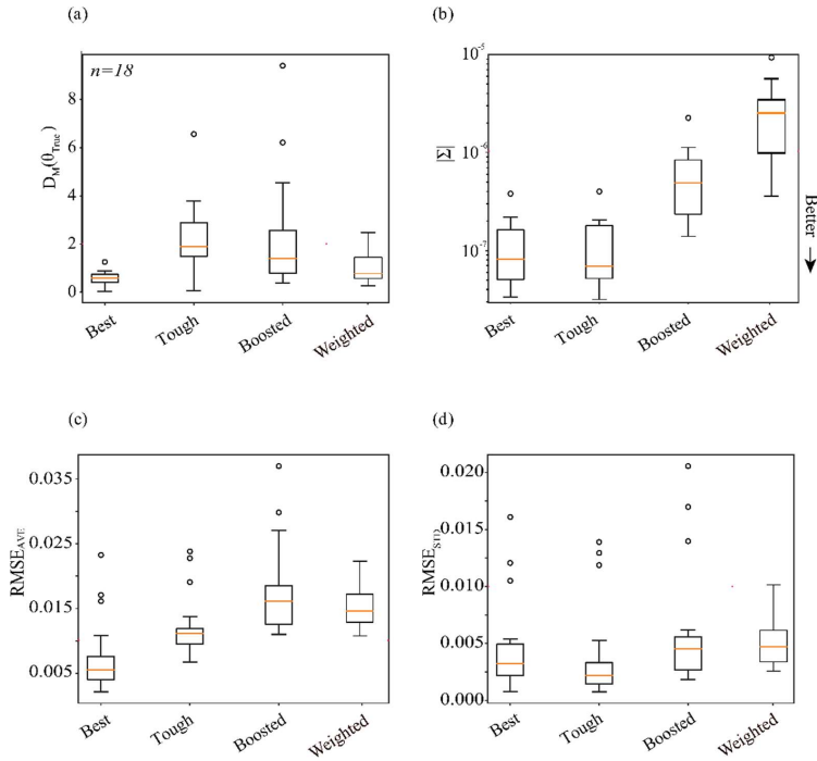
855 Figure 8: Comparative plots showing the performance of simulation-based inference of parameters and predicted quantities across a set of n=18 test data. We compare the results of Experiments 1 ('base' case), 2 ('tough' case), 3 ('boosted' case), and 4 ('weighted' case). Subplots (a) and (b) show the accuracy and precision of parameter inference. Accuracy is shown in subplot (a) via the Mahalanobis Distance of the posterior parameter density. Precision is shown in subplot (b) via the Determinant, |\Sigma| . Subplots (c) and (d) show the accuracy and precision of the posterior predictive check. Subplot (c) shows the average of the error, RMSE_{\text{AVE}} of streamflow ensembles relative to 'truth', which can be thought of as a measure of accuracy. Subplot (d) shows the standard deviation of the error, RMSE_{\text{STD}} of streamflow ensembles, which can be thought of as a measure of precision. Values closer to the x-axis are more desirable. 860
