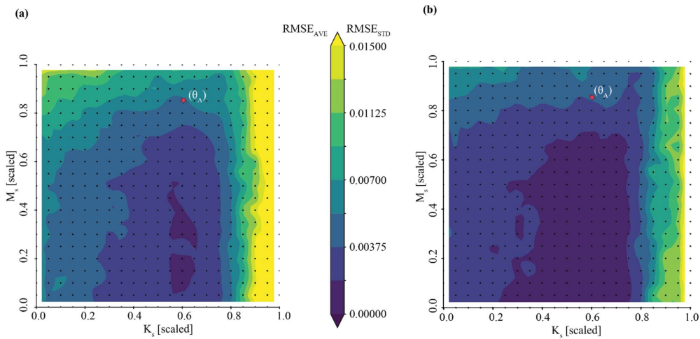
1125 Figure D2. Posterior predictive check for many observations: Once parameters are inferred, the posterior can be drawn ( n=50 ) to generate probabilistic streamflow ensembles. This figure shows the performance of streamflow ensembles derived from SBI at 441 locations across parameter space. Subplot (a) shows the average of the error ( RMSE_{AVE} ) of streamflow ensembles relative to 'truth', which can be thought of as a measure of accuracy. Subplot (b) shows the standard deviation of the error ( RMSE_{STD} ) of streamflow ensembles, which can be thought of as a measure of precision. Streamflow ensembles are evaluated against the 'true' synthetic streamflow time series generated by the surrogate simulator, where blue is better. 1130
