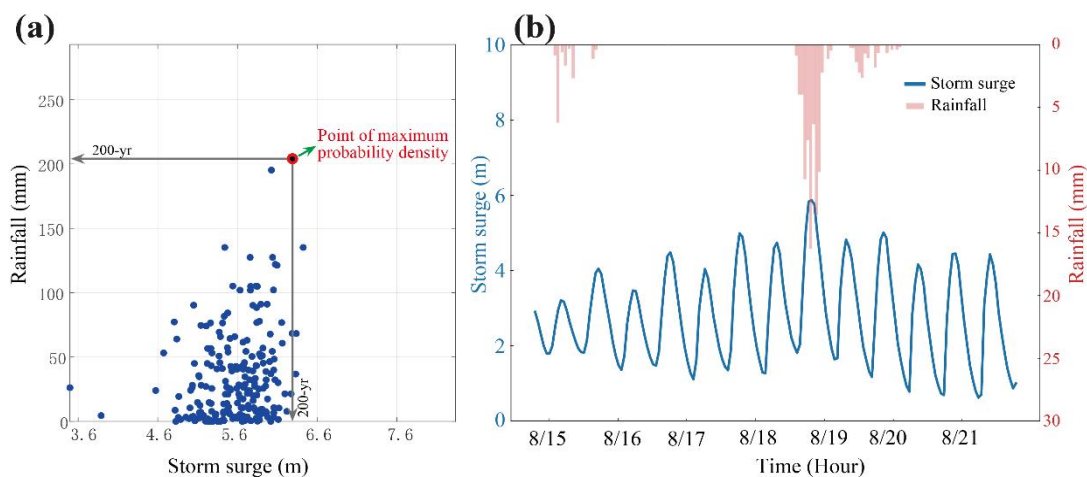
195 Figure 5: (a) Bivariate statistical analysis of joint distribution with “AND” scenario between peak storm surge and corresponding cumulative rainfall by MvCAT; (b) The boundary conditions for the hydrodynamic model based on a scenario of no time lag between the peak storm tide and the corresponding cumulative rainfall observed during typhoon Winnie.
