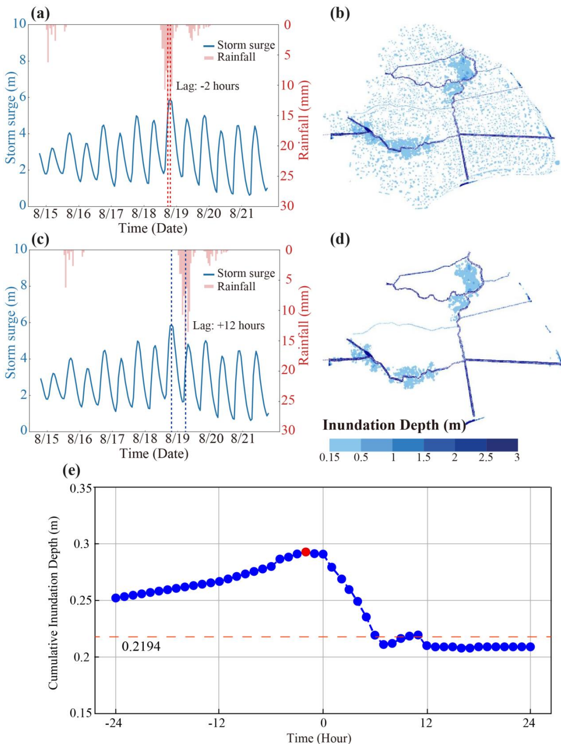
Figure 6: Cumulative inundation depth under combined impact of storm surge and rainfall with -2 and +12 hour lags. (a) The boundary conditions of -2h time lag between the peak storm surge and the corresponding cumulative rainfall; (b) Flooding
