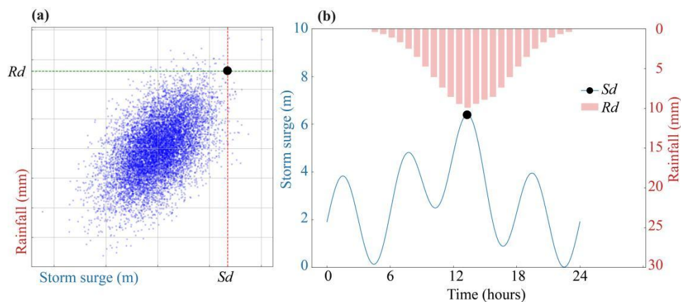
145 Figure 4: Sketch graph to illustrate the combination of the copula and SFA method. Panel (a) represents the dependence model of surge peaks and accumulated rainfall to derive their respective design values S_d and R_d . Panel (b) illustrates the amplified signals where the highest peak corresponds to the design value S_d and the volume of rainfall corresponds to the design value R_d .
