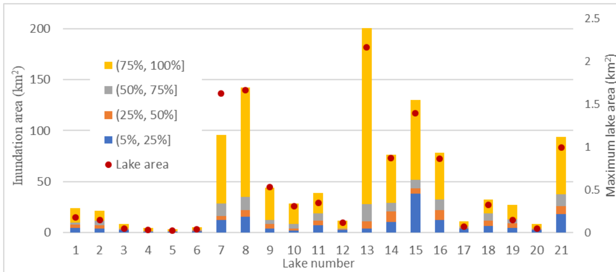
395 Fig 6 Inundation area (km 2 ) at different levels of inundation probabilities and maximum lake area (km 2 )
