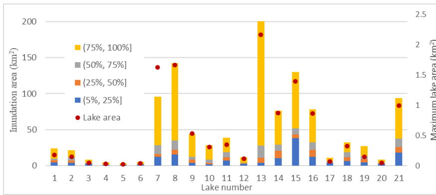
410 Fig 6 Inundation area (km 2 ) at different levels of inundation probabilities and maximum lake area (km 2 )
