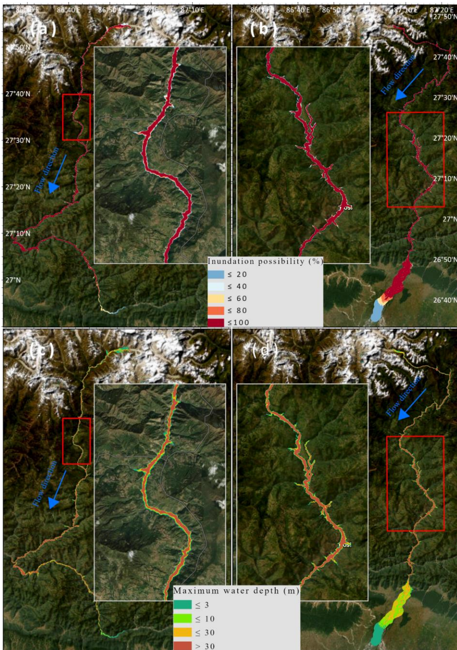
395 Fig 5 GLOF inundation probability for (a) Imja Tsho Lake and (b) Lower Barun Lake, and maximum water depth for (c) Imja Tsho Lake and (d) Lower Barun Lake under respective theoretical worst situation i.e., the complete breach of dam height — lake water will be released . (The basemaps used were accessed from ArcGIS Online Basemap provided by Esri.)
