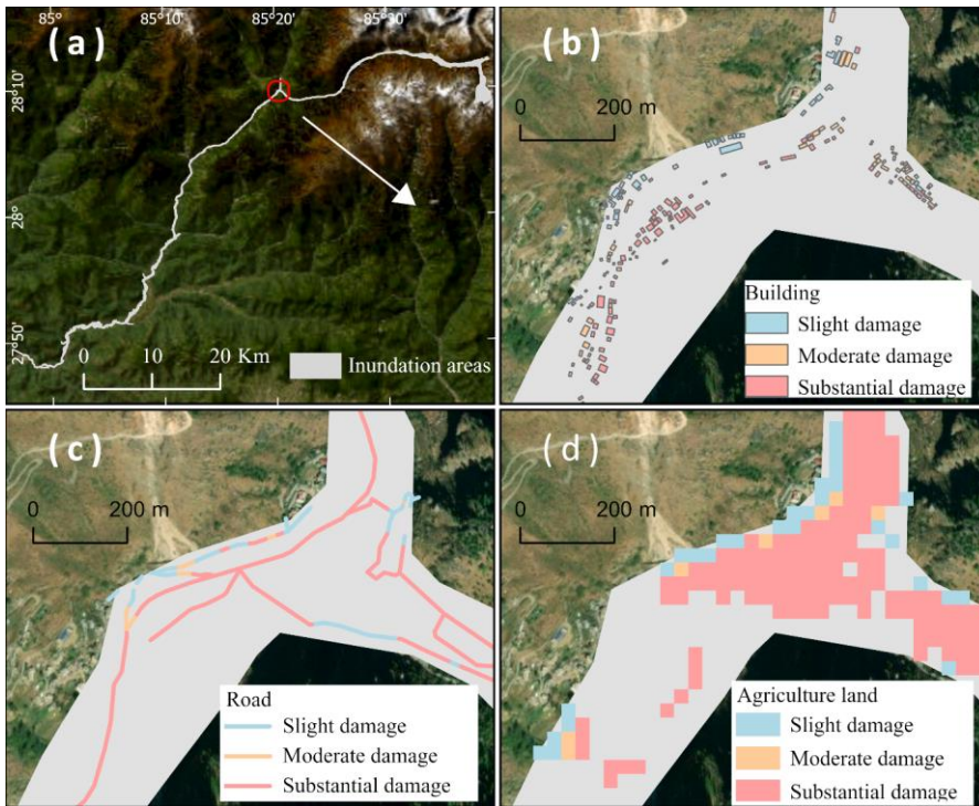
Fig 8 Damage to buildings, roads, and agricultural land caused by the theoretical most serious GLOF due to Lake Anonymous 12 ( Basemap sources: Earthstar Geographics and Maxar )
