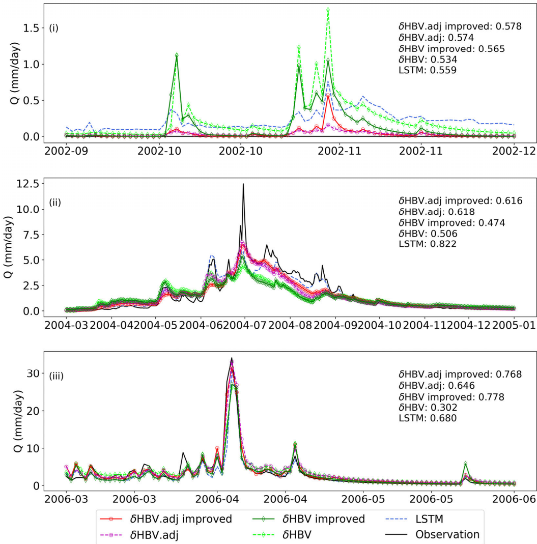
480 Figure 6: The time series of streamflow simulations from models and observation at locations annotated in Figure 4 and Figure 5. KGE values of models in the whole testing period are listed in the subfigures.
