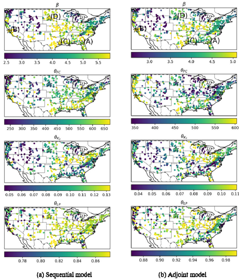
Figure 7: Map of the optimized parameter \beta , field capacity, \theta_{FC} , the recession coefficient of lower subsurface zone, \theta_{K_2} , and the wilting point, \theta_{LP} , from (a) sequential model and (b) adjoint model. The sites annotated in the maps represented by star-shaped points labeled with letters A-D, represent the locations for the plots in Figure 8.
