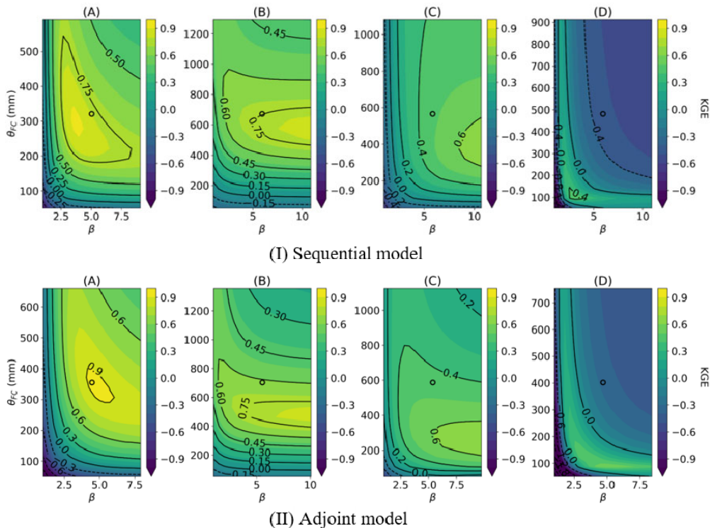
565 Figure 8: Impact of numerical schemes on the KGE surface of HBV model: The contour of KGE calculated from the (I) sequential model and (II) adjoint model on the 2D slice of field capacity ( \theta_{FC} ) and parameter \beta . The predicted parameter
