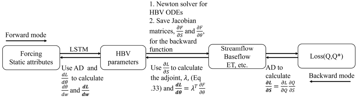
355 Figure 2: Schematic view of the forward code for streamflow prediction and backward code for gradient backpropagation. In the backpropagation process, the steps utilizing automatic differentiation (AD) can be automatically executed by PyTorch. We only need to address the adjoint calculation and pass \frac{dL}{d\theta} for backpropagation to the subsequent step. The bolded derivatives represent the outputs of each step in the backward mode.
