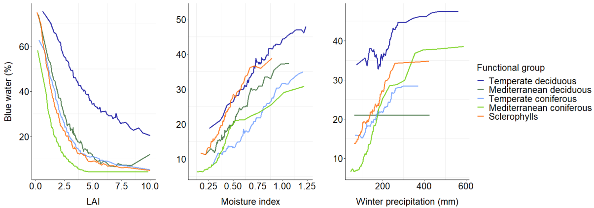
Figure 76. Partial dependence plots for the three main predictor variables (A, LAI; B, Climatic moisture index; C, Winter precipitation) and their effect on blue water percentage for the different functional groups.
