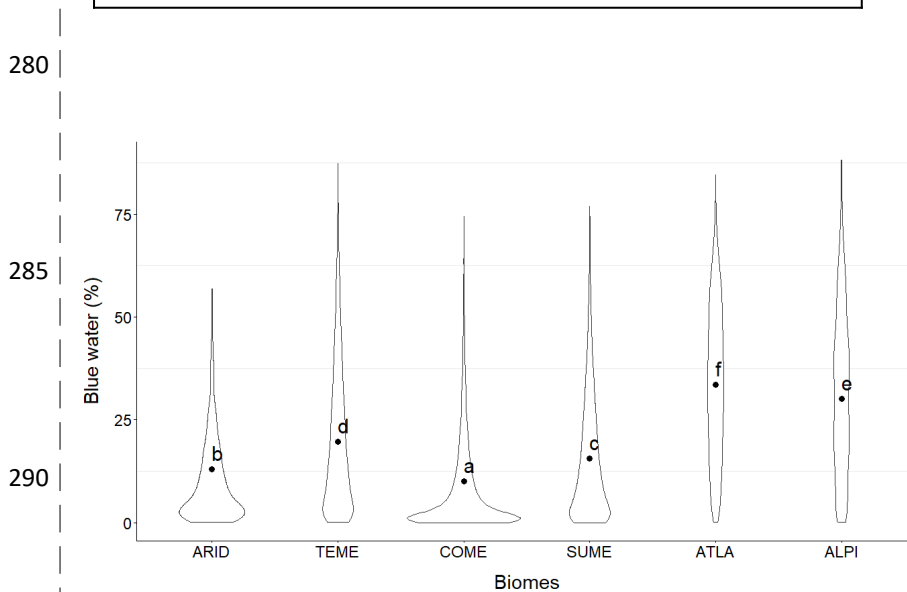
Figure 32. Percentage of blue water in the different biomes. Different letters denote significant differences among biomes ( p < 0.01 ) after Tukey's test. Abbreviations of the biomes: ARID, Arid; TEME, Temperate Mediterranean; COME, Continental Mediterranean; SUME, Submediterranean; ATLA, Atlantic; ALPI, Alpine.
