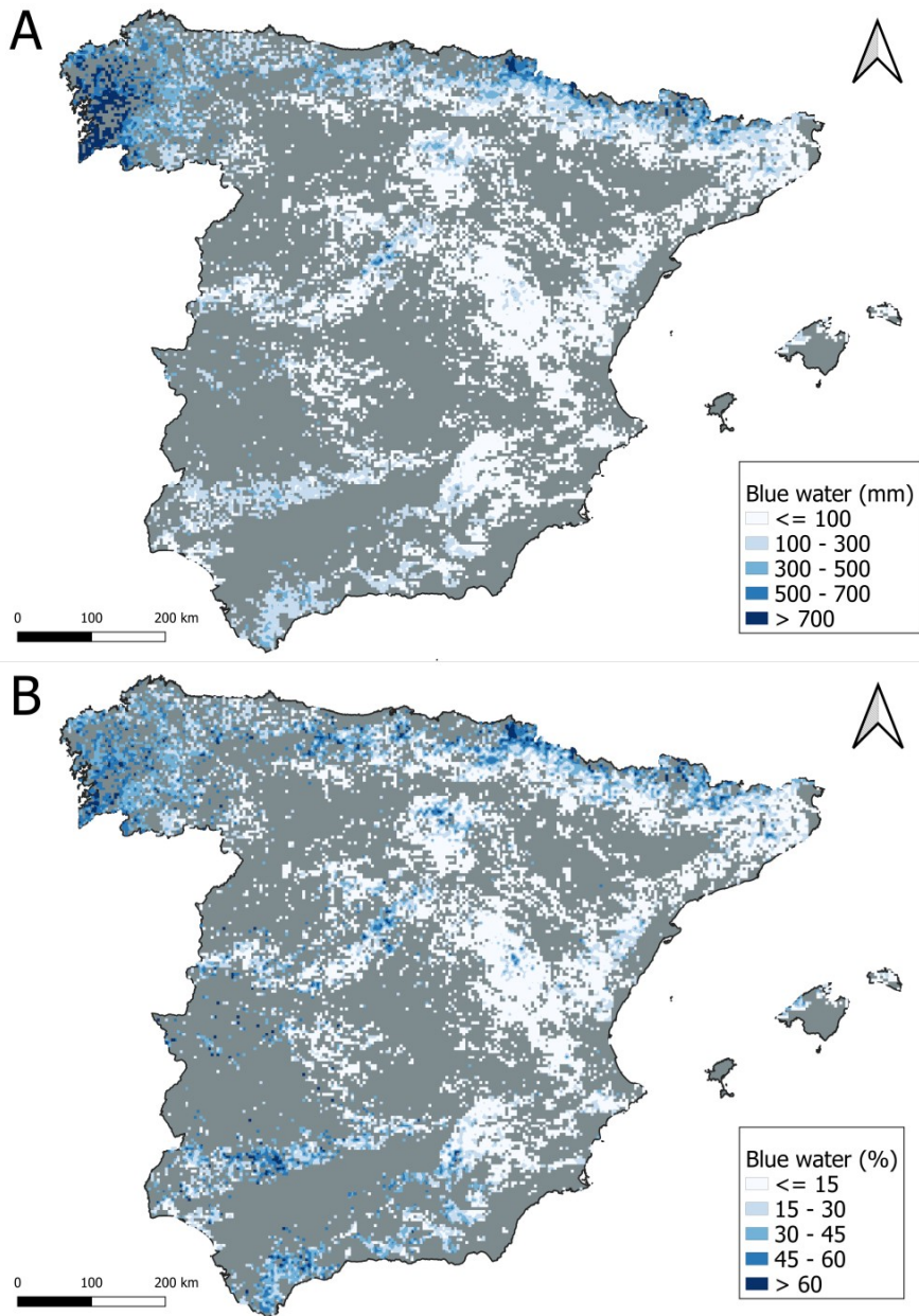
275 | Figure 24. Total (A) and relative (B) blue water in the Spanish Peninsula and Balearic Islands. In grey, no forest covers. Maps were realized with a rasterization of the SFI3 plots results at 1 km 2 .
