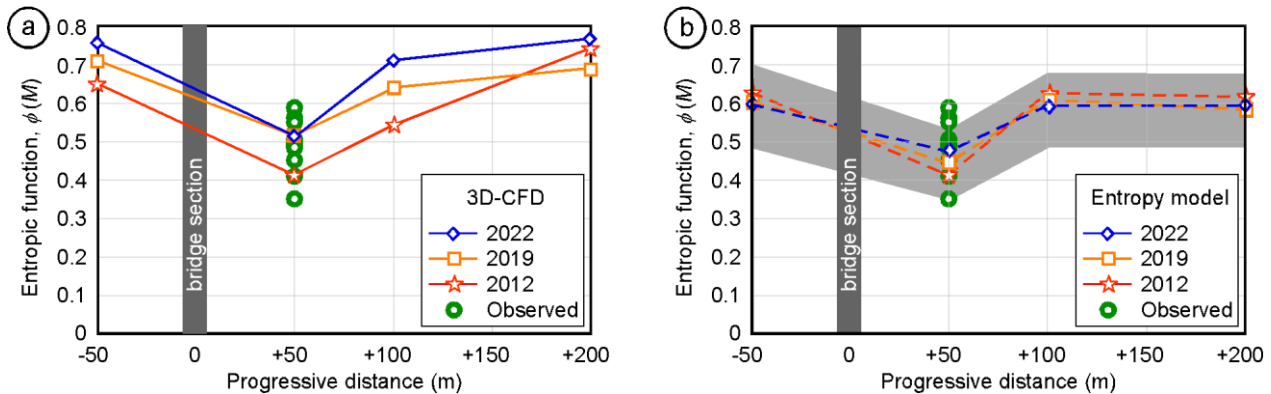
285 Figure 3. Entropic function \phi(M) , for the different simulated scenarios, as a function of the distance from the bridge (positive downstream), (a) computed from the 3D-CFD flow fields and (b) estimated with Eq. (4), where the lines refer to the average values and the gray band is obtained by varying the reference height y_0 in Eq. (4) within the expected range. Green circles refer to data derived from velocity distributions measured with the current meter just downstream of the bridge.
