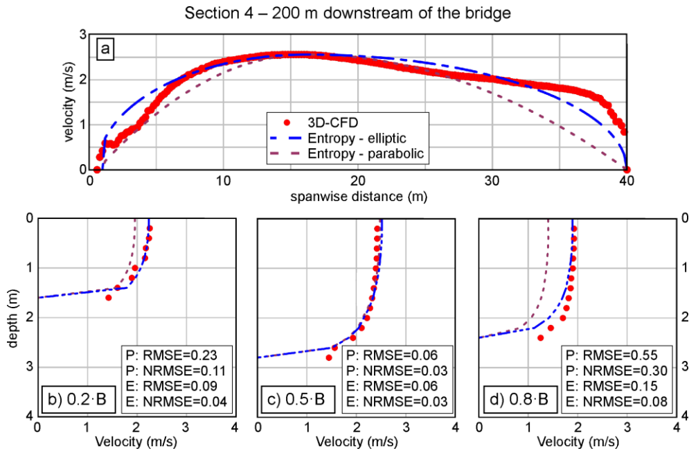
410 Figure 10. Flood event of 2022, cross-section 4 (200 m downstream of the bridge). Spanwise distribution of the surface velocity (a); comparison of vertical distributions of velocity at 0.2B (b), 0.5B (c), and 0.8B (d).
