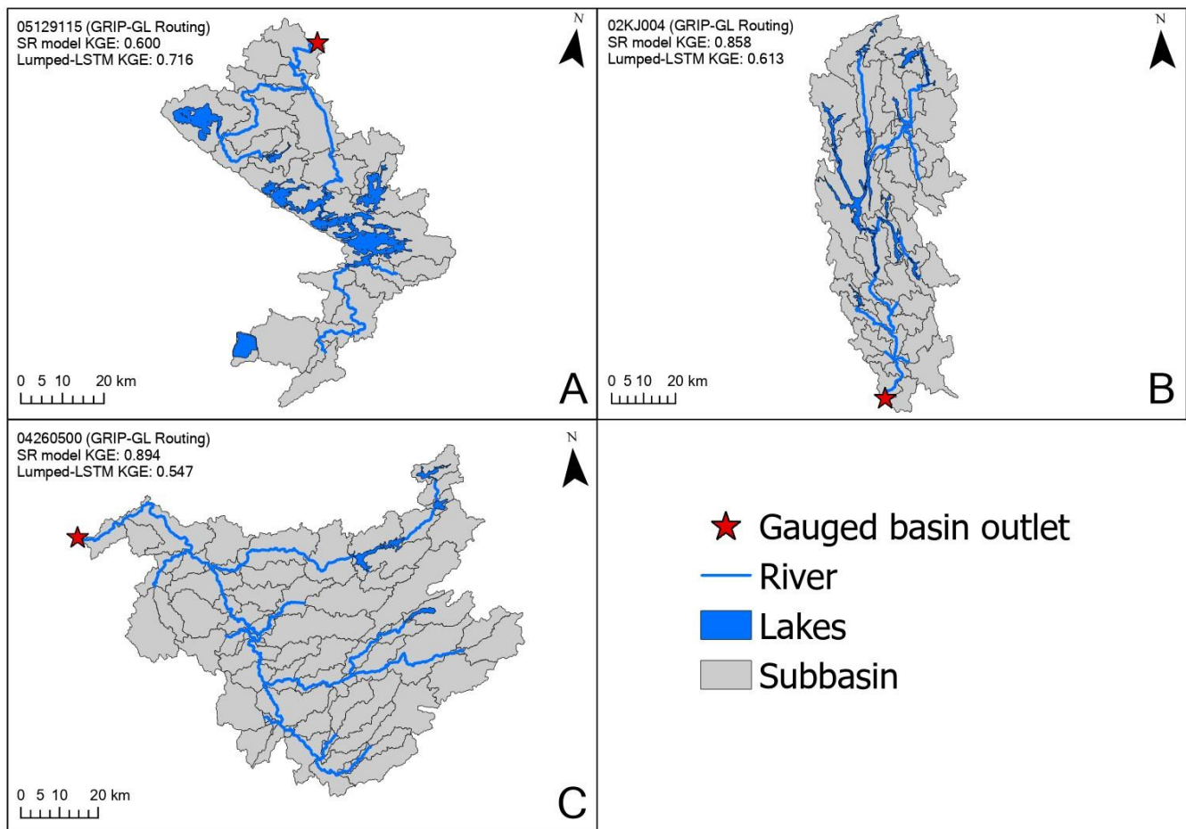
Figure 8. Comparison of the routing networks of 3 large Non-GRIP-GL basins to illustrate the variation in different lake densities. (A) Gauged basin 05129115 (5 lakes, 14% of basin is covered by lakes). (B) Gauged basin 02KJ004 (11 lakes, 10% of basin is covered by lakes) and (C) Gauged basin 04260500 (4 lake, 4% of basin is covered by lakes). The three illustrated routing networks were delineated to mimic the GRIP-GL routing delineation strategy.
