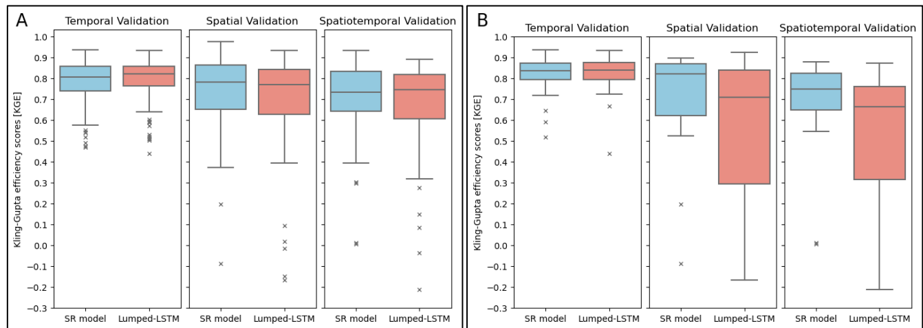
Figure 4. Boxplots of KGE validation scores for the SR model (blue) and the lumped LSTM (red). (A) The results of all basins participating in each validation experiment. (B) The results of basins with a size larger than 2000 km 2 .
