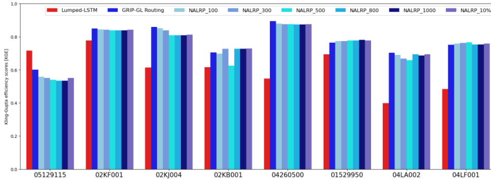
Figure 6. Overall model performances as adopting different routing network delineations in the 8 large Non-GRIP-GL basins, during the whole study period 2000-2017. The basins are sorted from left to right in ascending order according to their sizes, from smallest (2343 km 2 ) to largest (6760 km 2 ).
