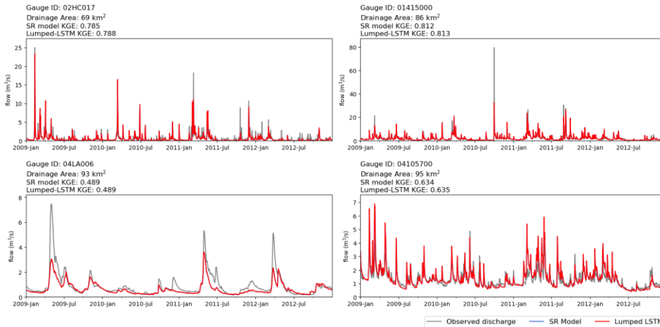
370 Figure 3. Comparison of observation (grey), lumped LSTM prediction (red) and SR model prediction (blue) for the 4 small Non-GRIP-GL basins. KGE values over the period from 2001 to 2017 are given for each basin.
