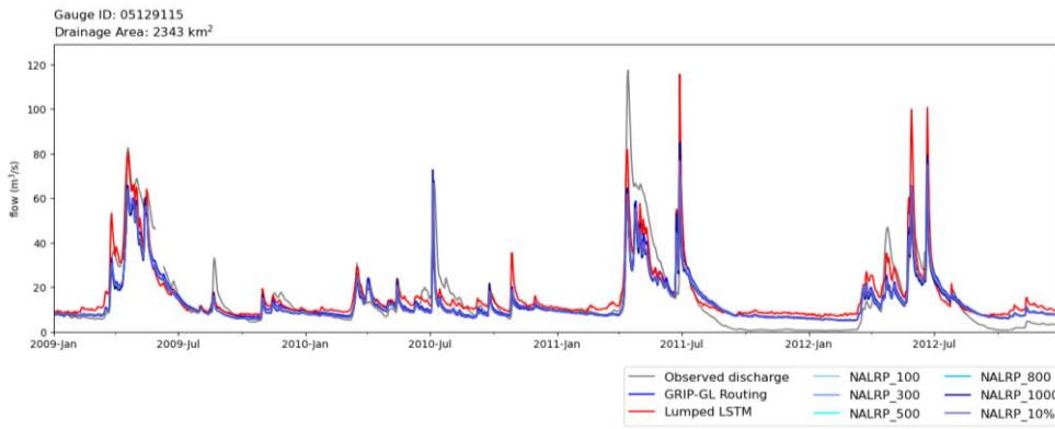
Figure 7. Comparison of the time series of observation (grey), lumped LSTM prediction (red) and SR model predictions with different routing networks for the Vermilion River basin 05129115. Note that the lines of NALRP time series all follow extremely similar trends as the GRIP-GL Routing series and thus are not distinguishable.
