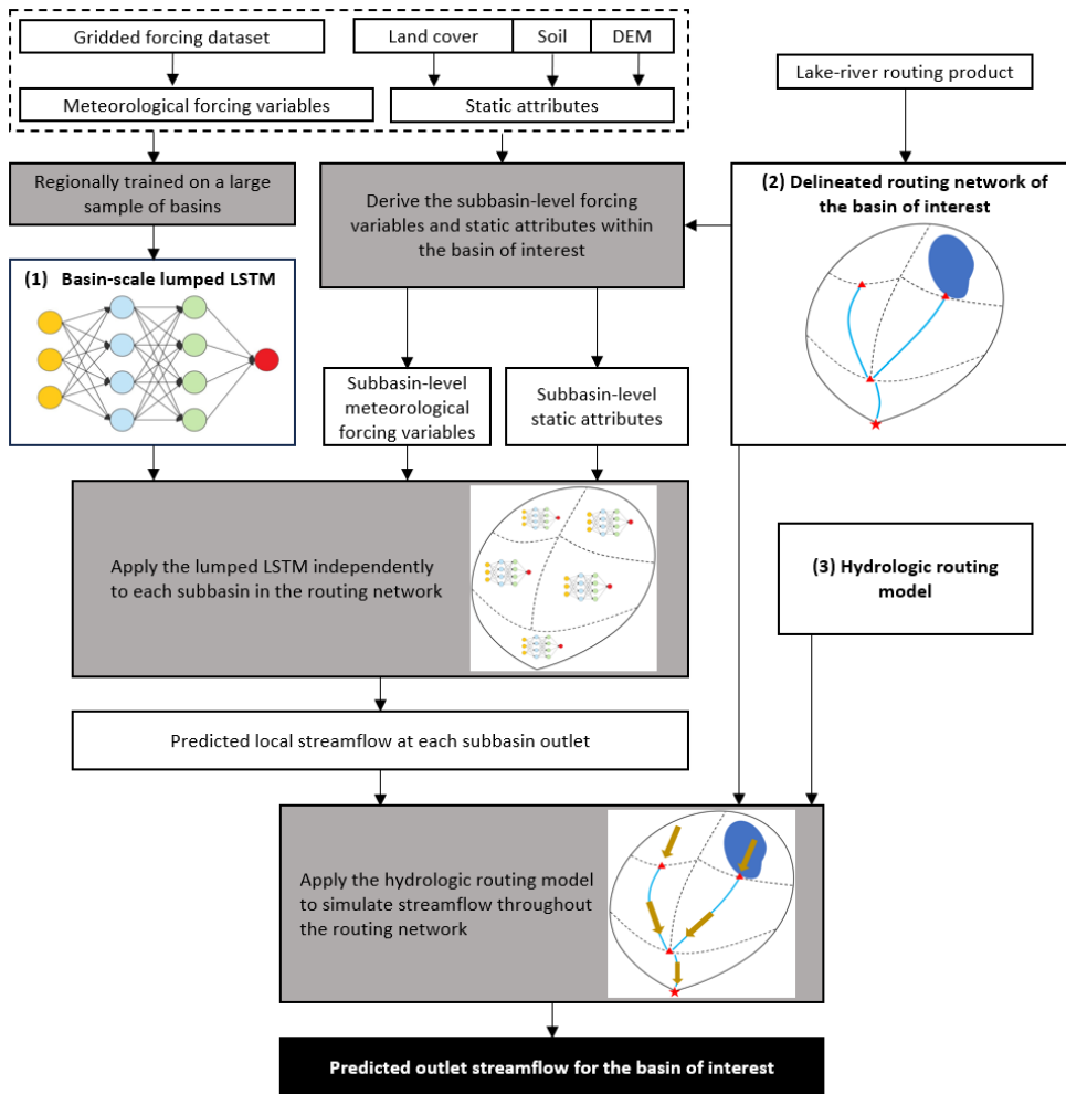
Figure 1. The spatially recursive model workflow for an arbitrary basin of interest. Note the workflow is conceptually model-agnostic (e.g., where the predictor model (lumped LSTM) can be replaced by another data-driven model), while each component needs to generate outputs compatible with other components. The three components of the SR-model are numbered in the order that they are applied in the workflow. Components with multiple arrows are utilized multiple times throughout the workflow.
