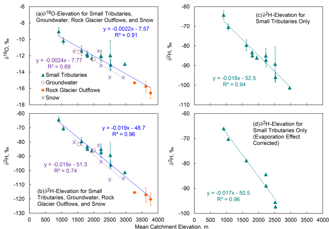
Figure 7. Variation of isotopic composition with mean catchment elevations: (a) and (b) for \delta^{18}\text{O} and \delta^2\text{H} values, respectively, in small tributaries (catchment area < 122 \text{ km}^2 ), groundwater with estimated source water elevations (Crane Flat and Hodgdon Meadow), and rock glacier outflows, along with snow and rain samples. The blue solid line shows the linear trend for small tributaries, groundwater and rock glacier outflows and the dashed purple line for snow and rain. (c) for \delta^2\text{H} values in small tributaries without groundwater and rock glacier outflows; and (d) for \delta^2\text{H} values in small tributaries with evaporation effect corrected by local meteoric water line. The number of samples in (d) is less than in (c) due to the lack of samples to establish a significant relationship between \delta^2\text{H} and \delta^{18}\text{O} values for the last four tributaries listed in Table 1.
