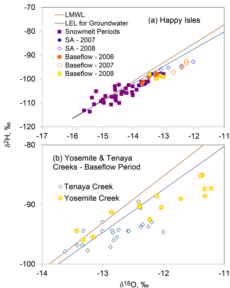
670 Figure 10. Scatter plot of \delta^2\text{H} vs. \delta^{18}\text{O} for (a) Merced River at Happy Isles during different periods and (b) comparison between Tenaya Creek and Yosemite Creek during the baseflow period. Local meteoric water line (LMWL) and evaporation line (LEL) of groundwater are also shown as references.
