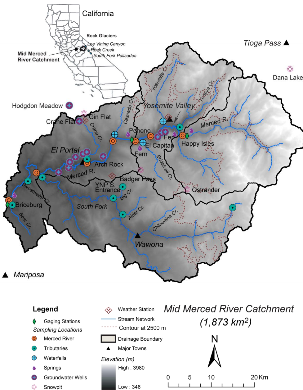
155 Figure 1. Sampling locations for snow, stream water, spring water and groundwater in the mid Merced River catchment, along with stream gages and meteorological stations, topography, stream network and drainage boundary. The inset map shows the locations of the mid Merced River catchment in California and rock glaciers outside the catchment. The elevation contour at 2,500 m (brown dashed line) is also marked to show the upper boundary of the snow-rain transition zone.
