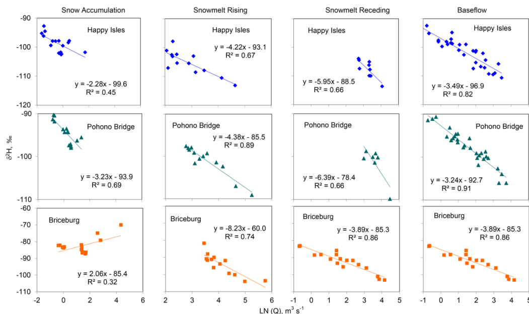
370 Figure 5. Correlation between \delta^2\text{H} values in stream water and stream flow (natural logarithmic values) during four periods at Happy Isles, Pohono Bridge and Briceburg.
