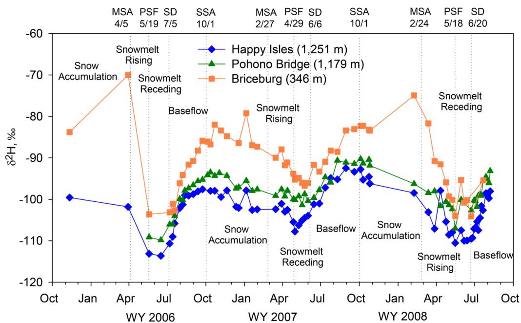
350 Figure 4. Variation of \delta^2\text{H} values in stream water from water years 2006 to 2008 at Happy Isles, Pohono Bridge and Briceburg. Dates marked by gray, dotted vertical grids are the same as in Figure 2 with addition of peak stream flow (PSF). Four periods were also marked wherever space is allowed.
