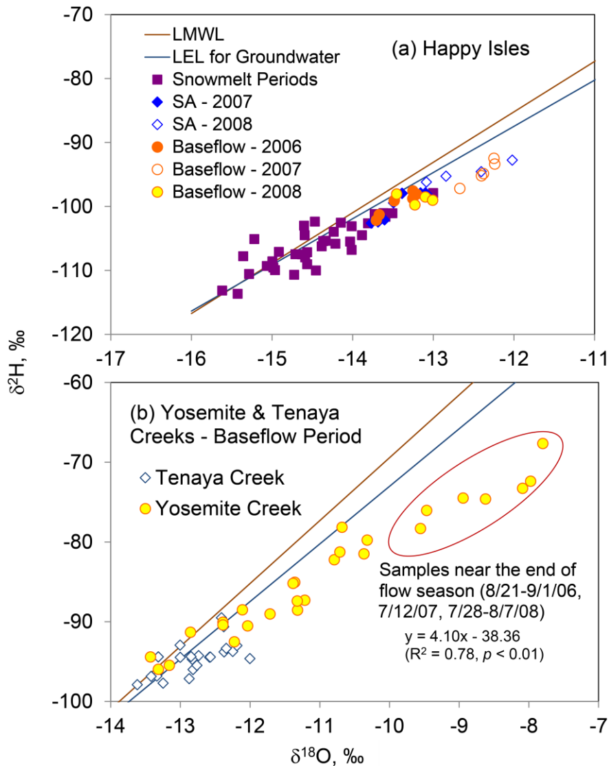
670 Figure 10. Scatter plot of \delta^2\text{H} vs. \delta^{18}\text{O} for (a) Merced River at Happy Isles during different periods and (b) 675 comparison between Tenaya Creek and Yosemite Creek during the baseflow period. Local meteoric water line (LMWL) and evaporation line (LEL) of groundwater are also shown as references. Highlighted by a red oval are samples collected in Yosemite Creek near the end of flow seasons from 2006 to 2008, along with a linear regression equation (Samples collected in Tenaya Creek near the end of flow seasons at Yosemite Creek did not have a significant relationship ( R^2 = 0.09, p = 0.47 ) between \delta^2\text{H} and \delta^{18}\text{O} ).
