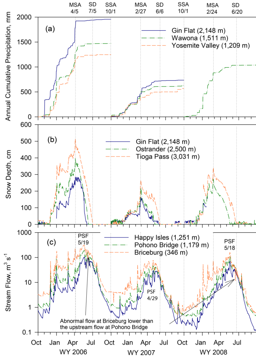
265 Figure 2. Hydrometeorology of the mid Merced River catchment for (a) daily accumulated precipitation, (b) daily snow depth, and (c) daily stream flow. Note the abnormal flow occasionally measured at Briceburg, which is lower than upstream flow at Pohono Bridge. Also note the lack of precipitation data in 2008 at Gin Flat and Yosemite Valley and snow depth data in most of 2008 at Gin Flat and in February 270 2008 at Tioga Pass. The grey dotted vertical grids mark the dates of the maximum snow accumulation (MSA), snow depletion (SD) at Tioga Pass, and start of snow accumulation (SSA) as October 1 each year; Dates of peak stream flow (PSF) were also marked in (c). Other than Gin Flat, the two other sites are not the same in (a) and (b), as precipitation and snow depth data were not available in the same sites.
