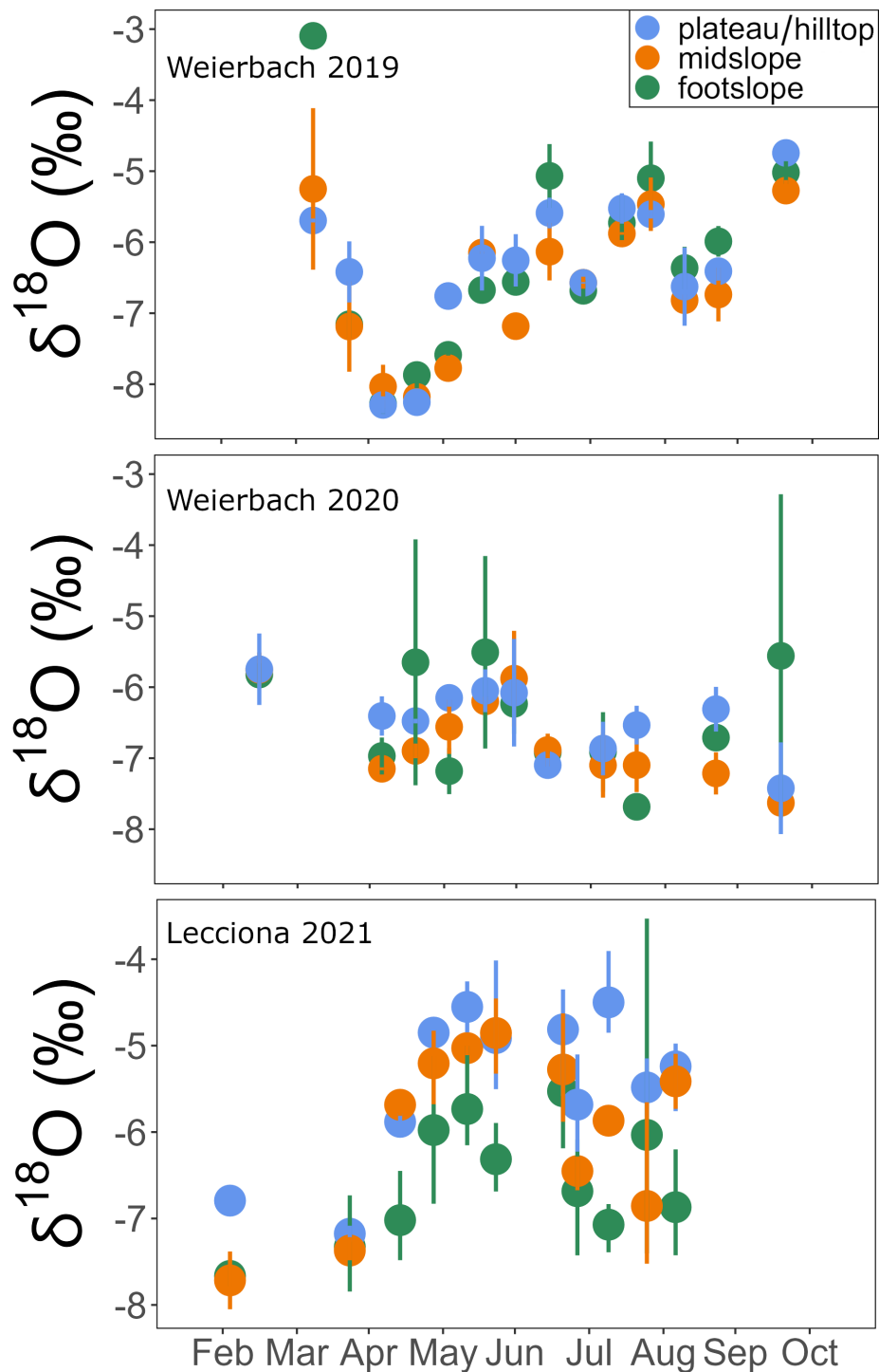
Figure A4. \delta^{18}\text{O} of xylem water for each sampling campaign across 2019 and 2020 growing season in the Weierbach catchment and 2021 in the Lecciona catchment. Data were averaged by location. Solid dots represent the mean, the whiskers indicate the confidence interval (95%).
