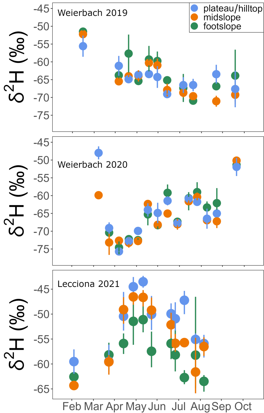
Figure A5. \delta^2\text{H} of xylem water for each sampling campaign across 2019 and 2020 growing season in the Weierbach catchment and 2021 in the Lecciona catchment. Data were averaged by location. Solid dots represent the mean, the whiskers indicate the confidence interval (95%).
