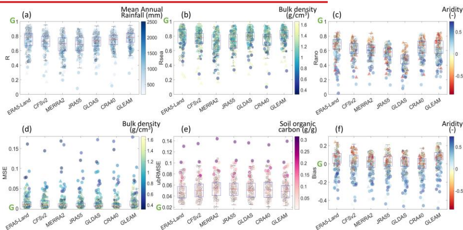
Figure 5: Influential factors in explaining the reanalysis product performance. The shape of the dots denotes the CRNS sites from different networks (UK: circle; mainland Europe: square; USA: triangle; Australia: diamond), while the colour of the dots represents the values of possible factors for each site. The green letter G denotes the good performance of the statistical metric values.
