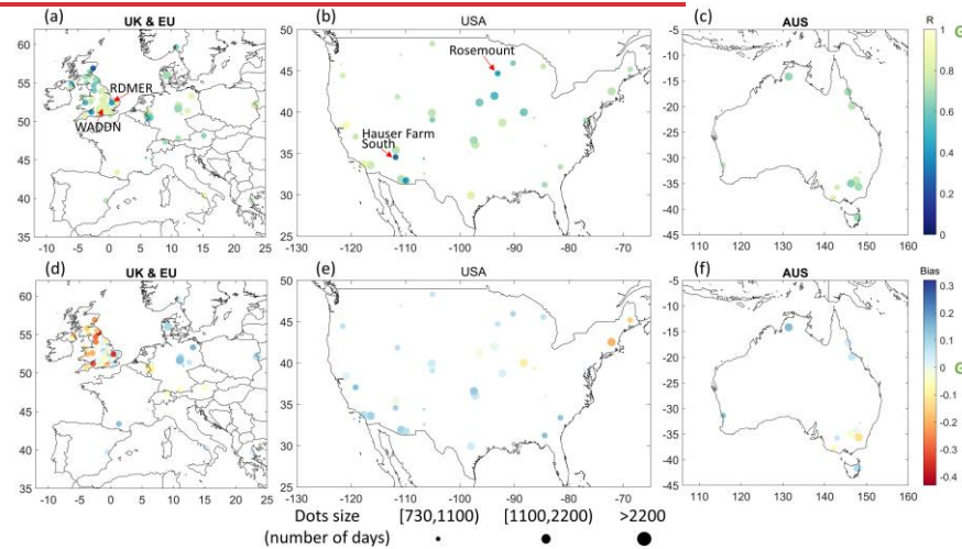
Figure 3: Spatial distribution of all 87 products average performance in terms of statistical metrics R and Bias . The green letter G denotes the statistical metric values with good performance. The size of the dots in the map indicates the length of the measurements (i.e., number of days).
