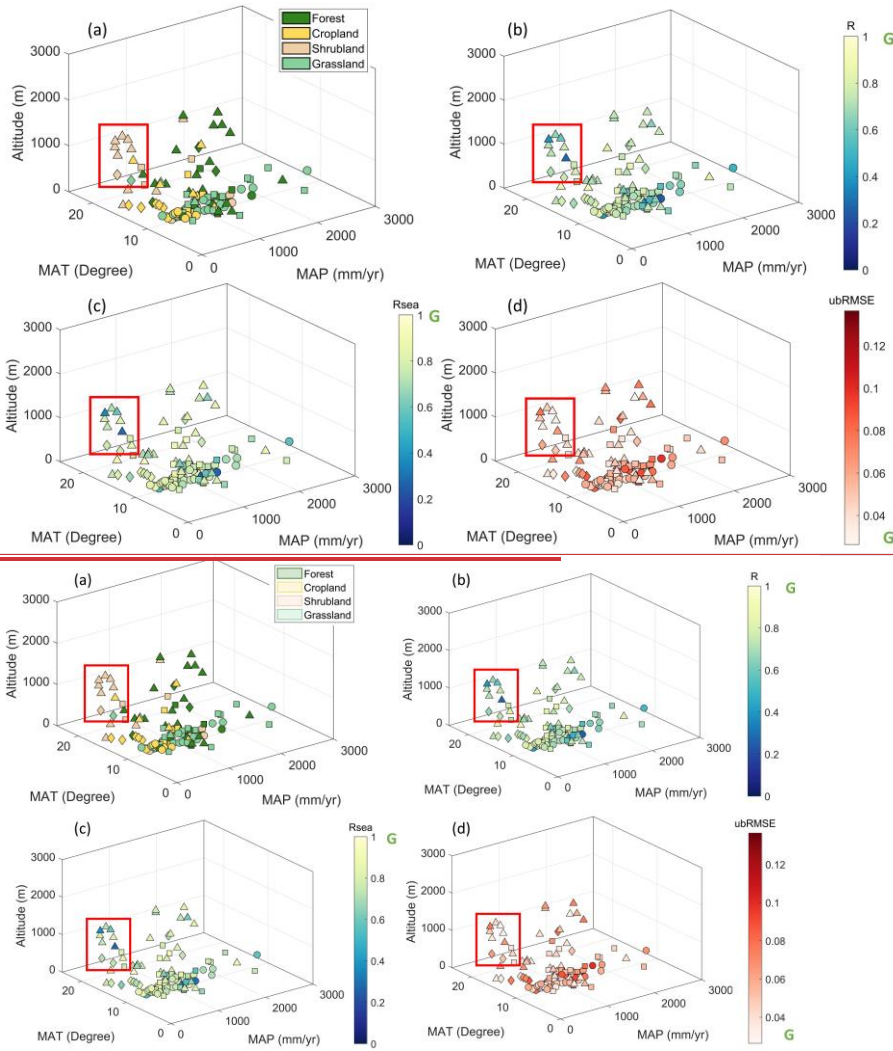
Figure 6: Average statistical metrics R , R_{sea} and ubRMSE performance of all 87 products under different land cover types, altitude, mean annual precipitation and mean annual temperature. The shape of the dots denotes the CRNS sites from different networks (UK: circle; mainland Europe: square; USA: triangle; Australia: diamond). The colour of dots in (a) denotes different land cover types, while the colour in other subplots represents the statistical metric values. MAT stands for mean annual temperature, and MAP is mean annual precipitation.
