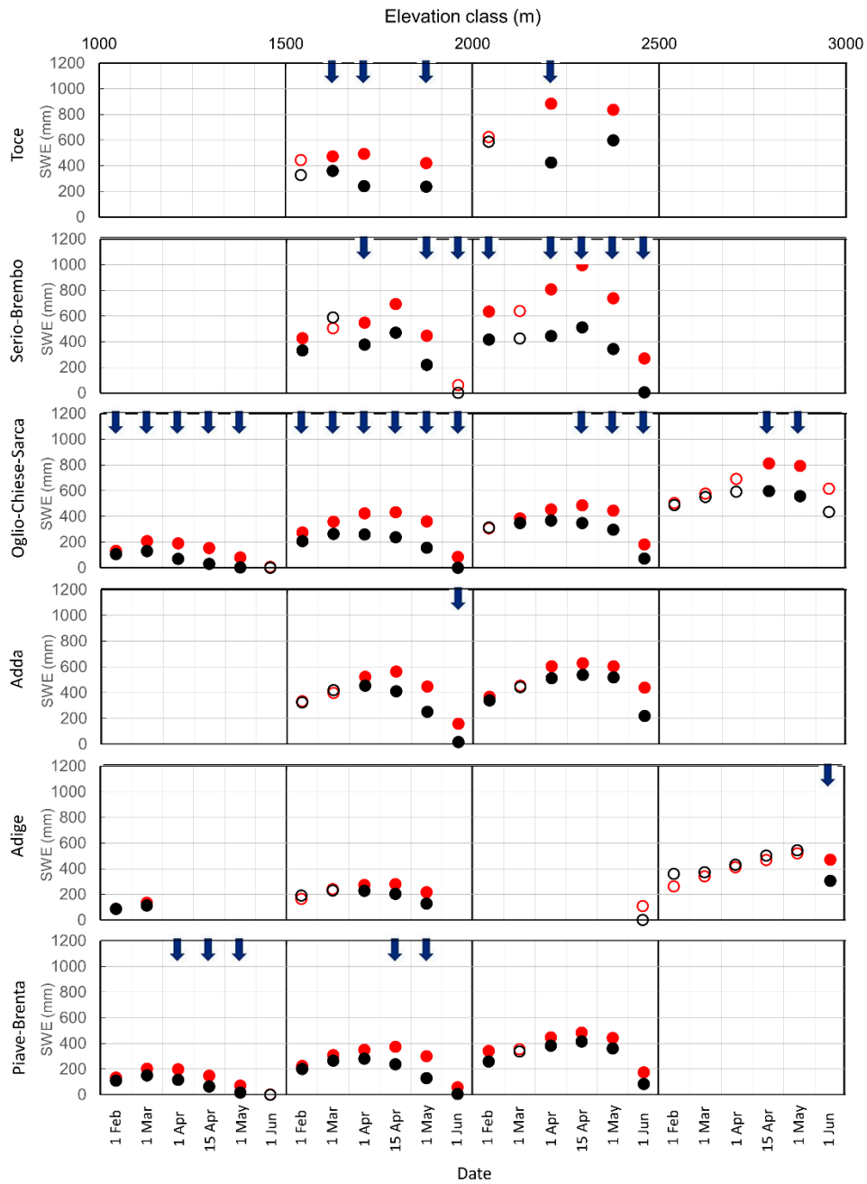
700 Figure 5: Average snow water equivalent (SWE) in the 1967-1993 (red circles) and in 1994-2020 (black circles) periods are plotted for each elevation class in the six observation campaigns dates (1 Feb, 1 Mar, 1 Apr, 15 Apr, 1 May, 1 Jun). Statistically significant ( p \leq 0.01 , Mann-Kendall test) trends of the entire 1967-2020 period are sketched as upward (downward) blue arrow for increasing (decreasing) trends. Circles are filled if the difference of SWE between the two periods is statistically significant ( p \leq 0.01 , Mann-Whitney test).
