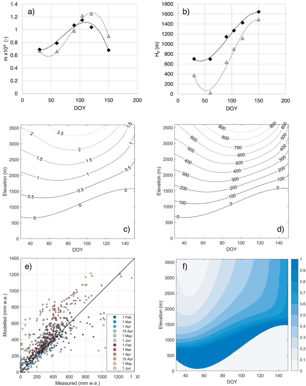
715 Figure 8: Slope m (a) and null snow depth elevation H_0 (b) as function of the day of the year for the sub periods 1967-1993 (grey triangles) and 1994-2020 (black diamonds). Dotted lines represent the third order polynomial fitting curve (Equation 4 and 5). 720 Counter plots of snow depth (c) and snow water equivalent (d) in the time-elevation (DOY-H) space for the 1994-2020 sub period. In panel e) the scatter plot reporting measured and modelled climatological SWE in the Oglio-Chiese-Sarca macro basin for the first (red) and second (blue) sub periods. Panel f) reports the comparison between the modelled climatological SWE in the first and in the second sub periods, expressed as relative decrease of SWE.
