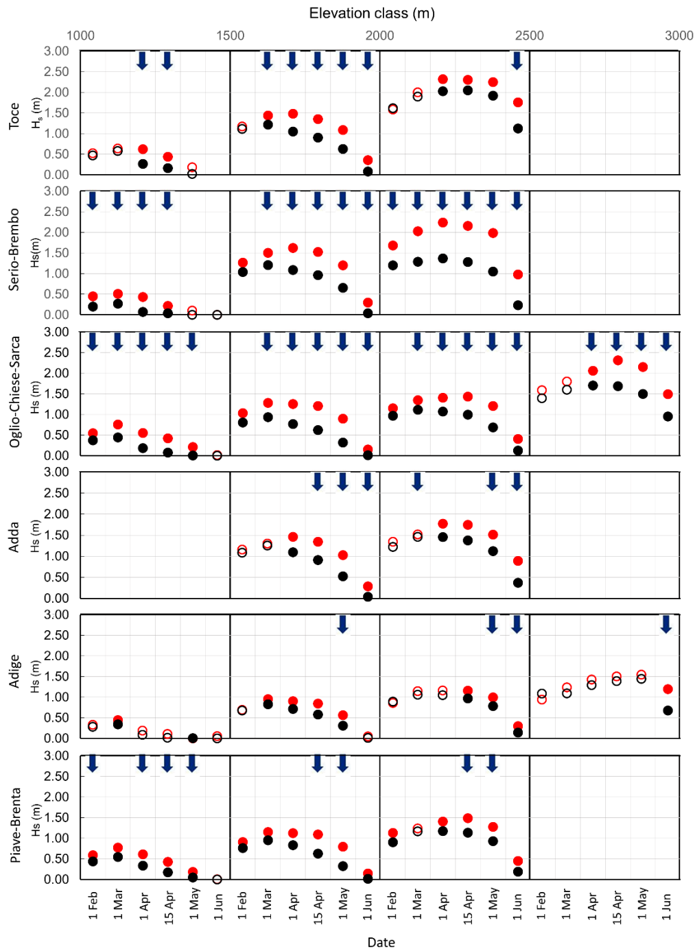
690 Figure 3: Average snow depth (Hs) in the 1967-1993 (red circles) and in 1994-2020 (black circles) periods are plotted for each elevation class in the six observation campaigns (1 Feb, 1 Mar, 1 Apr, 15 Apr, 1 May, 1 Jun). Statistically significant ( p \leq 0.01 , Mann-Kendall test) trends of the entire 1967-2020 period are sketched as upward (downward) blue arrow for increasing (decreasing) trends. Circles are filled if the difference of Hs between the two periods is statistically significant ( p \leq 0.01 , Mann-Whitney U test).
