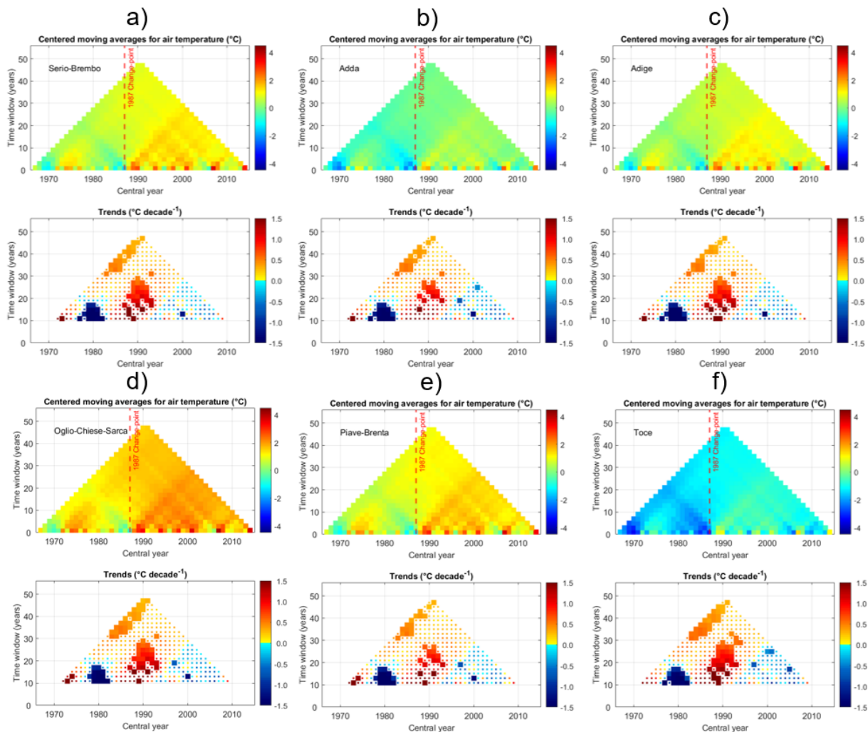
710 Figure 7: MARTA triangles of average winter (DJFM) temperature for the six macro-basins from the HISTALP dataset. In the top part of each panel the statistically significant change point detected by the Pettitt's test is reported as dashed line while in the bottom part the statistically significant trends with 5% significance level of the Mann – Kendall test are reported as thicker pixels.
