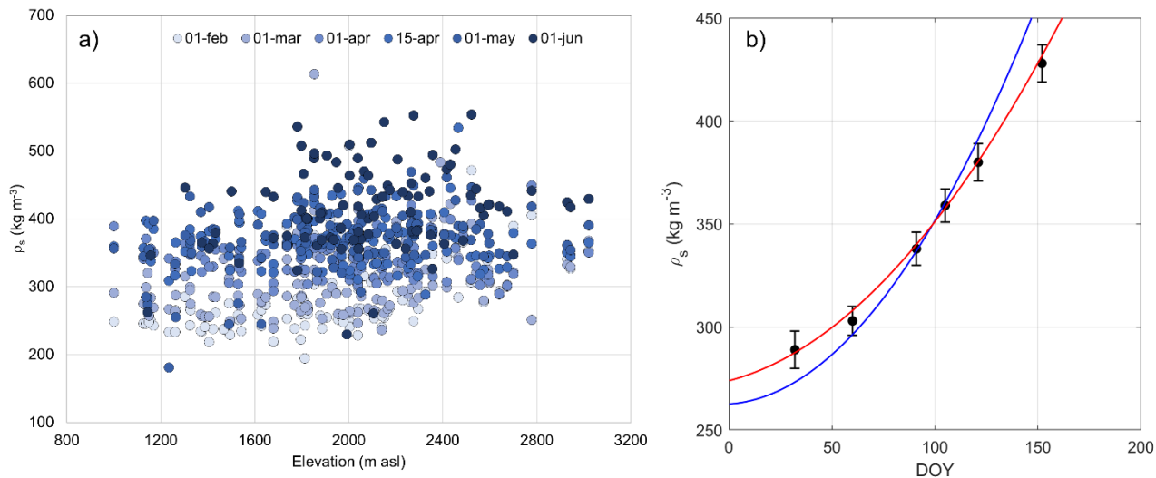
695 Figure 4: a) Bulk snow density dependence on elevation. Average bulk snow density for each measurement date is represented with different color intensity with changing date of the year. b) Temporal variability of bulk snow density. Average bulk snow density for each measurement date is represented as a black diamond and the error bars represent the standard deviation. We also report in red the computed polynomial model and in blue the one proposed in Guyennon et al. (2019).
