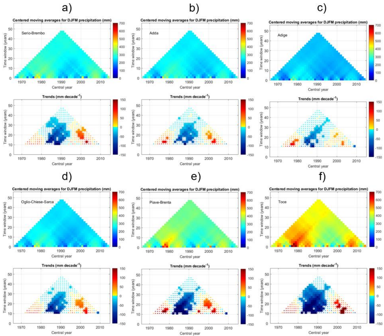
Figure 6: MARTA triangles of total winter (DJFM) precipitation for the six macro-basins from the HISTALP dataset. In the bottom part the statistically significant trends with 5% significance level of the Mann – Kendall test are reported as thicker pixels.
