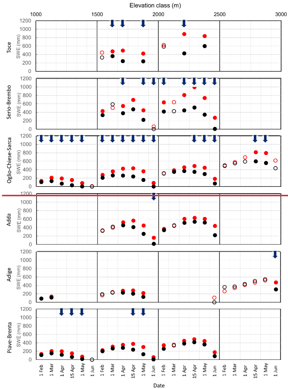
725 Figure 5: Average snow water equivalent (SWE) in the 1967-1993 (red circles) and in 1994-2020 (black circles) periods are plotted for each elevation class in the six observation campaigns dates (1 Feb, 1 Mar, 1 Apr, 15 Apr, 1 May, 1 Jun). Statistically significant ( p \leq 0.01 , Mann-Kendall test) trends of the entire 1967-2020 period are sketched as upward (downward) blue arrow for increasing (decreasing) trends. Circles are filled if the difference of SWE between the two periods is statistically significant ( p \leq 0.01 , Mann-Whitney test).
