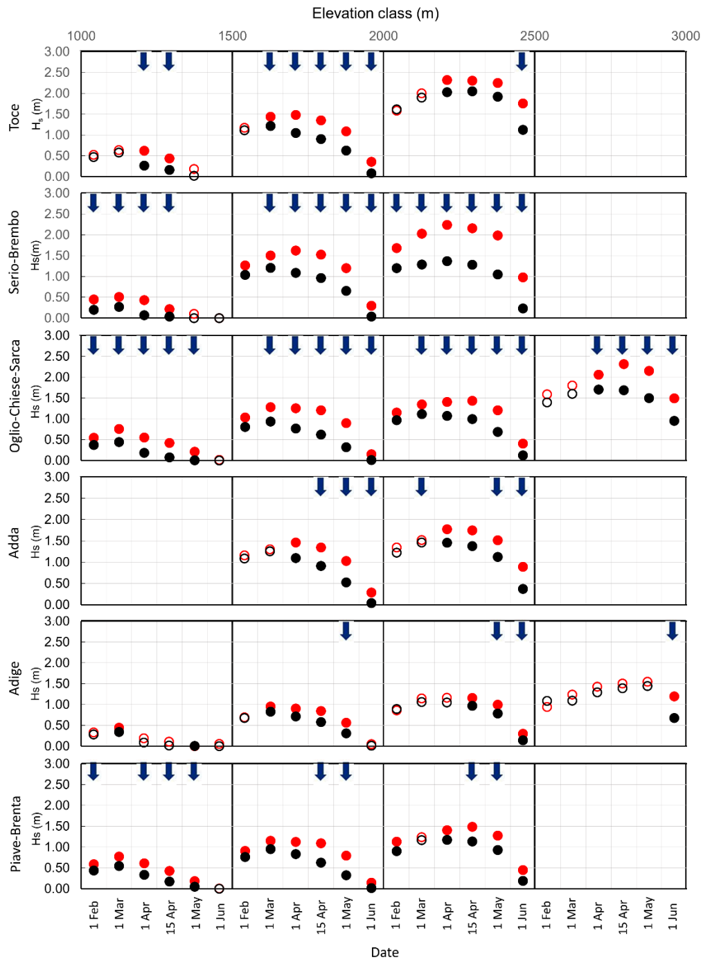
Figure 3: Average snow depth (Hs) in the 1967-1993 (red circles) and in 1994-2020 (black circles) periods are plotted for each elevation class in the six observation campaigns (1 Feb, 1 Mar, 1 Apr, 15 Apr, 1 May, 1 Jun). Statistically significant ( p \leq 0.01 , Mann-Kendall test) trends of the entire 1967-2020 period are sketched as upward (downward) blue arrow for increasing (decreasing) trends. Circles are filled if the difference of Hs between the two periods is statistically significant ( p \leq 0.01 , Mann-Whitney U test).
