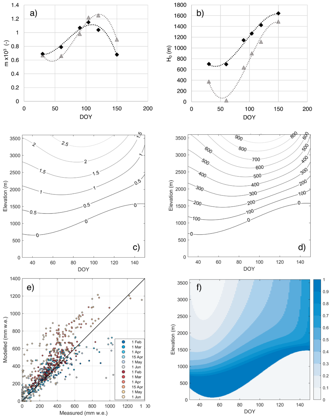
745 Figure 8: Slope m (a) and null snow depth elevation H_0 (b) as function of the day of the year for the sub periods 1967-1993 (grey triangles) and 1994-2020 (black diamonds). Dotted lines represent the third order polynomial fitting curve (Equation 4 and 5). Counter plots of snow depth (c) and snow water equivalent (d) in the time-elevation (DOY-H) space for the 1994-2020 sub period. In panel e) the scatter plot reporting measured and modelled climatological SWE in the Oglio-Chiese-Sarca macro basin for the first (red) and second (blue) sub periods. Panel f) reports the comparison between the modelled climatological SWE in the first and in the second sub periods, expressed as relative decrease of SWE (unitless). 750
