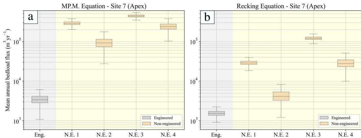
466 Figure 6. Boxplot representation of the mean annual bedload estimates using (a) the MP.M. and (b) the Recking 468 approaches for the Guerbe River catchment. The engineered (Eng.) and the non-engineered (N.E.) scenarios are based on using the parameters shown in Fig. 4. Specifically, the engineered scenario is based on the average of the engineered slopes, whereas the results for the non-engineered scenarios are based on: (N.E.1) a 75% 470 reduction of the channel width and grain sizes from site 7; (N.E. 2) a 75% reduction of the channel width and grain sizes from site 1; (N.E. 3) a 25% reduction of the channel width and grain sizes from site 7; and (N.E. 4) 472 25% reduction of the channel width and grain sizes from site 1.
