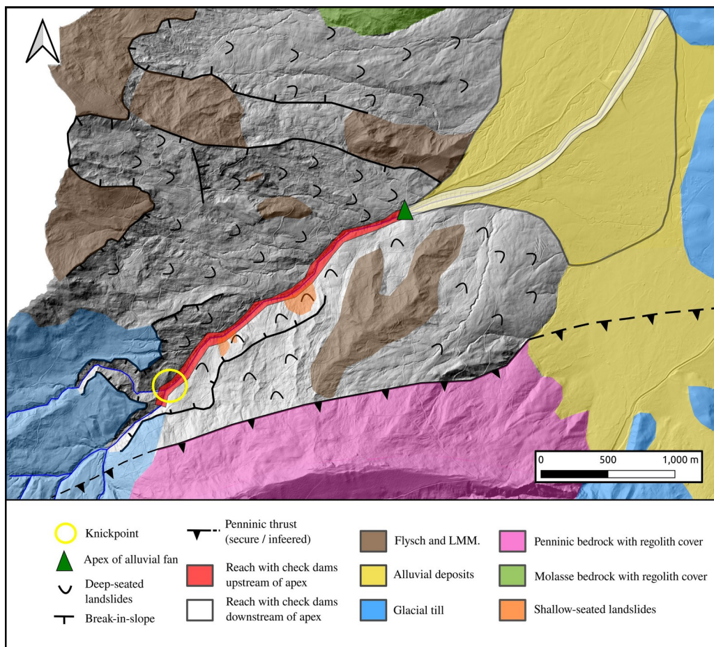
Figure 2. Map of the landslides and incised areas of the Guerbe River together with the bedrock geology underlying the catchment. The position of the knickpoint is marked located inside the yellow circle. See Fig. 1 for the position of this map. Here the LMM denotes the Lower Marine Molasse.
