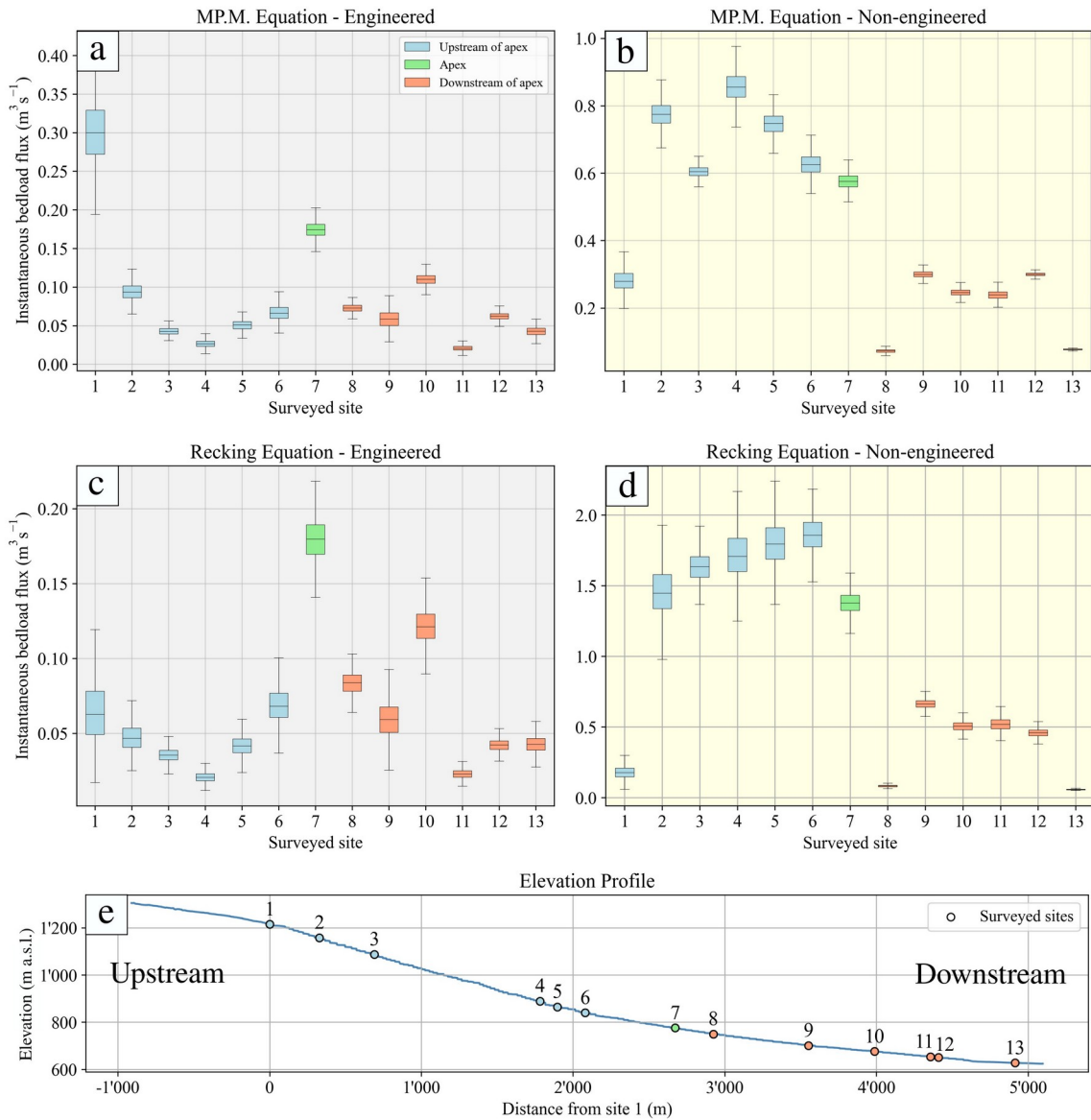
Figure 8. Boxplot representation of the bedload predictions using MP.M. and Recking during the 2021 peak runoff along all the surveyed sites. The engineered (a and c) and the non-engineered (b and d) scenarios are based on the parameters shown in Fig. 4. Specifically, in the non-engineered scenario we show the results where 50% of the current channel width is employed. The sites upstream and downstream of the alluvial fan apex are indicated by the blue and red colours, respectively, and the site on the apex is indicated by the green colour.
