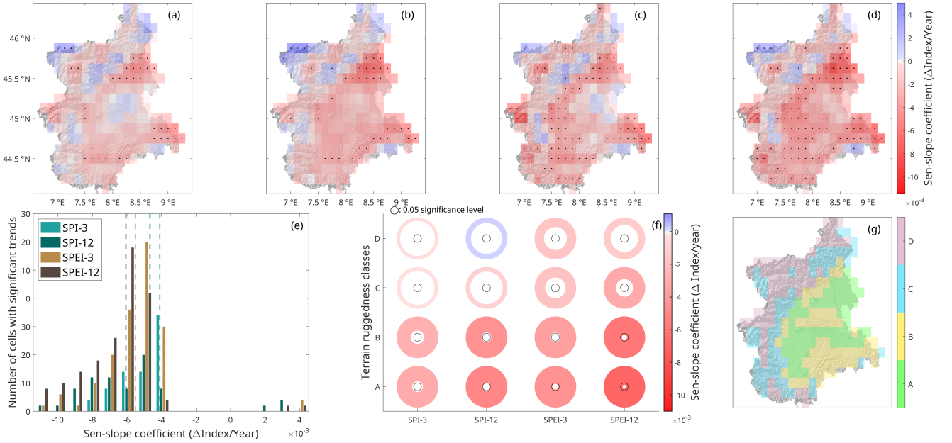
Figure 3. Trend analysis on drought indices. (a) SPI-3 trends. (b) SPEI-3 trends. (c) SPI-12 trends. (d) SPEI-12 trends. Cells containing a dot denote trends at 5% significance. (e) Frequency histogram of significant Sen-slope coefficients, with dashed lines representing the respective mean values of indexes' slope. (f) Trend analysis on drought indices calculated from data belonging to areas defined by terrain ruggedness inside cells. The colour of the circles represents the slope coefficient of the trend, while the inner radius of the circles represents the significance of the trend (a smaller inner radius represents a more significant trend). The black circles denote a significance level of 5%. (g) Representation of terrain ruggedness classes (see Figure A1 for more details on their definition).
