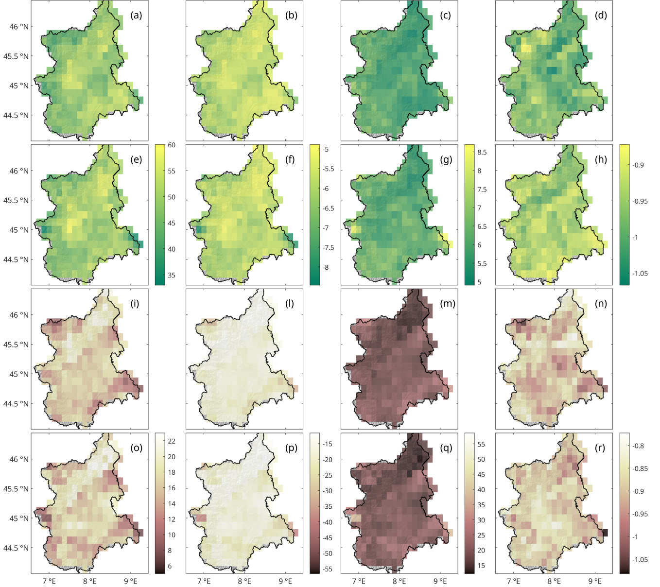
Figure 4. Spatial distribution of drought run characteristics at 3- and 12-month time scales. SPI-3's number of runs (a), average severity of local drought \overline{DS}_L (b), average length of local drought \overline{DD}_L (c), average intensity of local drought \overline{DI}_L (d). SPEI-3's number of runs (e), \overline{DS}_L (f), \overline{DD}_L (g), \overline{DI}_L (h). SPI-12's number of runs (i), average severity of local drought \overline{DS}_L (j), average length of local drought \overline{DD}_L (m), average intensity of local drought \overline{DI}_L (n). SPEI-12's number of runs (o), \overline{DS}_L (p), \overline{DD}_L (q), \overline{DI}_L (r).
