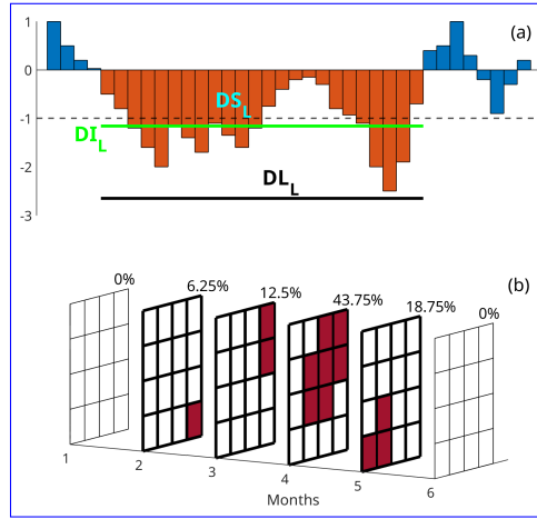
Figure 2. Drought runs examples, highlighted in orange. (a) Runs obtained with a simple -1 threshold (not Examples of the method used in this paper) for drought event definition. (b) Run (a) Local drought events defined by a threshold and by including their onset and offset, i.e. all negative values before and after the values under the threshold (as used in this paper). In both cases DS_L is the sum of the index value during the run, DD_L is the length of each run and DI_L is the mean index value during the run. (b) Region-wide drought events calculated for the entire study area, starting when at least 25% of cells have a drought index lower than -1 (represented as dark red in the figure) and including all preceding and following months with some cells with a lower than -1 index value. Months considered part of the drought event are highlighted by bolder grid lines in the figure.
