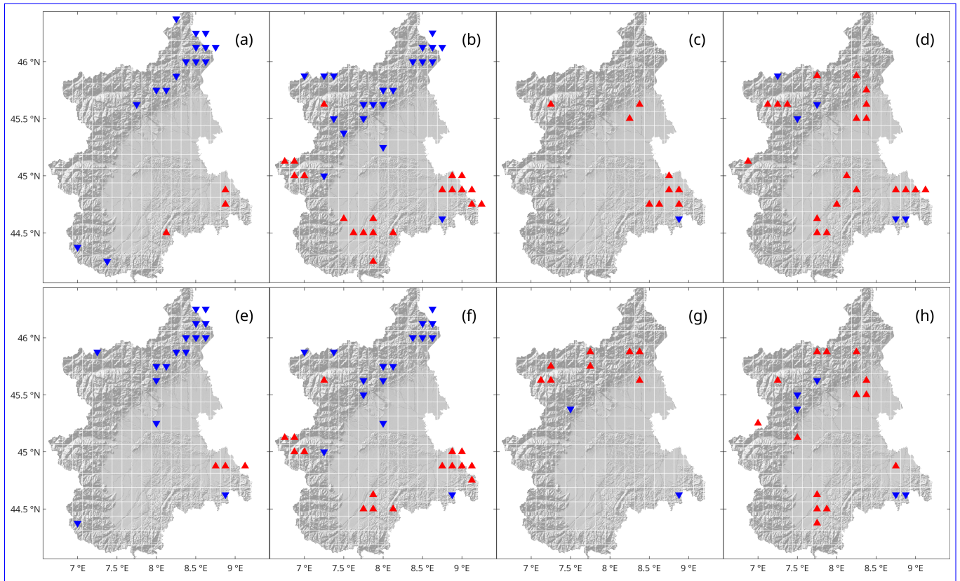
Figure 5. Cells with significant changes in-between the mean drought characteristics between-for the 1958-1990 and 1990-2023 periods according to the two sample t-test. (a) (a-d) Mean drought severity ( \overline{DS}_L ) increasechange for SPI-3 (a), SPEI-3 (b), SPI-12 (c), SPEI-12 (d). (e-h) Mean drought duration ( \overline{DD}_L ) increasechange for SPI-3 (e), (e) Mean drought severity ( \overline{DS}_L )-decreaseSPEI-3 (f), (d) Mean-SPI-12 (g), SPEI-12 (h). Red/blue arrows indicate a worsening/bettering of drought duration-conditions ( \overline{DD}_L i.e. higher/lower severity and longer/shorter duration) decrease .
