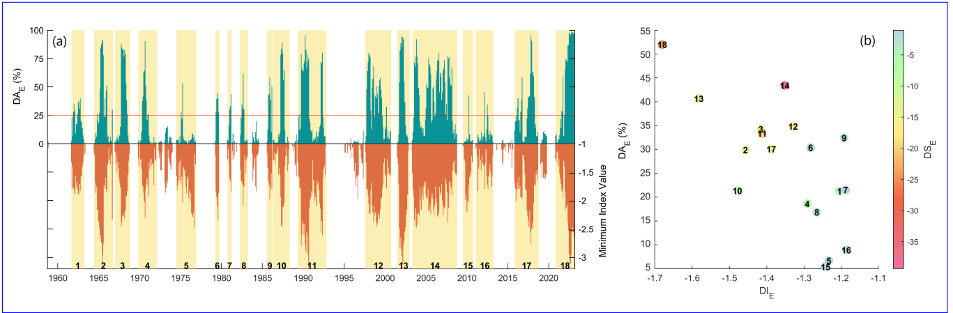
Figure 6. Region-wide drought event analysis conducted on SPEI-12. (a) Time series of percentage of cells in drought condition (only the portion below the -1 threshold, upper part of the diagram) and minimum index value in the domain (lower part of the diagram). Each event is highlighted in yellow and labeled. (b) Drought event characteristics: drought intensity ( DI_E ), mean drought area ( DA_E ) and drought severity ( DS_E ).
