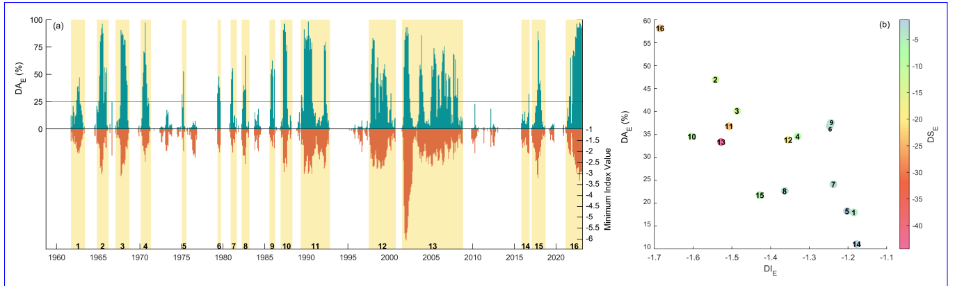
Figure A3. Region-wide drought event analysis conducted on SPI-12. (a) Series of percentage of cells in drought condition (below the -1 threshold) and the minimum index value in the domain. Each event is highlighted in yellow and labeled. (b) Drought event characteristics.
