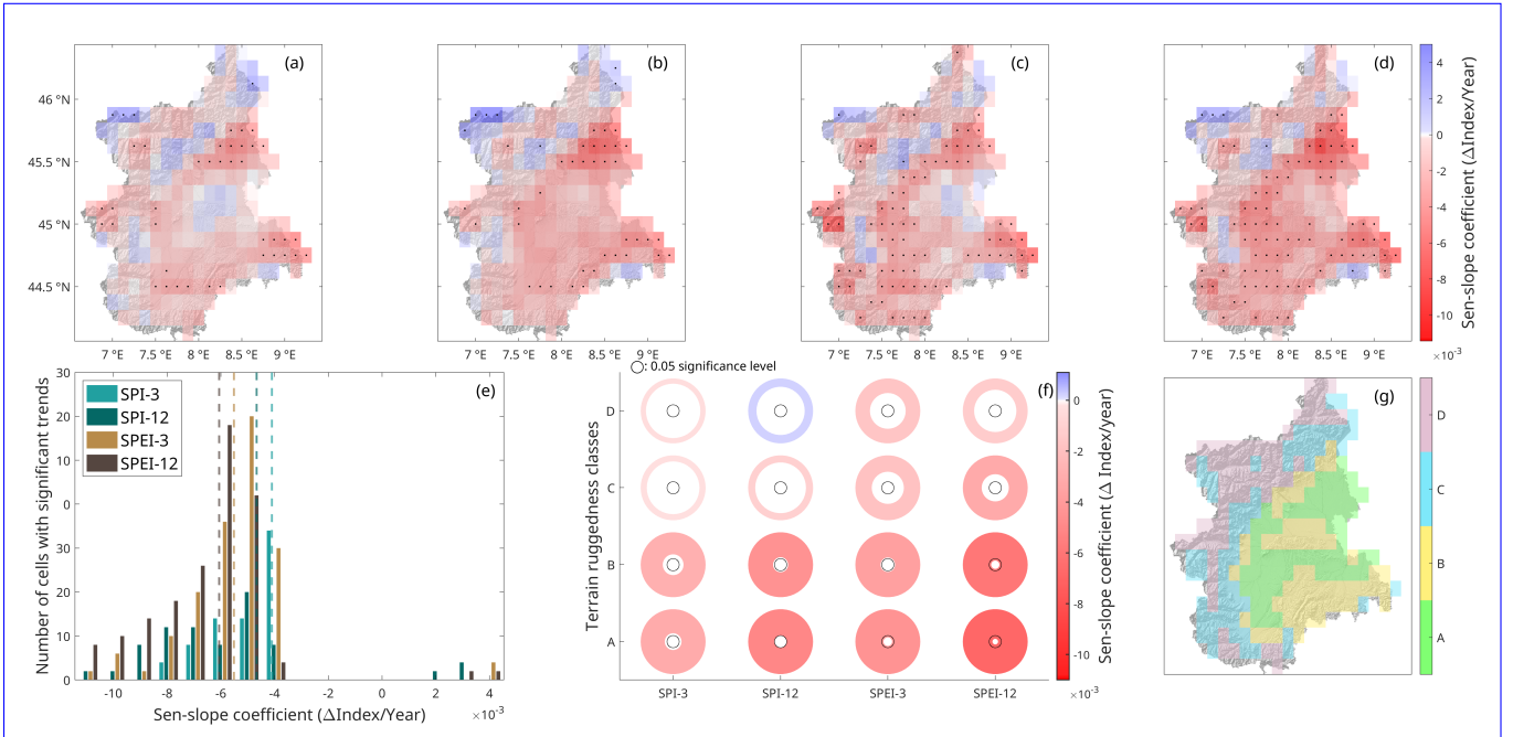
Figure 3. Trend analysis on drought indices. (a) SPI-3 trends. (b) SPEI-3 trends. (c) SPI-12 trends. (d) SPEI-12 trends. Cells containing a dot denote significant trends at 5% significance. (e) Frequency histogram of significant trends-per-distribution-of-trends' Sen-slope coefficients, with dashed lines representing the respective mean values of indexes' slope . (f) Trend analysis on drought indices calculated from data belonging to areas defined by terrain ruggedness inside cells. The colour of the circles represents the slope coefficient of the trend, while the inner radius of the circles represents the significance of the trend (a smaller inner radius represents a more significant trend). The black circles denote a significance level of 5%. (g) Representation of terrain ruggedness classes (see Figure 2-A1 for more details on their definition).
