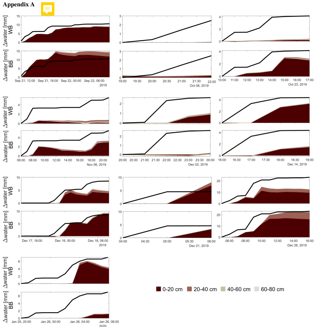
Figure A1. Panels show cumulative precipitation (line) and cumulative soil water storage change of each sensor for all precipitation events not shown in figure 2, for both the windbreak (upper row) and the blackberry (lower row) location. The different colours represent the different depths of the sensors.
