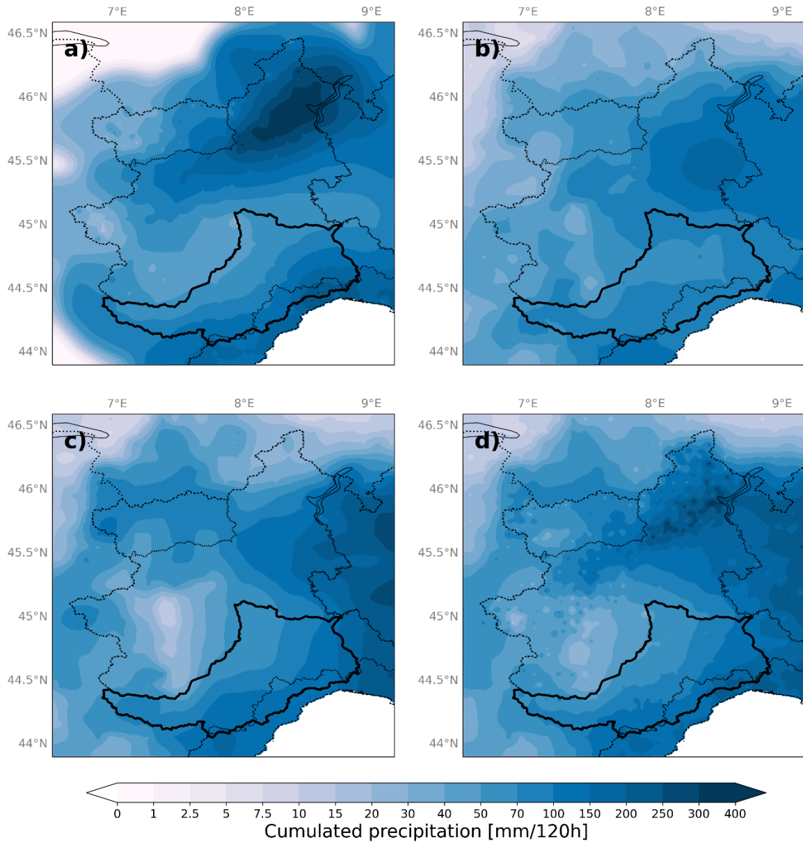
Figure 56: CS 01 Areal Precipitation Estimation: the figures show the rain field rebuilt using rain gauge data (a), GPM IMERG FINAL CAL (b), GPM IMERG FINAL UNCAL (c). Panel d shows the rain field obtained forcing the hydrological model with rain gauge data, using a radius of influence equal to 5km, merged with GPM IMERG FINAL UNCAL.
