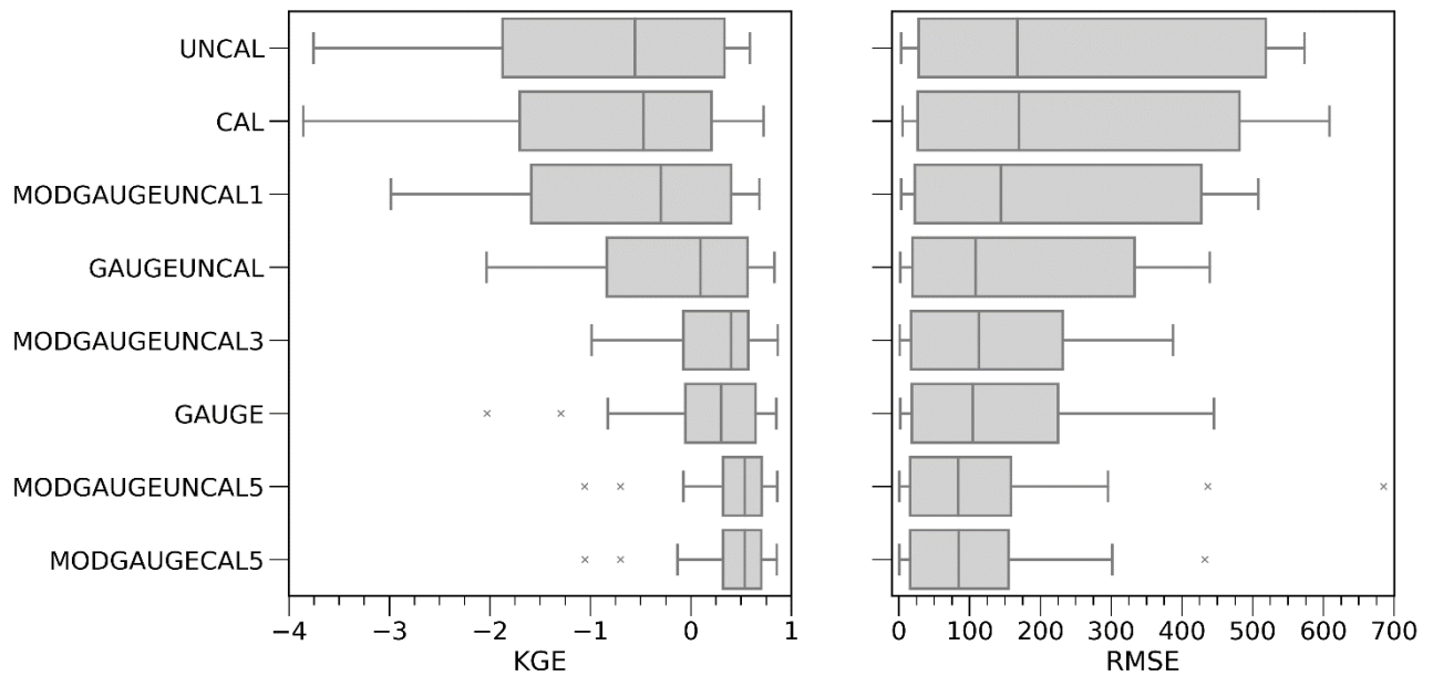
Figure 78. The boxplots show the summary refer to KGE and RMSE obtained from the CHYM simulation using the eight APE fields as input, related to all three Case Studies and all river sections. The rain gauge data (GAUGE simulation) allows for better performance than using the satellite data alone (UNCAL and CAL), but the results are better if the two data sources are merged, especially using the MODGAUGEAL5 setting, which is comparable to MODGAUGEUNCAL5. The same results are obtained both in terms of quality score (KGE) and error estimation (RSME).
