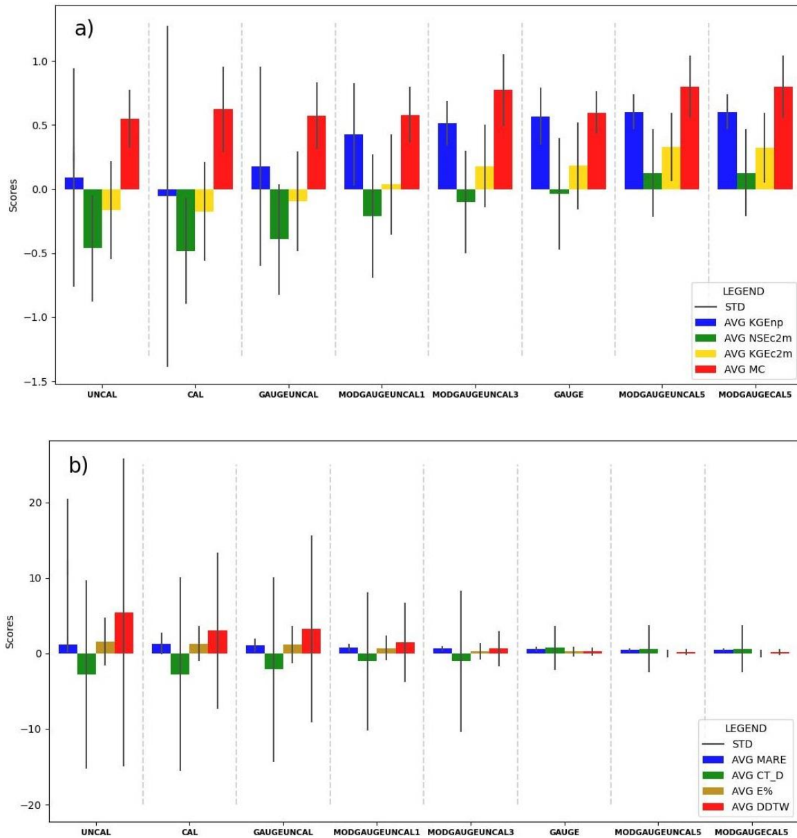
Figure 89. The histograms summarize the statistical analysis performed for the different scores, evaluating their average (AVG) and the standard deviation (STD). The figure a) shows the quality scores (KGE np , NSE c2m , KGE c2m and MC) where the best performances are identified by a value equal to 1. In the figure b) (MARE, CT D , E% and DDTW) the best performances are identified by values close to zero.
