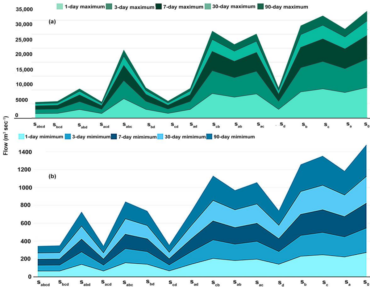
470 Figure 7. The magnitude of annual extreme flow conditions (upper panel: maxima, lower panel: minima) of flow regimes generated by different configurations of reservoirs
