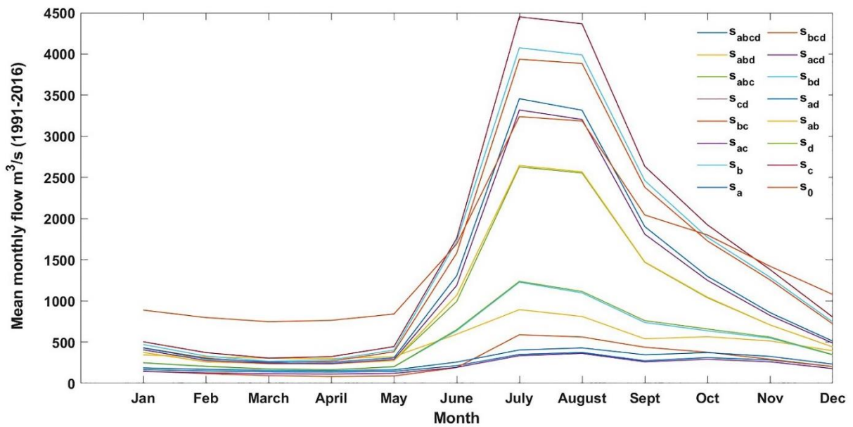
445 Figure 6. The mean monthly flows resulting from different configurations of reservoirs
