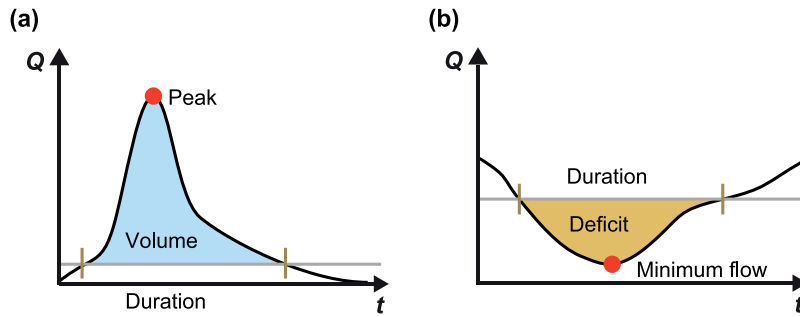
Figure 4. Illustration of flood and drought characteristics: (a) floods: peak discharge, volume, and duration; (b) droughts: minimum flow, deficit, and duration.
