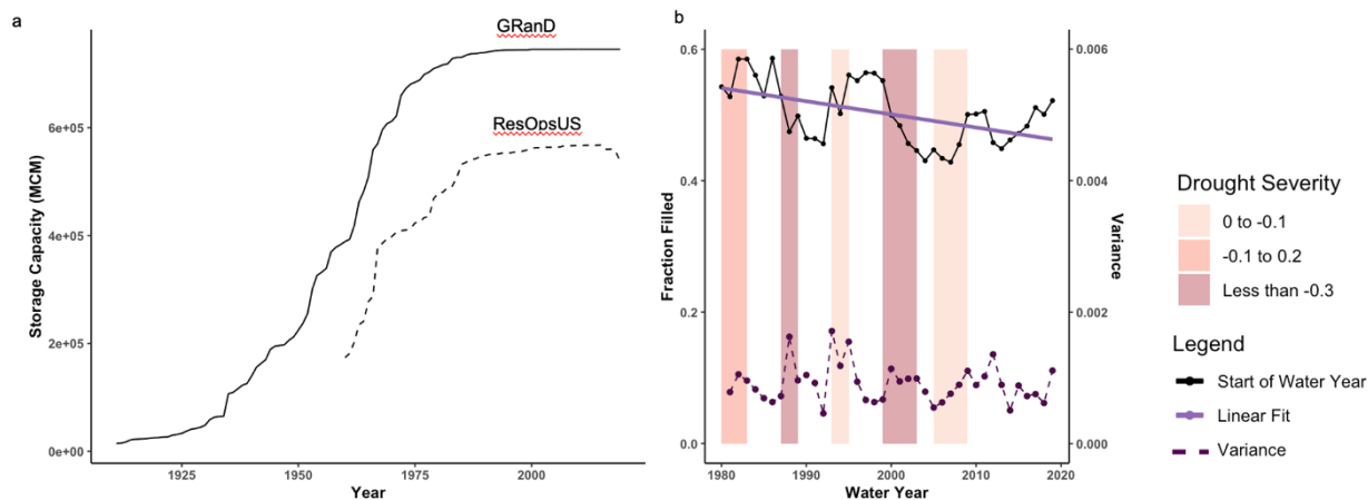
355 Figure 5: Total storage capacity reported by GRanD (solid line) and the storage capacity of 679 large dams in ResOpsUS (dashed). (b) The reservoir fraction filled value on October 1st from the ResOpsUS data from the forty-year period from 1980 – 2019 (interannual fraction filled). The lavender line is the linear fit through this entire period of record with a slope of -0.002 fraction filled per year and a p value of 0.01. The colored rectangles depict the drought periods with darker colors referring to more severe droughts (SPI values less than -0.3), medium dark (SPI values between -0.1 and -0.3) and lighter bars for least severe droughts (values between 0 and -0.1).
