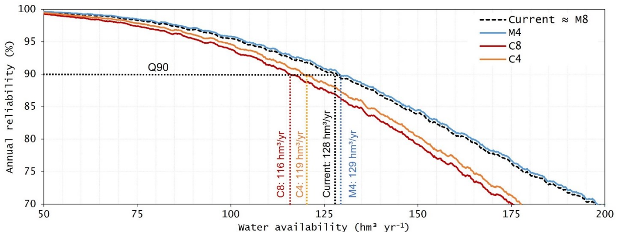
335 Figure 8: Water availability as a function of annual reliability level for the Gavião, Riachão and Pacoti reservoirs. Each curve represents a different evaporation rate: current (1961-2005) historical average and four climate change scenarios (M4, M8, C4, and C8) at the end of the 21st Century.
