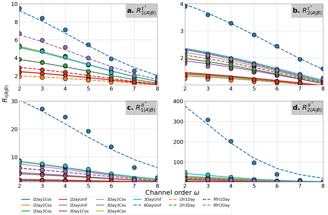
400 Figure 4. Convergence for all the signals relative to the Dirac assuming constant velocity routing. The dots correspond to the median value of the moments ratio R , and the lines correspond to equation (7) results.
