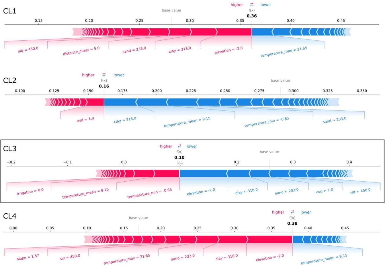
680 Figure E7 SHAP force plots explaining the prediction of the CL3 exemplary well site from the case study region in northern Germany (Fig. 5a) that is confused with CL4. At this well site, the probability that CL4 is predicted is the largest in the case study (test dataset). The average scores of all classifications made by the Random Forest model for the training dataset are 0.28, 0.29, 0.26, and 0.17 respectively (base values). The model's probability scores for predicting the clusters at the exemplary well site (bold printed numbers) sum up to 100 %. Features that are important for the respective predictions are displayed with their values. Their importance and effects can be assessed by the SHAP values visualized by bar length and color (i.e. the larger the feature's share of 685 the bar the more important; red represents rejecting effect and blue represents supporting effect).
