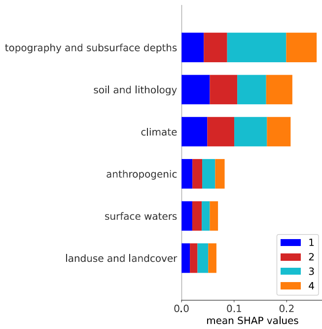
645 Figure E2 Overall SHAP feature importance stacked for individual clusters for aggregated features (SHAP values added up for features from the same attribute categories from Table 1).
