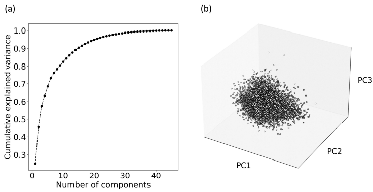
610 Figure C1 Principal component analysis with the indices dataset. (a) Cumulative explained variance with an increasing number of Principal Components (PCs). (b) Dataset value space of the first three PCs (which together explain more than 50 % of the variance of the dataset).
