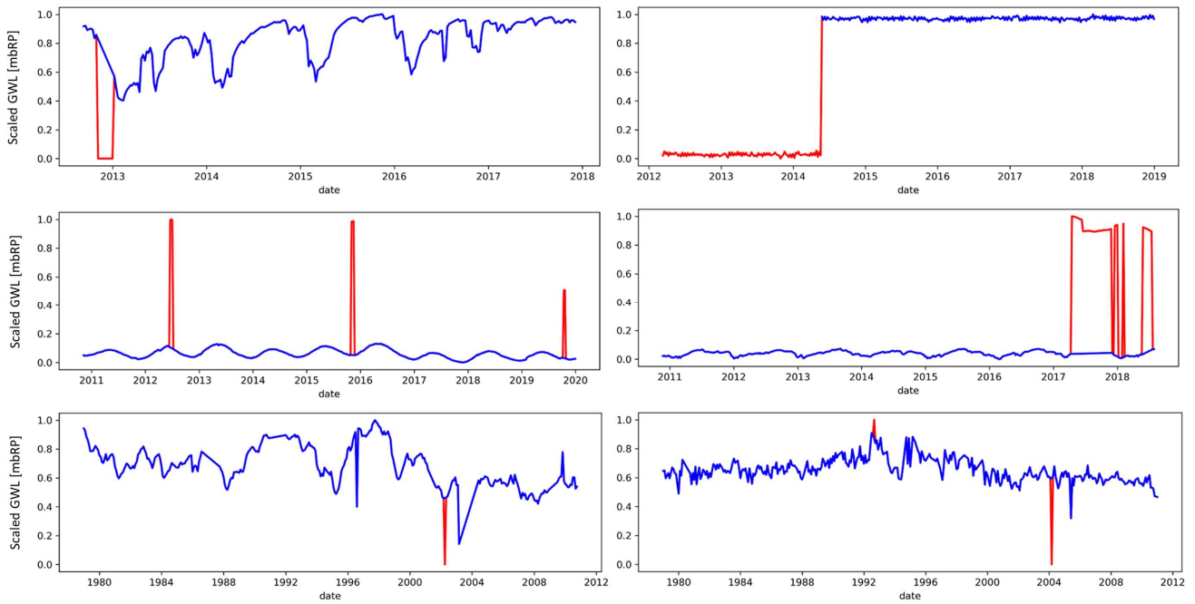
590 Figure A1 Examples of time series outlier removal with DBSCAN (scikit-learn library in Python): Raw (scaled) time series are shown in blue, and the anomalies identified by DBSCAN (Ester et al., 1996) are shown in red. The use of DBSCAN is less successful or difficult to verify in the bottom two examples (left: The first abrupt change in direction of the GWL between 1996 and 2000 is not identified as an outlier, although one would expect one based on the magnitude and position of the change; right: From visual inspection, it is unclear whether the identified outliers in both directions are due to measurement error, human activity or reflect natural behavior of the groundwater system e.g. to extreme events). In summary, like other tested outlier detection methods, DBSCAN does not allow us to detect all types of outliers and anomalies that we would expect should be removed to represent undisturbed GWL dynamics. With the parameters set, we can successfully detect most density-dependent outliers, but many values were incorrectly identified as outliers. Therefore, we performed a visual inspection of all time series where DBSCAN identified potential outliers. 595
