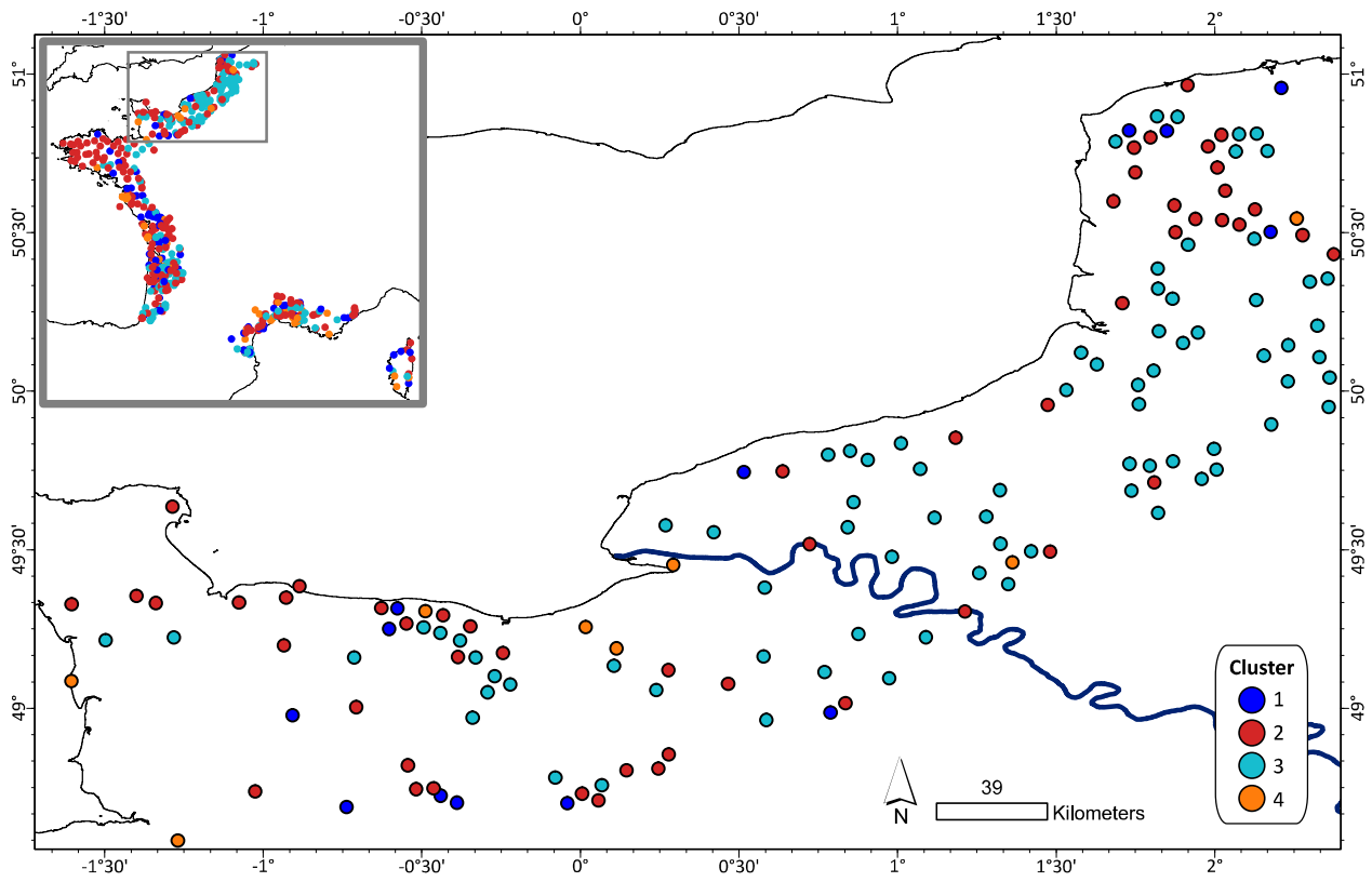
635 Figure C6 Assignment of clusters to well locations in the Normandy, Paris Basin displayed with the Seine River. Overlapping well markers were jittered at a minimum spacing of 1000 meters and thus no longer represent the original well locations. The window in the upper left corner shows the Normandy region in the north of France.
