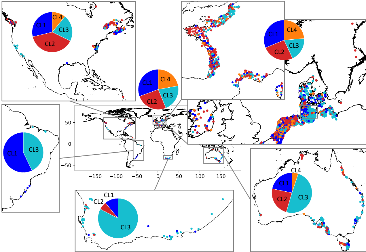
270 Figure 1 Assignment of clusters to well locations globally (center) and in coastal regions in North America, Europe (enlarged map of France and northwestern Europe), Australia, South Africa, and Brazil. Due to the large scale, overlapping dots are not jittered, but well points are shuffled to prevent the same clusters from being constantly drawn over others.
