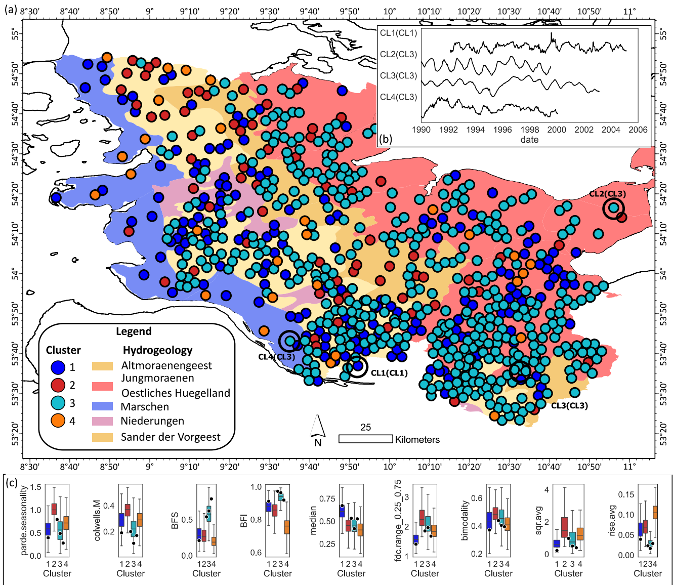
385 Figure 5 GWL dynamics patterns in the German federal state Schleswig-Holstein. (a) Cluster assignment to well locations and hydrogeology map of the German federal state Schleswig-Holstein (LfU-SH, 2003). Overlapping well markers are jittered at a minimum spacing of 500 meters and thus no longer represent the original well locations. The cluster number in parentheses marks the true cluster from k-means clustering. (b) Exemplary time series of each cluster from the encircled well sites in (a). (c) Within-cluster variability of the example indices that each represent a component of the Heudorfer et al. 2019 typology from Fig. 3 plotted
