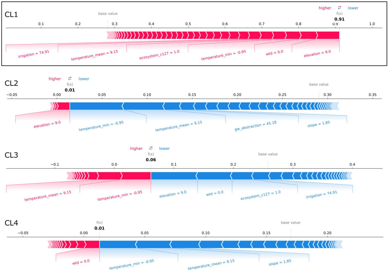
655 Figure E4 SHAP force plots explaining the correct prediction of the CL1 exemplary well site from the case study region in northern Germany (Fig. 5a). At this well site, the probability that CL1 is predicted is the largest in the case study (test dataset). The average scores of all classifications made by the Random Forest model for the training dataset are 0.28, 0.29, 0.26, and 0.17 respectively (base values). The model's probability scores for predicting the clusters at the exemplary well site (bold printed numbers) sum up to 100 660 %. Features that are important for the respective predictions are displayed with their values. Their importance and effect can be assessed by the SHAP values visualized by bar length and color (i.e. the larger the feature's share of the bar the more important; red represents rejecting effect and blue represents supporting effect).
