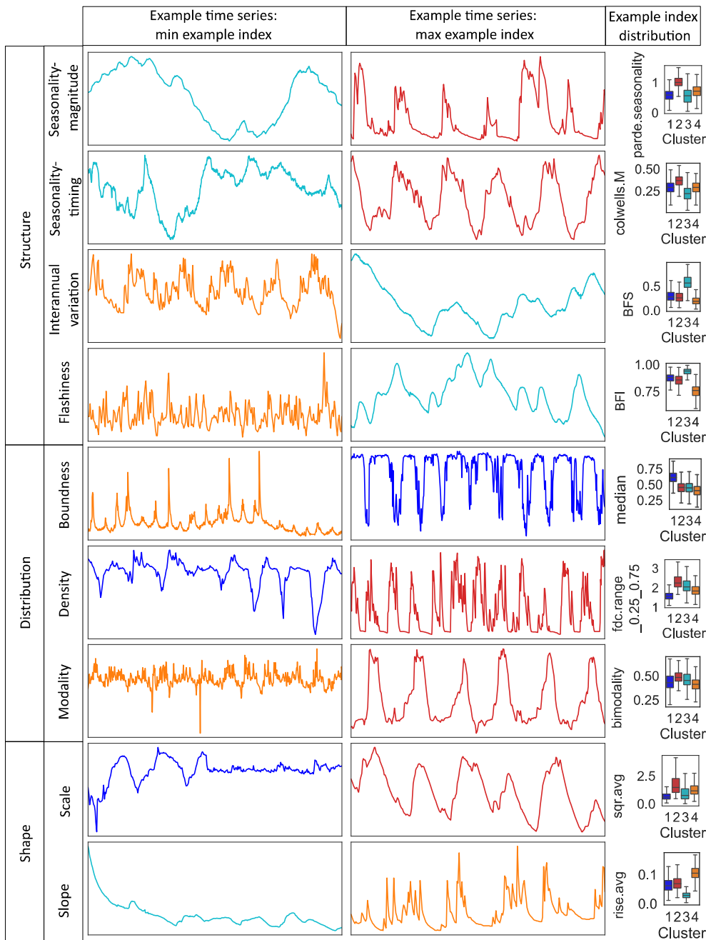
295 Figure 3 Example groundwater time series from the European continent illustrate typical scaled GWL time series where one aspect from each component of the Heudorfer et al. (2019) typology of GWL dynamics (Table B1) is weak (left column) and strong (right column), with an example index from that component that is displayed showing within-cluster variability (see Fig. C4 for within-cluster variability for all indices).
