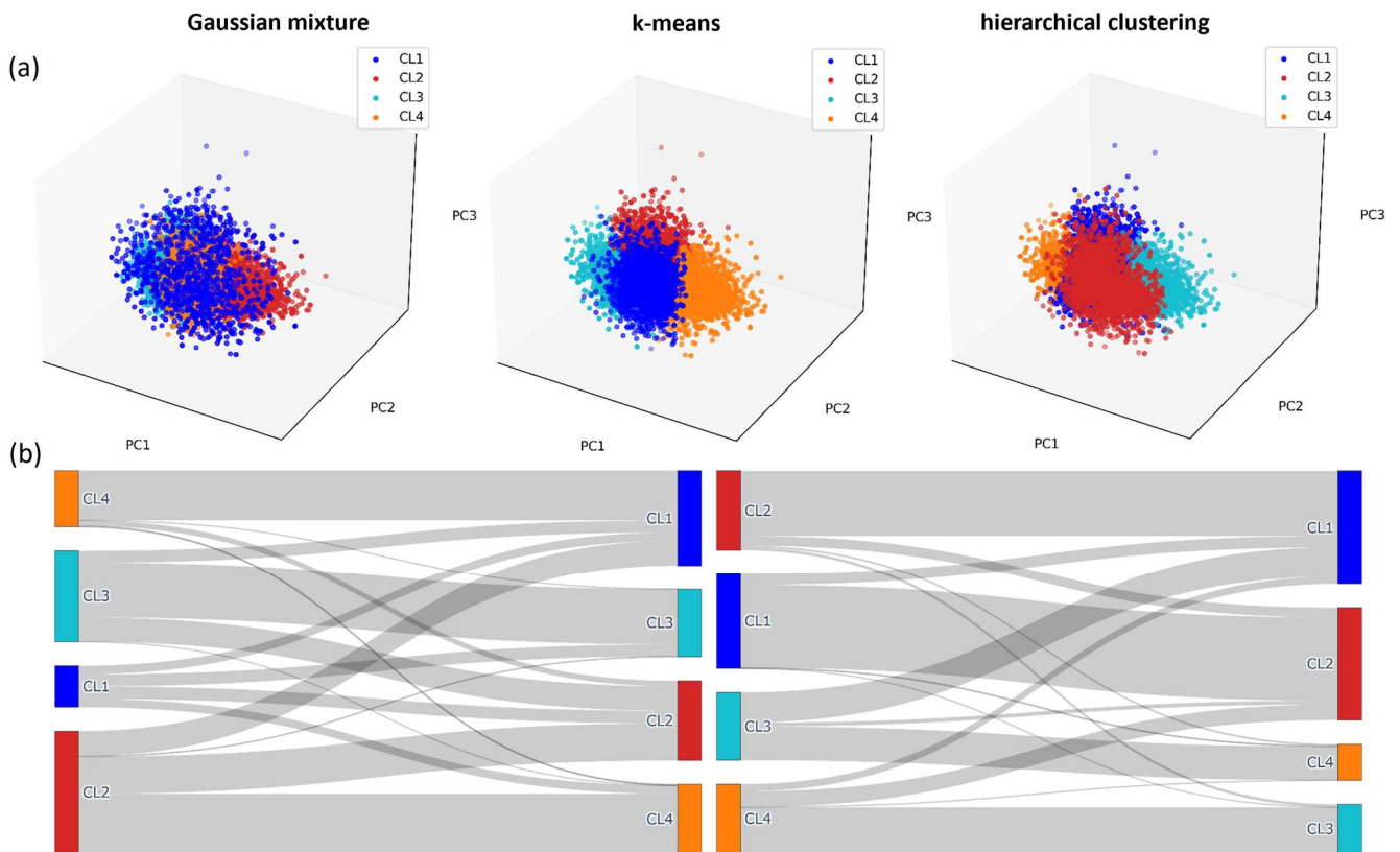
Figure C3 Assignment of the time series to four different clusters by three algorithms (Gaussian mixture, k-means, and hierarchical clustering). (a) Illustrative cluster assignment within the range of values of the first three principal components (PCs) of the dataset. (b) Sankey plot allows comparison of the quantitative distribution of the samples among the clusters (left between Gaussian mixture and k-means and right between k-means and hierarchical clustering).
