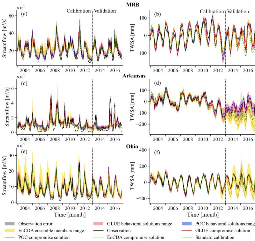
Figure 4. Monthly time series of simulated and observed Q (a, c, e) and TWSA (b, d, f) during calibration period 2003-2012 and validation period 2013-2016 for MRB (a, b), Arkansas River basin (c, d) and Ohio River basin (e, f). Observations and their assumed errors are shown together with simulated GLUE, POC, and EnCDA compromise solutions, with the range of GLUE and POC behavioral solutions (maximum and minimum monthly values of the behavioral solutions, Table 36) and the range of all 32 EnCDA ensemble members, as well as with the WaterGAP variant with standard calibration.
