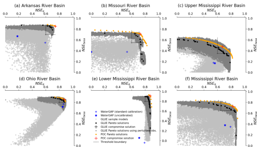
660 Figure 3. Performance of 1) Pareto-optimal solutions derived by an evolutionary optimization algorithm (POC) (orange dots), 2) the GLUE ensemble (light grey pluses), and 3) the Pareto-optimal subset of the GLUE ensemble (black dots), in all cases neglecting observation error when computing NSE. In addition, the performance of 4) the Pareto-optimal GLUE parameter subset for 1,000 realizations of perturbed observations are shown (dark grey dots), which shows the impact of observation errors on NSE. Compromise solutions of both POC and GLUE approaches are shown, too, together with the model performance after standard calibration and without calibration, consistent with Table 2. The thresholds for behavioral parameter sets (Table 3) are indicated by the grey dashed lines.
