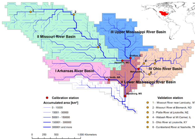
Figure 2. The Mississippi River basin as represented by the 0.5^\circ \times 0.5^\circ grid cells in WaterGAP, with delineation of the five CDA units. The CDA units were defined as the upstream cells of the five indicated calibration stations (streamflow gauging stations, shown in red). The stream network implemented in WaterGAP is shown, indicating the upstream areas of each grid cell by the line width. In addition, the locations of the six streamflow validation stations are plotted, shown in orange. 375
