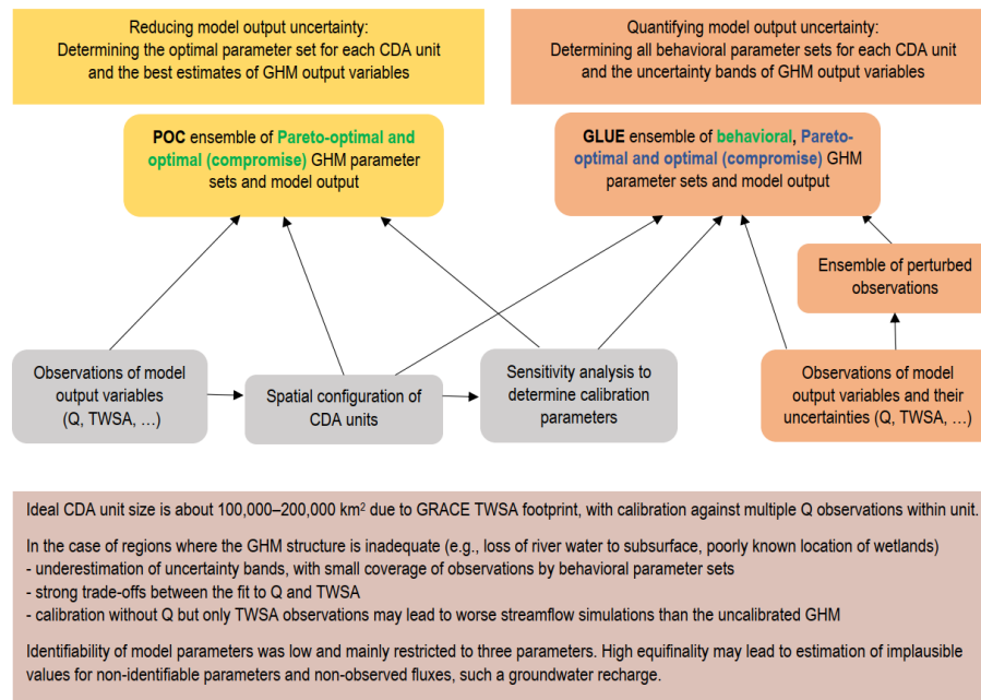
1325 Figure 7. The proposed approach for reducing and quantifying model output uncertainty of GHM by multi-variable parameter estimation and main recommendations and caveats for applying the approach in global hydrological modeling. Green letters indicate for which purpose POC and GLUE are best suited, while blue letters indicate an acceptable capability. A CDA unit is composed of all GHM grid cells to which the same calibration parameter value is assigned.
