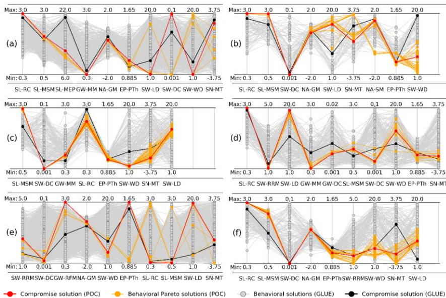
900 Figure 5. Parameter sets determined by POC and GLUE calibration approaches as depicted by parallel coordinate plots for CDA units (a) Arkansas, (b) Missouri, (c) Upper MRB, (d) Ohio, (e) Lower MRB, and (f) MRB. The parameter abbreviations are given at the bottom of each plot, where the order was selected to show interesting relations between parameter values. The numbers at the top and bottom of the plots indicate the a-priori range of the calibration parameters listed in Table 1. The number of behavioral solutions is given in Table 3. GLUE behavioral solutions are shown in greys, GLUE compromise solution in black, POC Pareto behavioral solutions in oranges and POC compromise solution in red.
