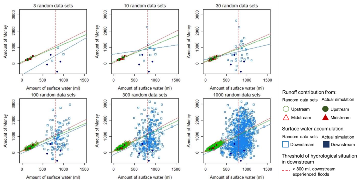
695 Figure E4. Runoff and economic conditions based on random value simulation and actual simulation
