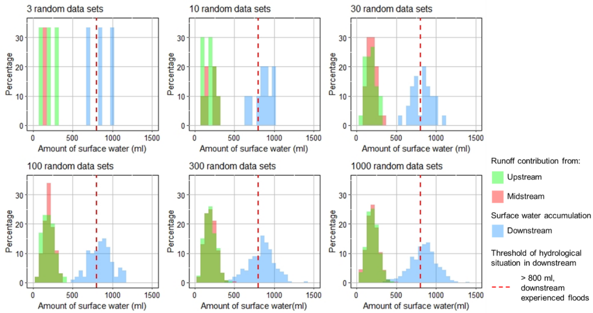
690 Figure E2. Distribution of runoff contribution from upstream and midstream and surface water accumulation in downstream based on simulation with the random value
