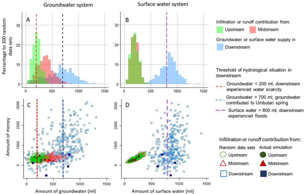
360 Figure 4: Simulation of hydrological and economic situation in H 2 Ours game using random value (N = 300) and game actual simulation (obs.) results (N = 4) for the Rejoso watershed. A. Distribution of infiltration contribution from upstream and midstream and groundwater supply in downstream based on simulation with the random value; B. Distribution of runoff contribution from upstream and midstream and surface water accumulation downstream based on simulation with the random value; C. Groundwater situation and economic situation based on random value simulation and actual simulation; D. Runoff situation and economic situation based on random value simulation and actual simulation. Appendix E provides a further analysis of the solution space 365
