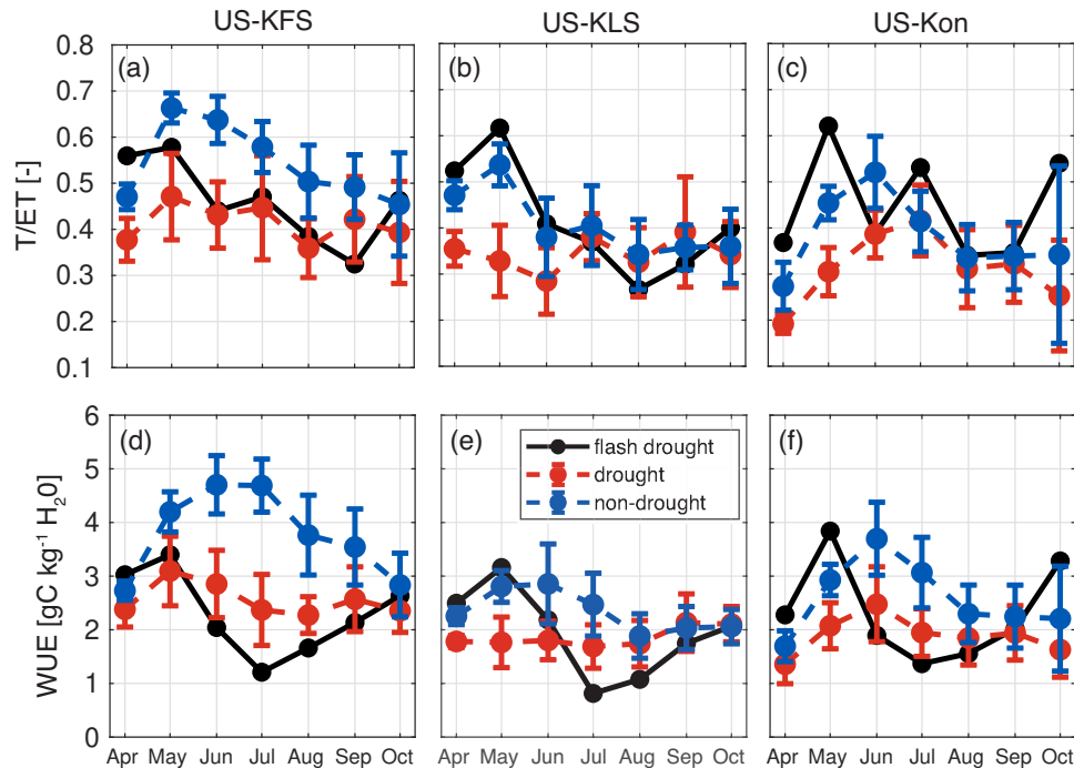
Figure 15. Ratio of transpiration to evapotranspiration, T/ET [-], and water-use efficiency, WUE [ g\ C\ kg^{-1}\ H_2O ], for for drought (red) and non-drought (blue) years compared to flash drought (black) for US-KFS (left), US-KLS (middle), and US-Kon (right).
