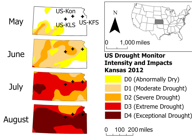
Figure 2. Evolution of the 2012 flash drought from May - Aug -August in the US Drought Monitor with the three AmeriFlux tower study sites (US-KFS, US-KLS, and US-Kon).
