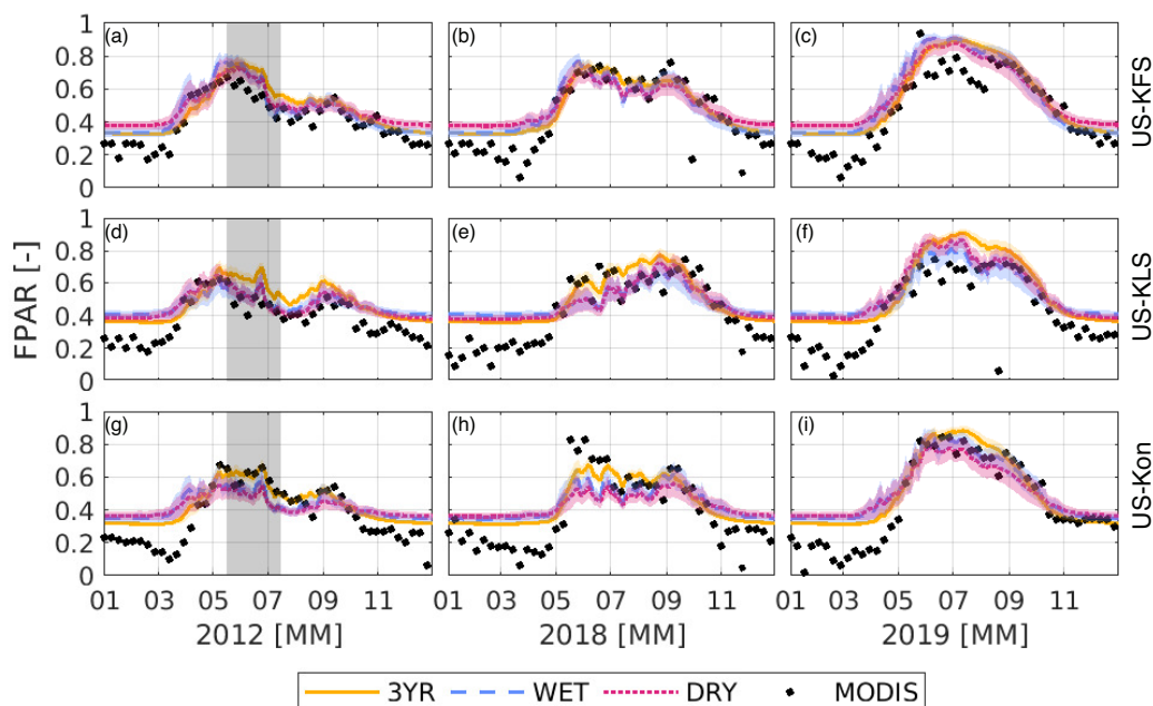
Figure 5. Fraction of photosynthetically active radiation ( f_p , FPAR) [-], predicted from the DCHM-PV for the flash drought year (2012), a drought year (2018), and a non-drought year (2019) for US-KFS (top row), US-KLS (middle row), and US-Kon (bottom row). Colors indicate the different data assimilation periods: 3YR (yellow), WET (blue), DRY (red). Corresponding shaded regions represent one standard deviation of model outputs from the 2000 ensemble members. The 8-day MODIS MOD15A2H LAI FPAR is shown as black dots. The gray shaded regions in the left most panels highlights the 2012 flash drought period.
