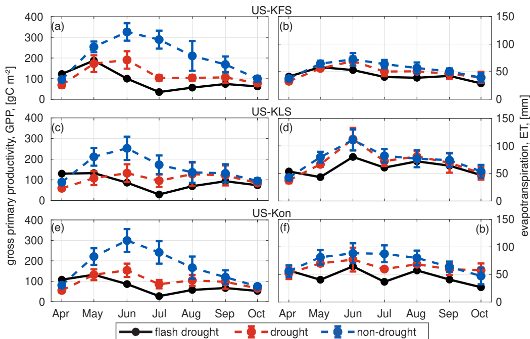
Figure 10. DCHM-PV 3YR monthly totals of GPP [ \text{gC m}^{-2} ] (a,e,efleft) and ET [mm] (b,d,fright) for drought (red) and non-drought (blue) years compared to flash drought (black) for US-KFS (top row), US-KLS (middle row), and US-Kon AmeriFlux-sites (bottom row). Monthly totals are computed from the ensemble means of the 2000 Monte Carlo simulations then averaged across drought or non-drought years. Error bars represent one standard deviation across drought and non-drought years, respectively.
