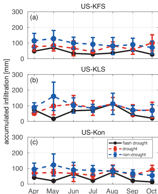
Figure 7. DCHM-PV 3YR ensemble means of monthly infiltration accumulations [mm] for drought (red dashed line) and non-drought (blue dashed line) years compared to 2012 (black solid line) for all three study sites US-KFS (top), US-KLS (middle), and US-Kon (bottom) . Monthly sums are computed from the ensemble means of the 2000 Monte Carlo simulations then averaged across drought or non-drought years. Error bars represent one standard deviation across drought and non-drought years.
