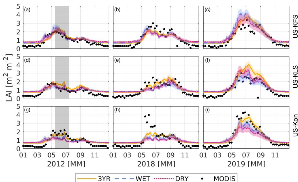
Figure 6. Leaf area index ( LAI ) [ m^2 m^{-2} ], predicted from the DCHM-PV for the flash drought year (2012), a drought year (2018), and a non-drought year (2019) for US-KFS (top row), US-KLS (middle row), and US-Kon (bottom row). Colors indicate the different data assimilation periods (yellow—3YR (2003-2005), blue—WET (2005), red—DRY (2003)), with corresponding shaded regions representing represent one standard deviation of model outputs from the 2000 ensemble simulations members. The 8-day MODIS MOD15A2H LAI is shown in as black markers dots. The gray shaded regions in the left most panels highlights the 2012 flash drought period.
