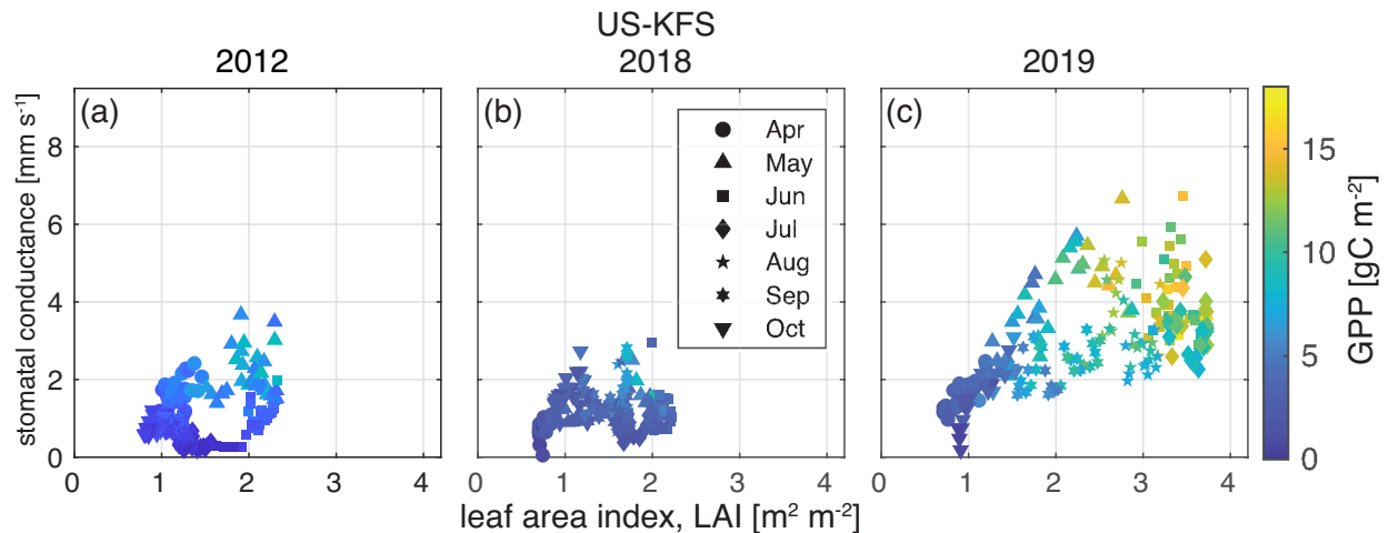
Figure 12. Stomatal conductance [ \text{mm s}^{-1} ] vs leaf area index, LAI [ \text{m}^2 \text{m}^{-2} ], for US-KFS for a flash drought year (2012), a drought year (2018), and a non-drought year (2019). Marker shapes indicate individual days between April 1 - October 31. Each month is given a unique shape whose color reflects daily accumulations of gross primary productivity, GPP [ \text{gC m}^{-2} ].
