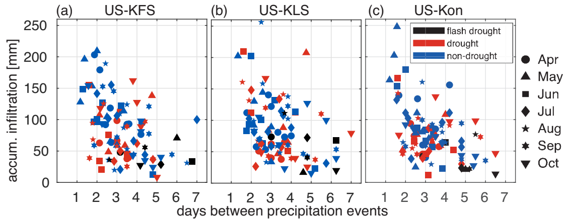
Figure 8. Monthly infiltration accumulation [mm] vs average days between precipitation events within a single month for (a) US-KFS, (b) US-KLS, and (c) US-KON. Each shape indicates the month over which the averaging occurred and colors distinguish flash drought (black) from drought (red) and non-drought (blue) years.
