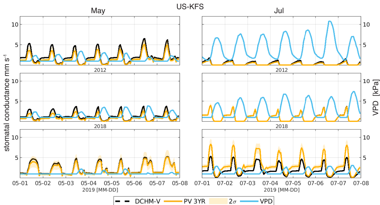
Figure 9. Stomatal conductance [ \text{mm s}^{-1} ] and vapor pressure deficit (VPD [ \text{kPa} ]) for one week in May (left) and July (right) of 2012, 2018, and 2019 for US-KFS.
