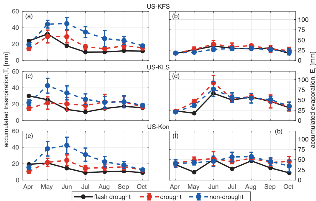
Figure 13. DCHM-PV 3YR monthly totals of transpiration T , [mm] (a,e, left) and evaporation E , [mm] (b,d, right) for drought (red) and non-drought (blue) years compared to flash drought (black) for US-KFS (top row), US-KLS (middle row), and US-Kon AmeriFlux sites (bottom row). Monthly totals are computed from the ensemble means of the 2000 Monte Carlo simulations then averaged across drought or non-drought years. Error bars represent one standard deviation across drought and non-drought years, respectively.
