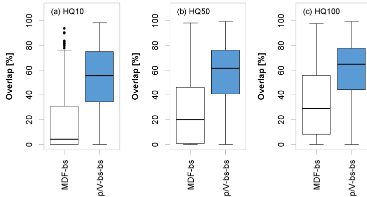
Figure 14. Percentage overlap for the three flood quantiles as per Eq. 12 computed from the 95% confidence intervals of mean daily flow (MDF) sample and parameter uncertainty (MDF-bs) and p/V-Lmoms total uncertainty (p/V-bs-bs). The boxplots are obtained by considering validation sites with more than 30 years of observations.
