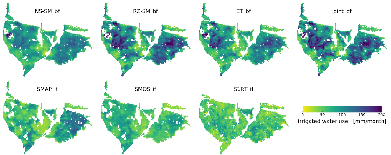
Figure 7: Mean monthly main irrigation season maps for 2016 and 2017 from four baseline and three SM-based inversion frameworks. The main irrigation season is assumed April – October.
