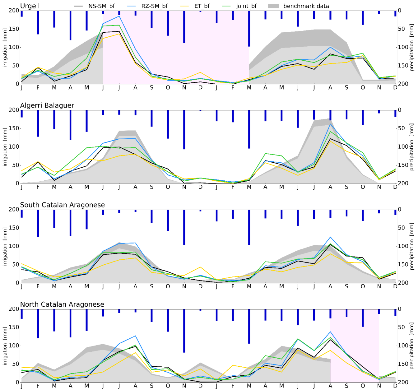
750 Figure 3: Irrigation estimates from the four approaches within the baseline framework. Estimates are shown for each of the four irrigation districts for the period 2016 – 2017 and compared with the benchmark. The gray shaded area shows the benchmark with and without irrigation water losses due to irrigation efficiency. Dark blue bars show precipitation amounts. Light red areas mark missing benchmark observations.
