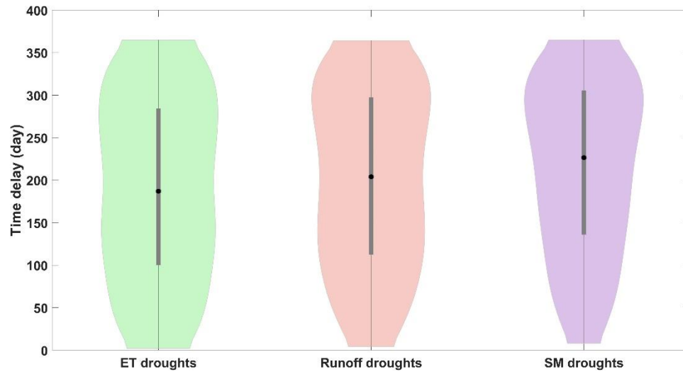
Figure S1. Violin boxplot of time delay for the ET, Runoff, and SM drought in all cascading drought events
