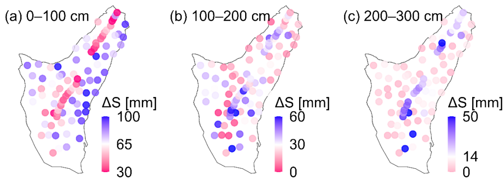
465 Fig. 10. Spatial pattern of annual soil moisture storage change ( \Delta S ) integrated over depths of (a) 0-100 cm, (b) 100-200 cm, and (c) 200-300 cm. In the top 100 cm of the soil profile (a), soil moisture changes are much greater on the hillslopes than in the gully, and greater on the NW-facing slope than on the SE-facing slope. These differences become less distinct between 100 and 200 cm (b), and become almost indistinguishable below 200 cm (c), where instead the greatest soil moisture changes occur in the gully. Note that the color scales differ among the three panels. Blue colors indicate changes that are larger than the catchment average; red values indicate changes that are smaller than the catchment average.
