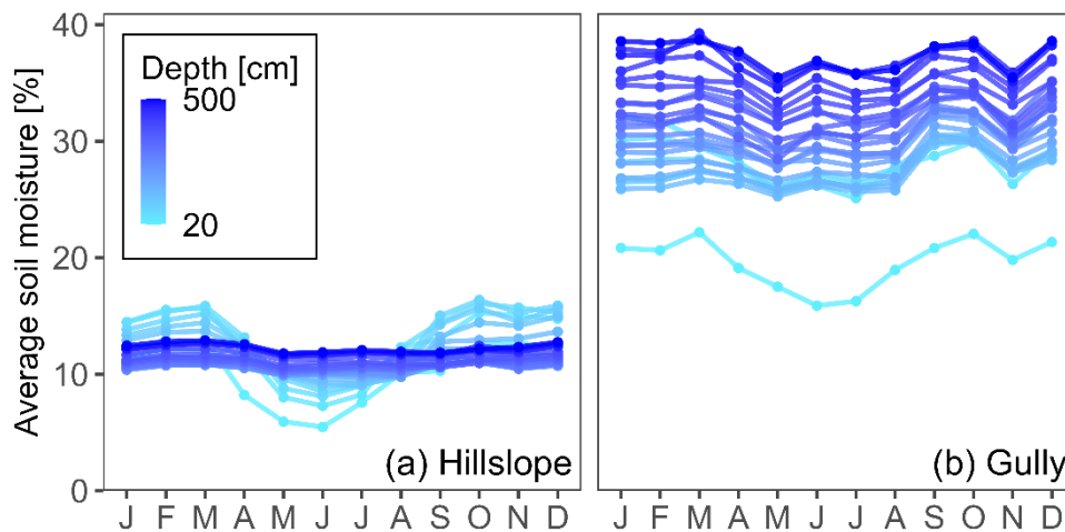
275 Fig. 2. Seasonal changes of the average soil moisture for (a) hillslope ( \theta_{hillslope,j,k} ) and (b) gully sites ( \theta_{gully,j,k} ). The capital letters on the x-axis indicate the months from January (J) to December (D). The light blue and dark blue colors indicate the average soil moisture in the shallow and deep soils, respectively. The soils in the gully were much wetter than those on the hillslopes. The rank order of soil moisture with depth reversed between winter and summer on the hillslopes, but exhibited little seasonal variation for the gully.
