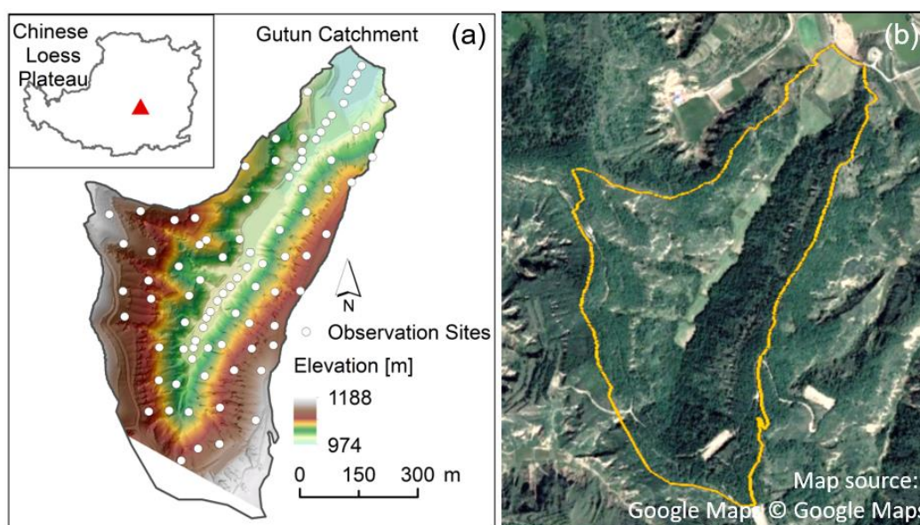
135 Fig. 1. (a) Map of the Gutun catchment showing the distribution of the 89 monitoring sites for volumetric soil moisture; (b) a satellite imagery from © Google Maps (taken in 2020) showing the relatively lush vegetation on the northwest-facing slope. The inset in (a) shows the location of the catchment in the Loess Plateau.
