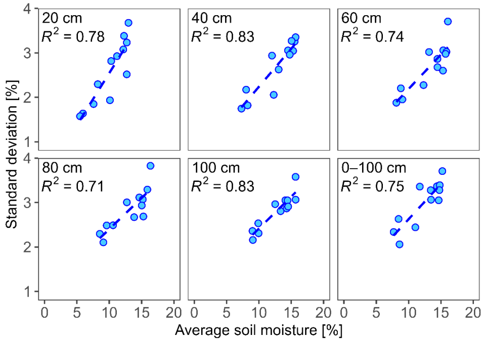
Fig. 8. Relationships between the monthly spatial standard deviation ( \sigma_{j,k} ) and monthly average soil moisture at slope sites ( \theta_{hillslope,j,k} ), for each depth within the top 100 cm of soil and for the profile average. Each point represents a different month of the year. The lines were fitted using a simple linear regression ( R^2 : 0.71-0.83). The standard deviation increased roughly linearly with increasing average soil moisture across hillslope sites.
