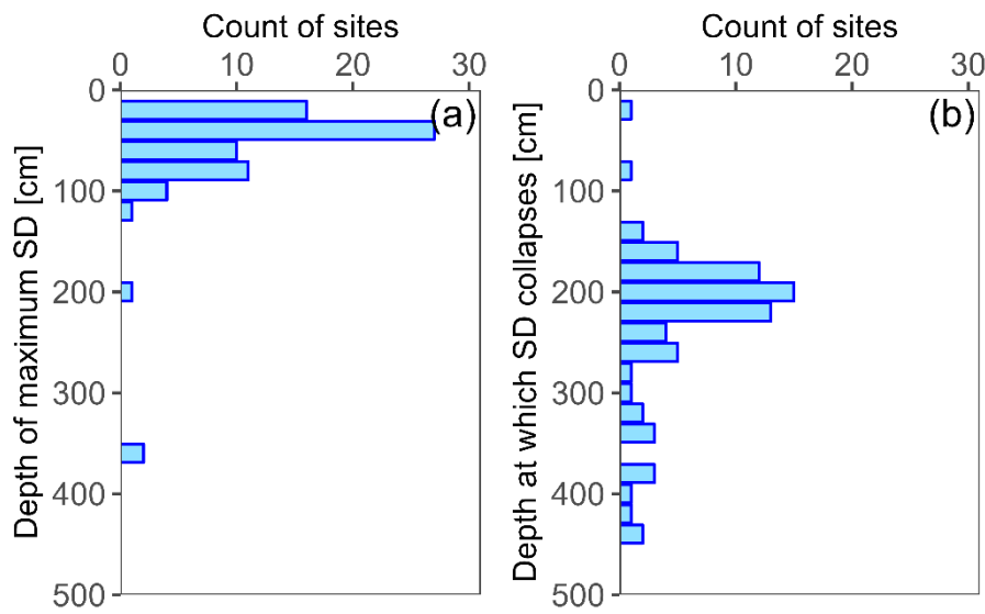
Fig. 4. (a) Depth of maximum standard deviation ( \sigma_{i,k} ) and (b) depth at which the standard deviation ( \sigma_{i,k} ) collapses (i.e., converges to a small value) for 72 monitoring sites. The remaining 17 monitoring sites were excluded from the analyses because they had several null values for deeper soils, making it impossible to calculate the depth at which the standard deviation collapses. The depth of the maximum standard deviation was between 20 and 100 cm for 94% of the sites. The depth at which it collapses was between 160 cm and 260 cm for 75% of the sites.
