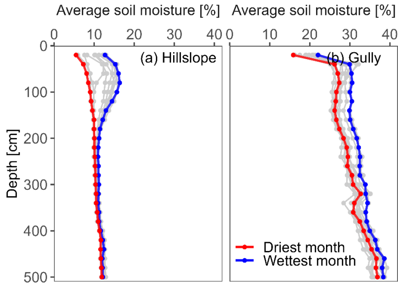
280 Fig. 3. The vertical patterns of average soil moisture (a) on the hillslope ( \theta_{hillslope,j,k} ) and (b) in the gully (b) (\theta_{gully,j,k}) . The blue line shows the soil moisture profile for the wettest month (October) and the red line for the driest month (June). The light grey lines show the profiles for the other ten months. The soil moisture on the hillslopes varied more as a function of depth in the wettest month than in the driest month, while the profiles in the gully were almost equally steep in the wettest and driest months. Seasonal 285 variations in average monthly soil moisture content were almost exclusively confined to the upper 260 cm on the hillslopes, but persisted over the full range of depths in the gully.
