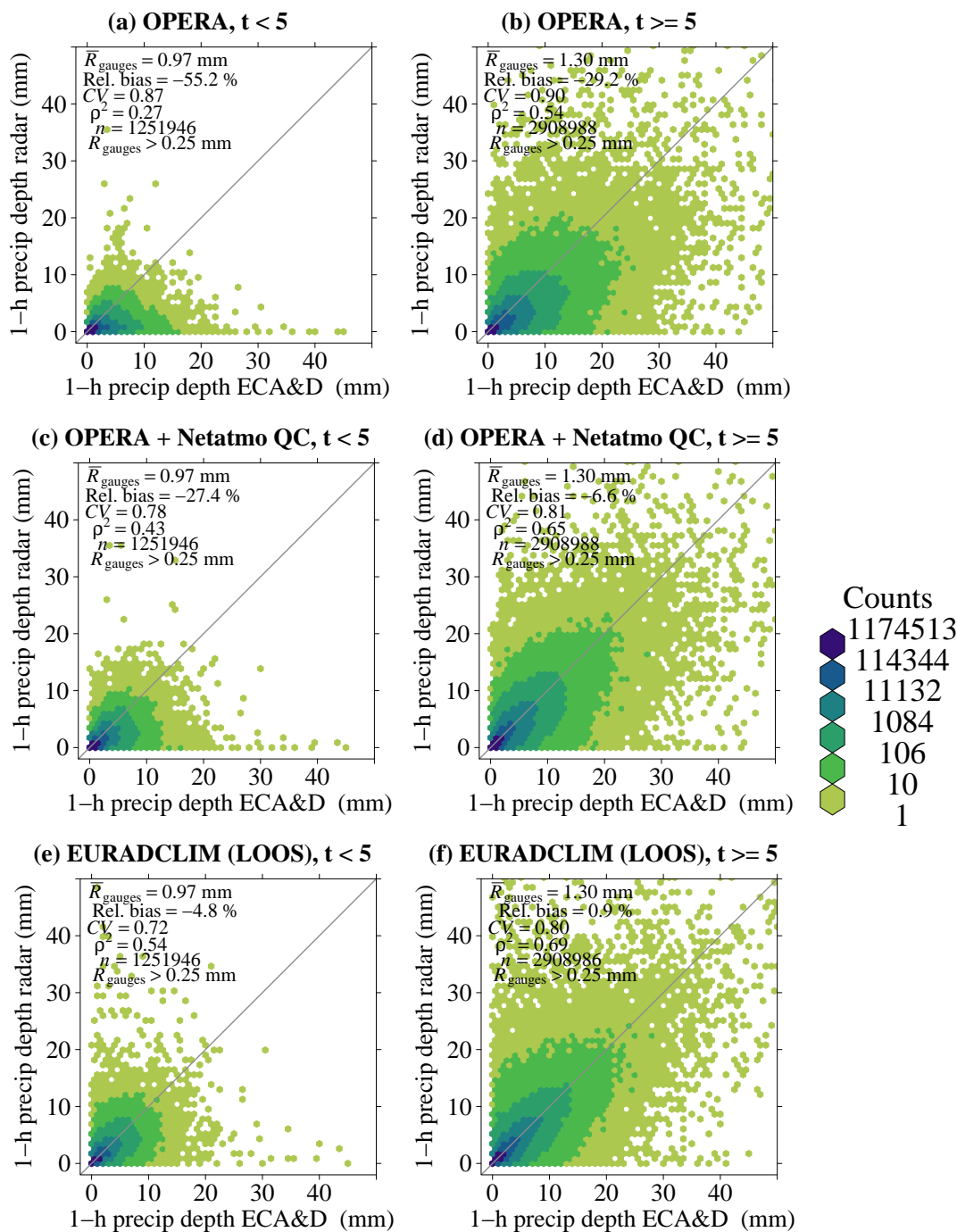
Figure 6. Scatter density plots of 1-h radar precipitation accumulations against ECA&D rain gauges over the period September 1, 2019–August 31, 2020. Disaggregated clock-hourly gauge precipitation accumulations are employed. Results are shown for the unadjusted OPERA dataset (a–b), for a merged OPERA-Netatmo dataset (c–d), and for the EURADCLIM dataset (e–f). For each dataset, results are shown for 1-h accumulations on days with mean daily air temperature < 5^\circ\text{C} (a, c, e) and \geq 5^\circ\text{C} (b, d, f). The independent verification for EURADCLIM is performed via leave-one-out statistics (LOOS).
