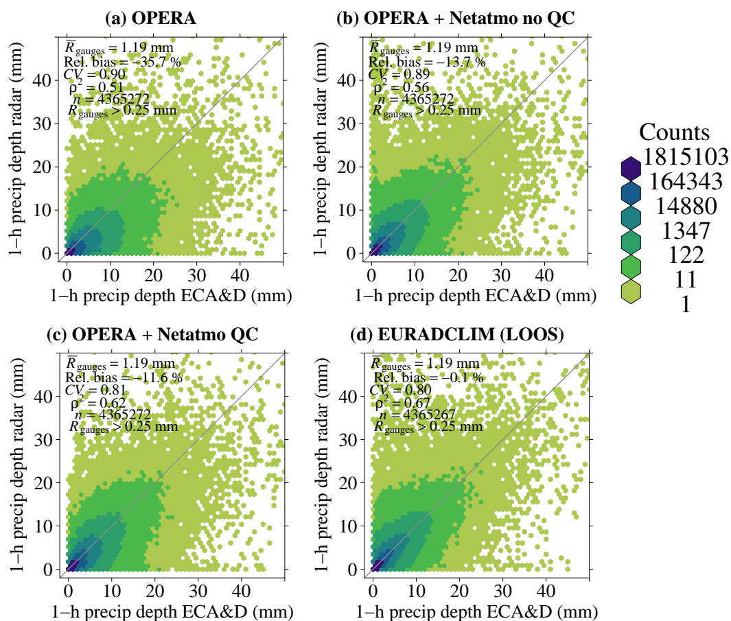
Figure 4. Scatter density plots of 1-h radar precipitation accumulations against disaggregated ECA&D rain gauge precipitation accumulations over the period September 1, 2019–August 31, 2020. Results are shown for the unadjusted dataset (a), for the merged OPERA-Netatmo datasets without (b) and with (c) quality control (QC) on Netatmo gauge data, and for the gauge-adjusted EURADCLIM dataset (d). The independent verification for EURADCLIM is performed via leave-one-out statistics (LOOS).
