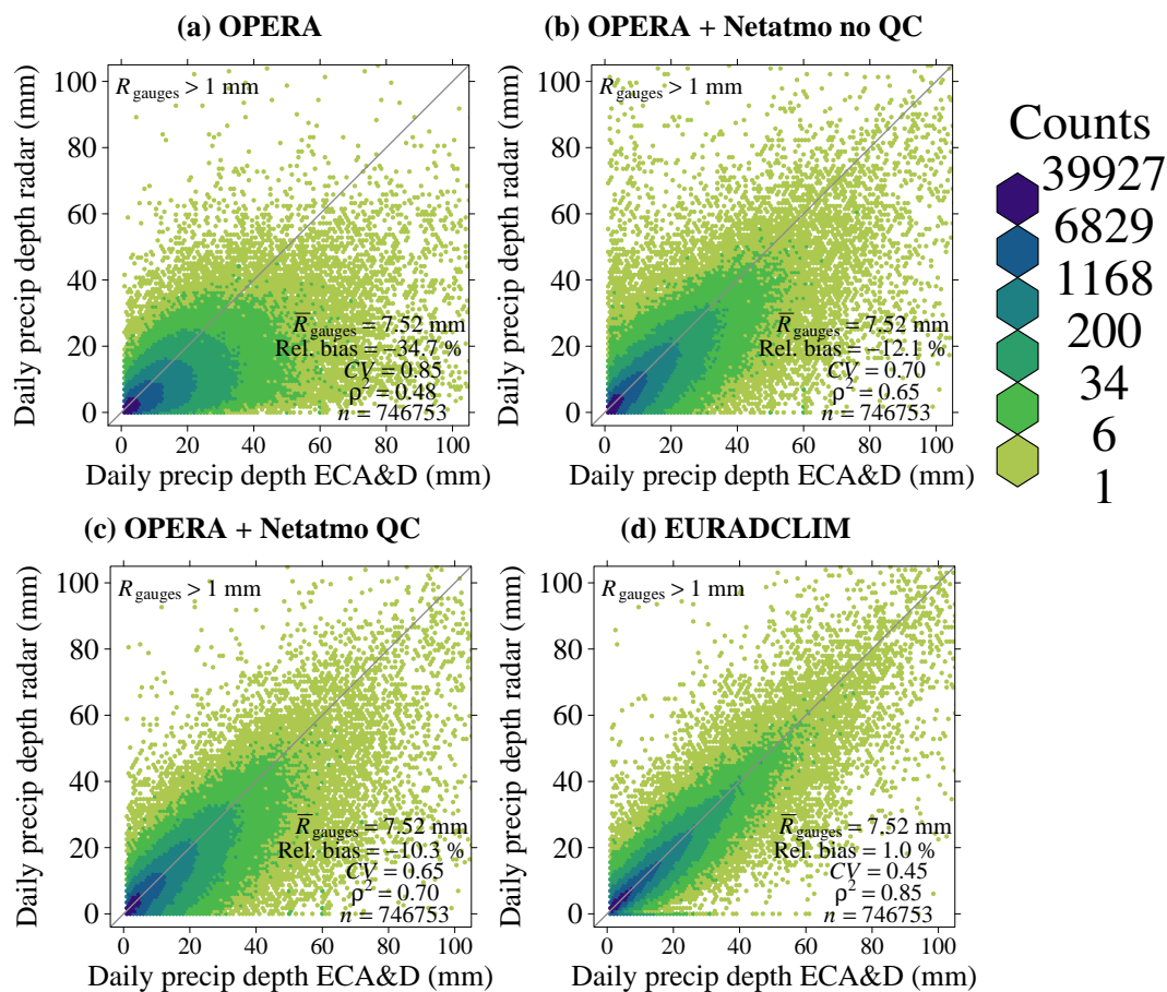
Figure 3. Scatter density plots of daily radar precipitation accumulations against ECA&D rain gauges (default measurement interval) over the period September 1, 2019–August 31, 2020. Results are shown for the unadjusted dataset (a), for the merged OPERA-Netatmo datasets without (b) and with (c) quality control (QC) on Netatmo gauge data, and for the gauge-adjusted EURADCLIM dataset (d). Note that the latter is not an independent verification.
