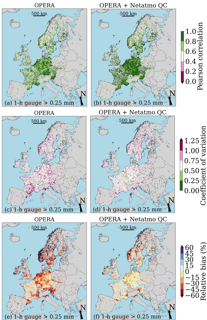
Figure 5. Spatial evaluation of 1-h precipitation accumulations against disaggregated clock-hourly ECA&D gauge precipitation accumulations over the period September 1, 2019–August 31, 2020. As indicated in Figure 1a, fewer ECA&D data are available for some gauge locations and hence the evaluation period is shorter. Verification results are displayed for the unadjusted OPERA radar dataset (a, c, e) and for the gauge-adjusted OPERA-Netatmo dataset (b, d, f). Maps made with Natural Earth. Free vector and raster map data ©naturalearthdata.com.
