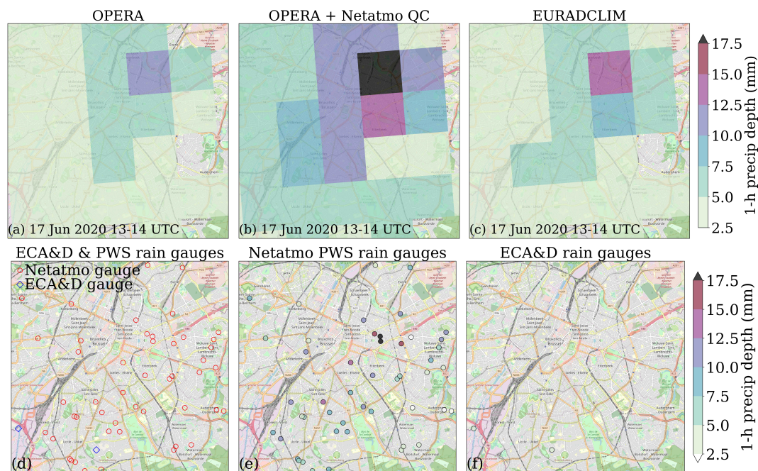
Figure 9. An extreme urban precipitation event over the city of Brussels, Belgium, from June 17, 2020 1300–1400 UTC (1-h precipitation accumulation). Accumulations are shown for the unadjusted OPERA (a), merged OPERA-Netatmo (b) and EURADCLIM (c) datasets. Locations of Netatmo and ECA&D gauges and their values are also provided (d–f). Map data ©OpenStreetMap contributors 2023. Distributed under the Open Data Commons Open Database License (ODbL) v1.0.
