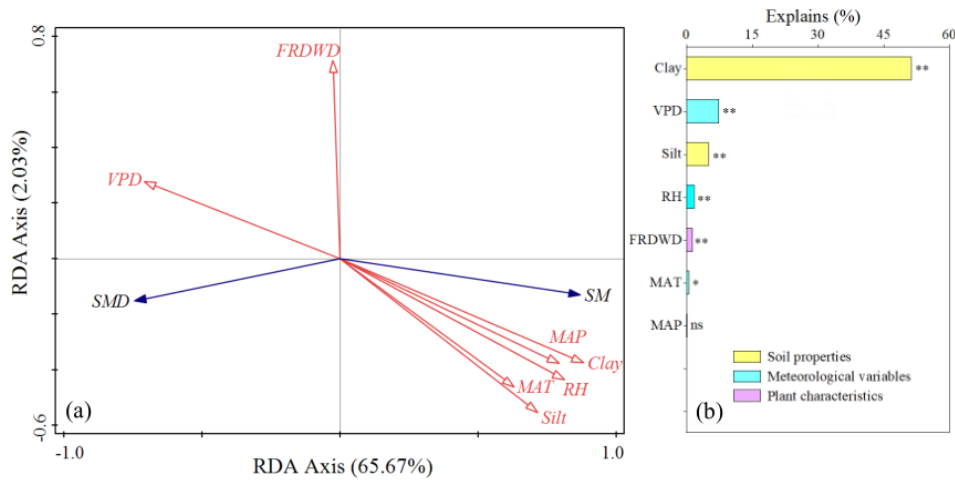
340 Figure 6: (a) the redundancy analysis (RDA) of “response variable (soil moisture deficit (SMD), soil moisture (SM, grav-%)) and environmental factors” is based on literature and field measured data. Descriptors (red arrows) are soil properties (clay and silt), meteorological variables (vapor pressure deficit ( VPD , kPa), mean annual precipitation ( MAP , mm), relative humidity ( RH ), and mean annual temperature ( MAT , °C)), and plant characteristic (fine root dry weight density ( FRDWD , g m -3 )). Axis 1 (65.67%, p <0.01) and Axis 2 (2.03%, p <0.01) are shown. (b) explanation provided by of each environmental variable for the response variables. **, *, and ns following the bar chart indicate that p <0.01, p <0.05, and no significant, respectively. 345
