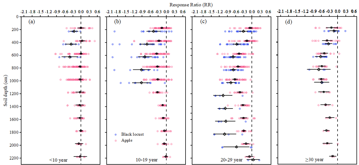
270 Figure 2: Mean effect sizes indicating the mean value of response ratio ( RR , a unit-free index with positive or negative value means soil moisture increases or decreases with the older of plantations) of soil moisture with the age of plantation on the Loess Plateau are divided into: (a) tree age <10 year, (b) 10 \text{ year} \leq \text{tree age} < 20 \text{ year} , (c) 20 \text{ year} \leq \text{tree age} < 30 \text{ year} , and (d) tree age \geq 30 \text{ year} . The vertical black dotted lines indicate RR=0 . Blue and red dots, which involves 11980 literature extraction data and 4200 field sampling data, represent black locust ( R. pseudoacacia ) forests and apple orchard RR s, respectively; diamonds and circles represent the mean RR of R. pseudoacacia and apple ( M. pumila ) orchard, respectively; and the error bars represent 95%CI.
