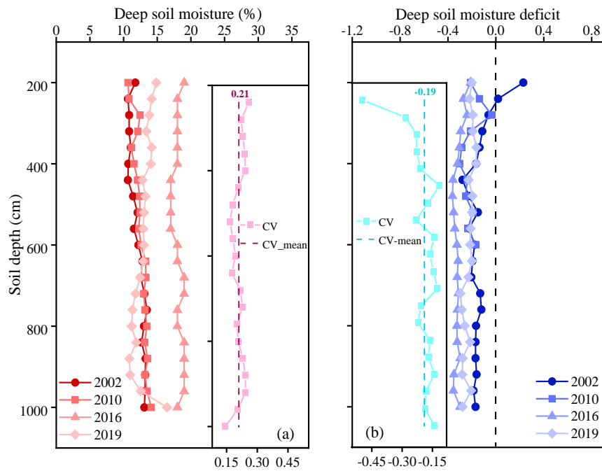
Figure 3: Distribution of deep soil moisture (a) and deep soil moisture deficit (b) of 15-year-old apple orchards in Changwu in 2002, 2010, 2016 and 2019, which is all based on literature extraction data. The variation coefficient (CV) of soil moisture and soil moisture deficit below 2 m are shown in the small figures, the dashed lines of which represent the mean values of the CV for deep soil moisture and deep soil moisture deficit, respectively.
