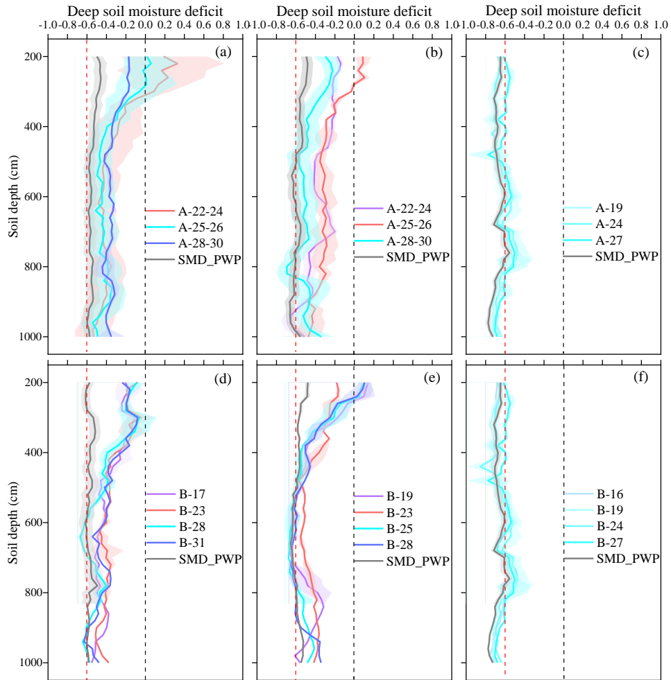
290 Figure 4: Deep soil moisture deficit (DSMD) distribution under apple orchards of different ages in Changwu (a), Luochuan (b) and Mizhi (c); and SMD under black locust forests of different ages in Changwu (d), Yan'an (e) and Mizhi (f). The capital letters A and B in the legend represent apple and black locust, respectively, and the numbers after the letters represent tree age, for example, A-22 represents 22-year-old apple. (a) and (b) come from data extracted from literature, while (c)-(f) are both field measured data. In order to reduce the randomness 295 caused by different sampling years and locations between the extracted data, the data for apple trees with similar ages in Changwu (a) and Luochuan (b) were combined. The gray line indicates SMD at permanent wilting point (SMD_PWP) in each sampling site, and the red dashed line indicates the SMD equal to -0.6. The shaded portion corresponding to each line represents the positive and negative values of the standard deviation.
