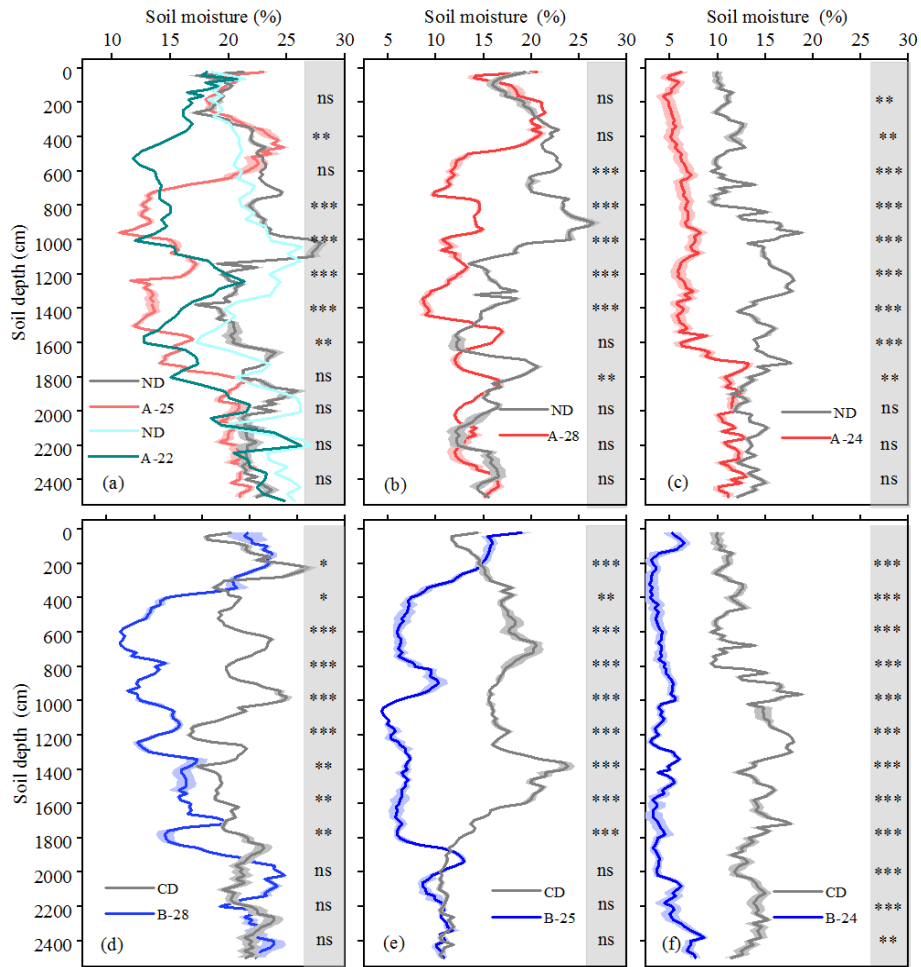
Figure 5: Dynamic distribution of maximum water absorption depth after reaching the moisture limitation of deep soil desiccation. The data of 22-year-old apple and cropland (dark green) in (a) belong to literature extraction data, and other data are field measured data. The capital letters A and B in the legend represent apple and black locust, respectively, and the numbers after the letters represent tree age, for example, A-22 represents 22-year-old apple. (a) and (d) indicate Changwu; (b) and (e) indicate Luochuan and Yan'an, respectively; (c) and (f) indicate Mizhi. Gray line represents soil moisture of grassland (CD) or farmland (ND). ***, **, * and ns in the gray bands indicate the significance level of measured data obtained by the paired sample t -test for p < 0.001 , p < 0.01 , p < 0.05 and no significant differences, respectively. The shaded portion corresponding to each line represents the positive and negative values of the standard deviation.
