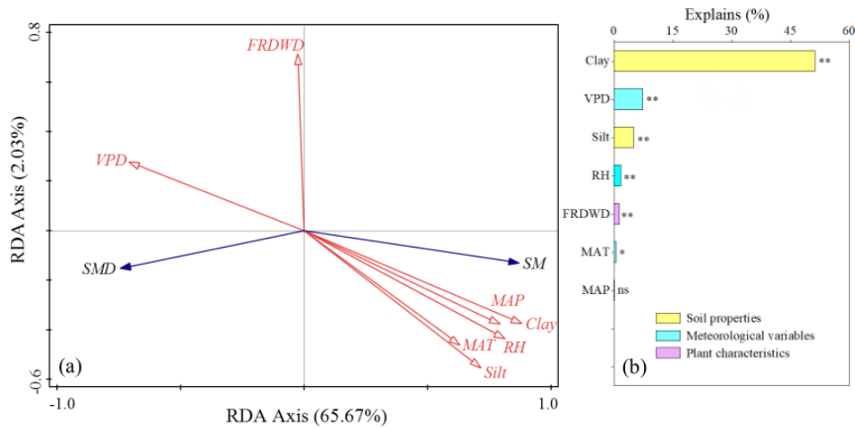
Figure 6: (a) the redundancy analysis (RDA) of “response variable (soil moisture deficit (SMD), soil moisture (SM)) and environmental factors” is based on literature and field measured data. Descriptors (red arrows) are soil properties (clay and silt), meteorological variables (vapor pressure deficit (VPD), mean annual precipitation (MAP), relative humidity (RH), and mean annual temperature (MAT)), and plant characteristic (fine root dry weight density (FRDWD)). Axis 1 (65.67%, p < 0.01 ) and Axis 2 (2.03%, p < 0.01 ) are shown. (b) explanation provided by of each environmental variable for the response variables. **, *, and ns following the bar chart indicate that p < 0.01 , p < 0.05 , and no significant, respectively.
