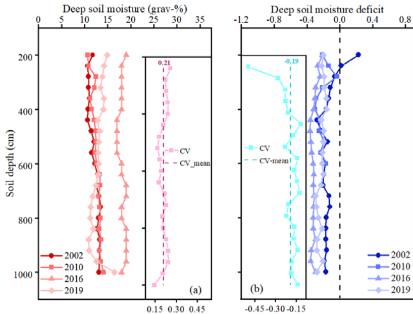
285 Figure 3: Distribution of deep soil moisture (grav-%, (a)) and deep soil moisture deficit (b) of 15-year-old apple ( M. pumila ) orchards in Changwu in 2002, 2010, 2016 and 2019, which is all based on literature extraction data. The variation coefficient (CV) of deep soil moisture and deep soil moisture deficit below 2 m are shown in the small figures, the dashed lines of which represent the mean values of the CV for deep soil moisture and deep soil moisture deficit, respectively.
