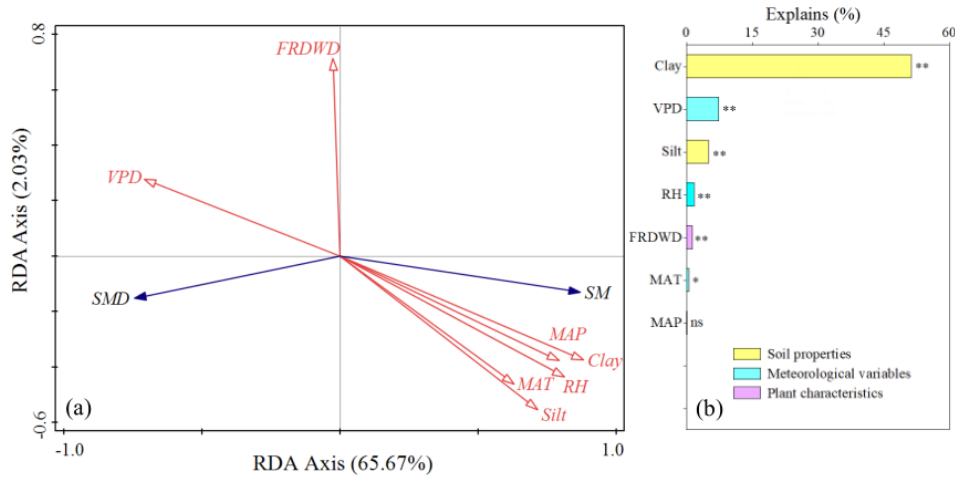
Figure 6: (a) the redundancy analysis (RDA) of “response variable (soil moisture deficit (SMD), soil moisture (SM, grav-% )) and environmental factors” is based on literature and field measured data. Descriptors (red arrows) are soil properties (clay and silt), meteorological variables (vapor pressure deficit (VPD, kPa ), mean annual precipitation (MAP, mm ), relative humidity (RH), and mean annual temperature (MAT, °C )), and plant characteristic (fine root dry weight density (FRDWD, g m -3 )). Axis 1 (65.67%, p < 0.01 ) and Axis 2 (2.03%, p < 0.01 ) are shown. (b) explanation provided by of each environmental variable for the response variables. **, *, and ns following the bar chart indicate that p < 0.01 , p < 0.05 , and no significant, respectively.
