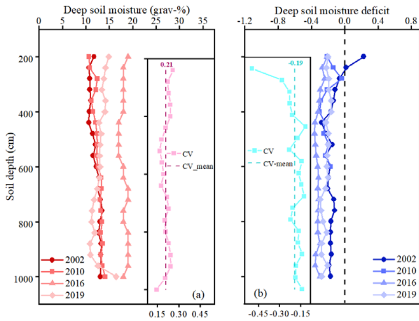
Figure 3: Distribution of deep soil moisture (grav-%, (a)) and deep soil moisture deficit (b) of 15-year-old apple orchards in Changwu in 2002, 2010, 2016 and 2019, which is all based on literature extraction data. The variation coefficient (CV) of deep soil moisture and deep soil moisture deficit below 2 m are shown in the small figures, the dashed lines of which represent the mean values of the CV for deep soil moisture and deep soil moisture deficit, respectively.
