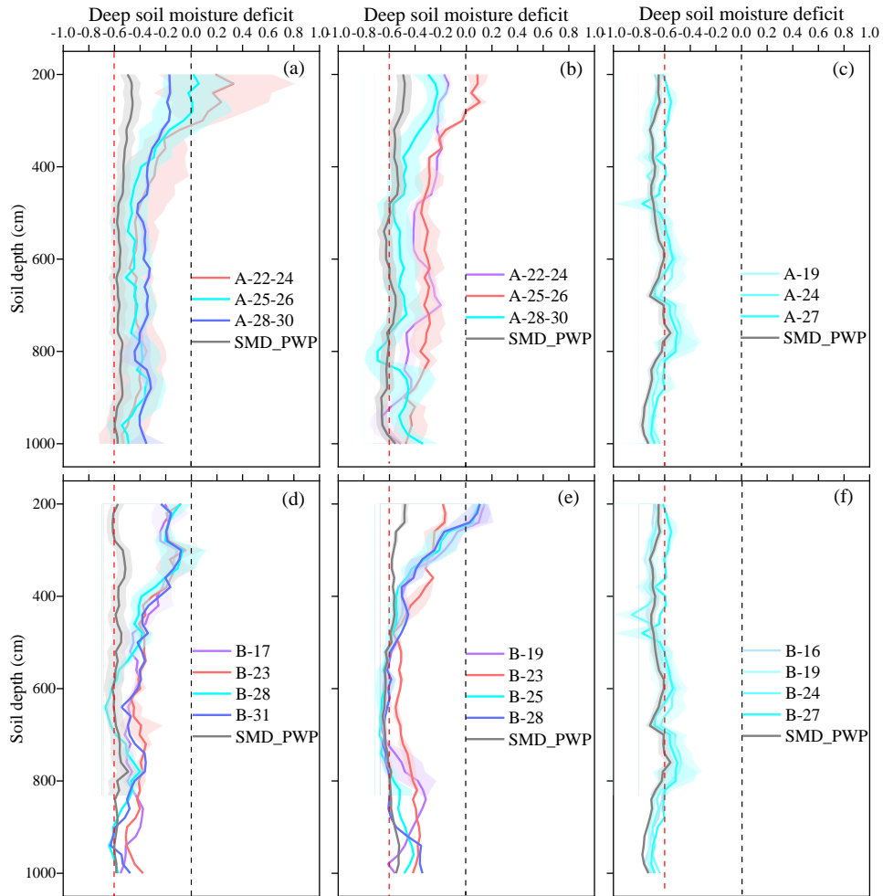
Figure 4: Deep soil moisture deficit (DSMD) distribution under apple ( M. pumila ) orchards of different ages in Changwu (a), Luochuan (b) and Mizhi (c); and SMD-soil moisture deficit under black locust ( R. pseudoacacia ) forests of different ages in Changwu (d), Yan'an (e) and Mizhi (f). The capital letters A and B in the legend represent M. pumila and R. pseudoacacia apple and black locust , respectively, and the numbers after the letters represent tree age, for example, A-22 represents 22-year-old M. pumila apple . (a) and (b) come from data extracted from literature, while (c)-(f) are both field measured data. In order to reduce the randomness caused by different sampling years and locations between the extracted data, the data for M. pumila apple trees with similar ages in Changwu (a) and Luochuan (b) were combined. The gray line indicates soil moisture deficit (SMD) at permanent wilting point (SMD_PWP) in each sampling site, and the red dashed line indicates the soil moisture deficit (SMD) equal to -0.6. The shaded portion corresponding to each line represents the positive and negative values of the standard deviation.
