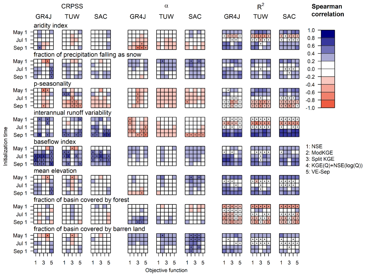
865 Figure 10. Spearman's rank correlation coefficients between catchment characteristics (shown in different rows) and the CRPSS (left), \alpha reliability index (center), and the coefficient of determination R^2 (right) obtained for seasonal streamflow hindcasts (period April/1987 – March/2020), produced with the five representative objective functions (x-axis in each color matrix), different initialization times (y-axis in each color matrix), and the three hydrological models. Black dots indicate statistically significant ( p < 0.05 ) correlations.
