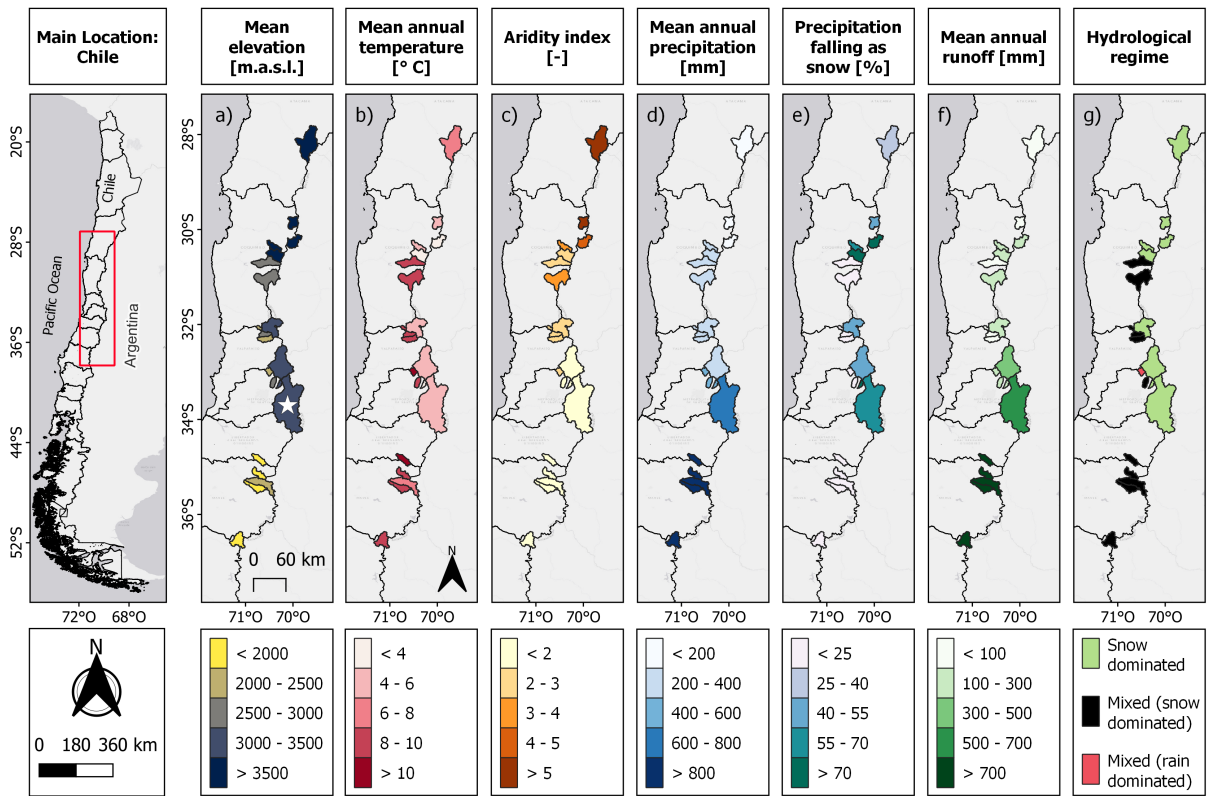
810 Figure 1. Location and spatial variability of catchment characteristics across the study domain. Hydroclimatic attributes are computed for the period April/1987 – May/2020 using data retrieved from the CAMELS-CL database (see details in Section 2). The white star in panel (a) denotes the outlet of the Maipo en El Manzano River basin, for which the analysis approach is illustrated (see section 4.1).
