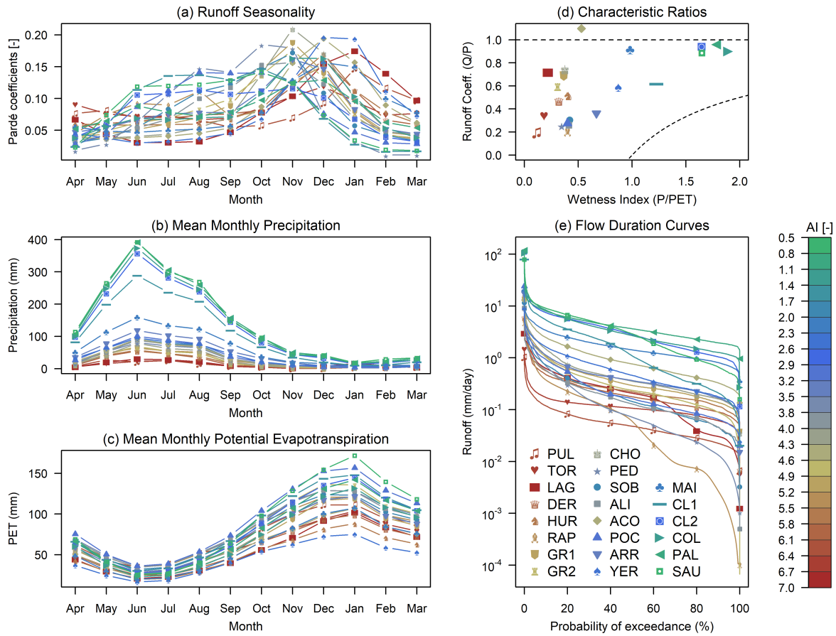
815 Figure 2. Study basins' characteristics: (a) runoff seasonality, (b) mean monthly precipitation, (c) mean monthly potential evapotranspiration, (d) characteristic ratios, and (e) daily flow duration curves (FDC). These graphs correspond to the period April/1987 – March/2020 and were produced using data retrieved from the CAMELS-CL database (see details in Section 2). In the legend (panel e), the basins are ordered from north (PUL) to south (SAU), and the colors indicate their aridity indices (AI; green to red – lower to higher index).
