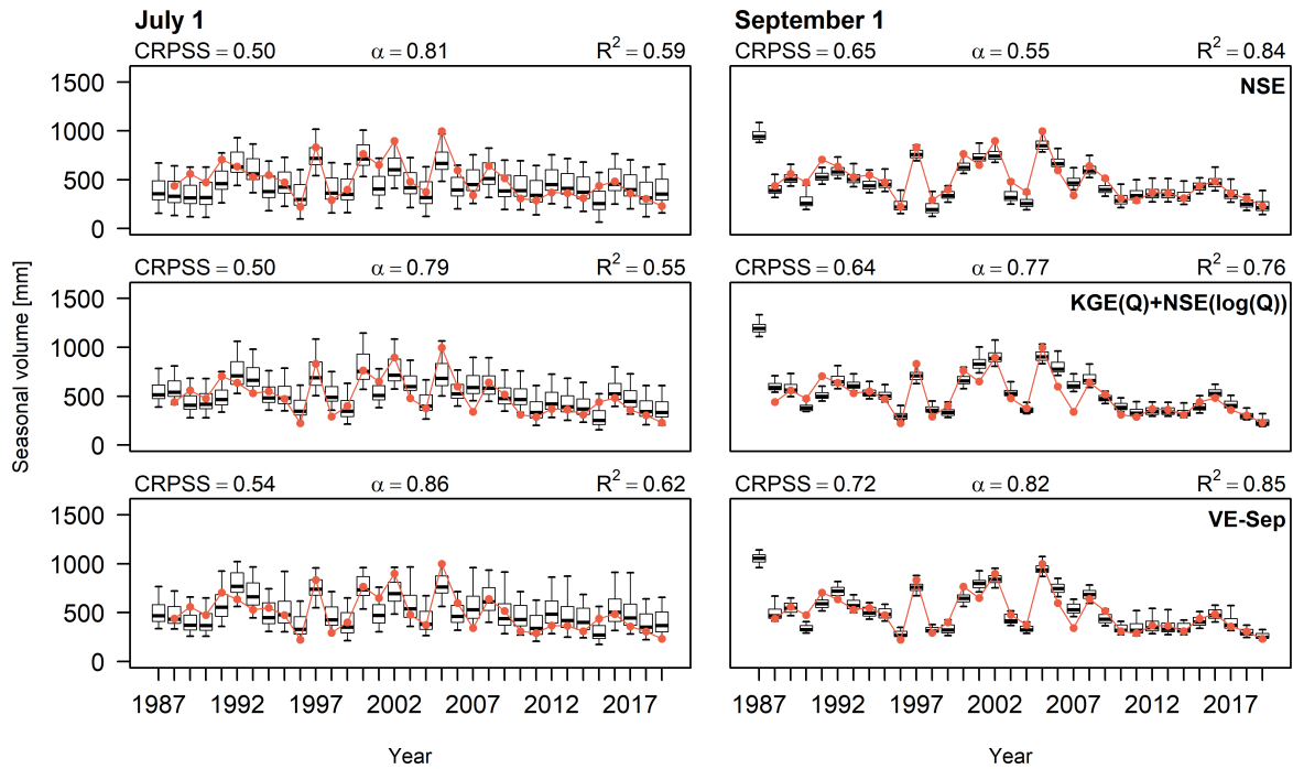
830 Figure 5. Time series with ESP seasonal hindcasts (i.e., September-March runoff) initialized on July 1 (left panels), and September 1 (right panels) for the Maipo at El Manzano basin. The boxes correspond to the interquartile range (IQR, i.e., 25th and 75th percentiles); the horizontal line in each box is the median, whiskers extend to the \pm 1.5 \cdot IQR of the ensemble, and the red dots represent the observations. The results were produced with the TUW model, using parameters obtained from calibrations conducted with NSE, KGE(Q)+NSE(log(Q)) and VE-Sep (see details in Section 3.1). Each panel displays the CRPSS, the reliability index \alpha , and the coefficient of determination R^2 (computed using the ensemble hindcast median).
