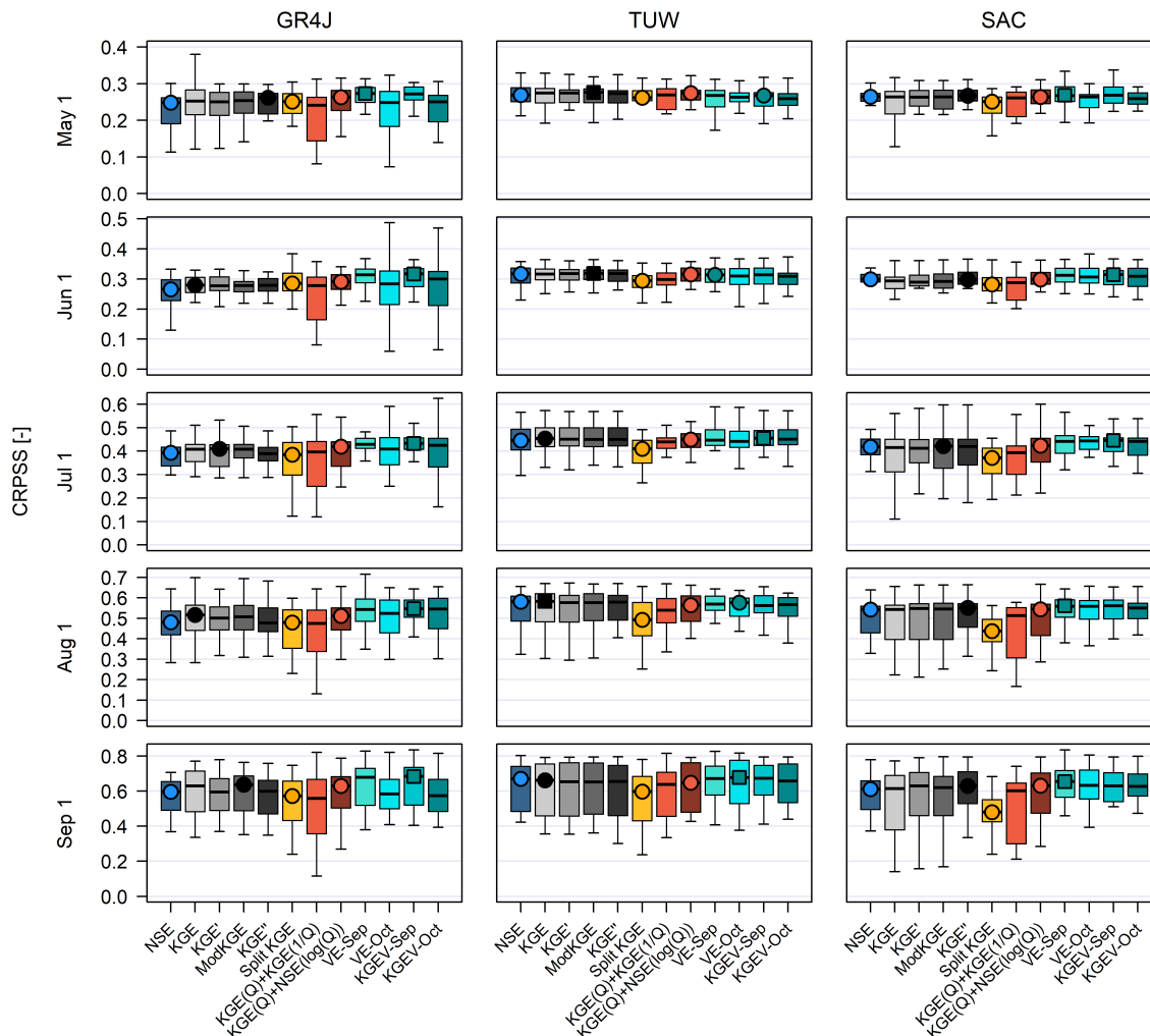
840 Figure 6. Comparison of CRPSS obtained with different calibration objective functions. Each panel contains results for a specific combination of initialization time (rows) and hydrological model (columns), and each boxplot comprises results from the 22 case study basins. The boxes correspond to the interquartile range (IQR, i.e., 25th and 75th percentiles), the horizontal line in each box is the median, and whiskers extend to the \pm 1.5 \cdot IQR of the ensemble. The circle indicates the objective function providing the highest median within each family of calibration metric (identified with different colors), and the square indicates the objective function that delivers the best set of metric values using a specific combination of initialization time and hydrological model.
