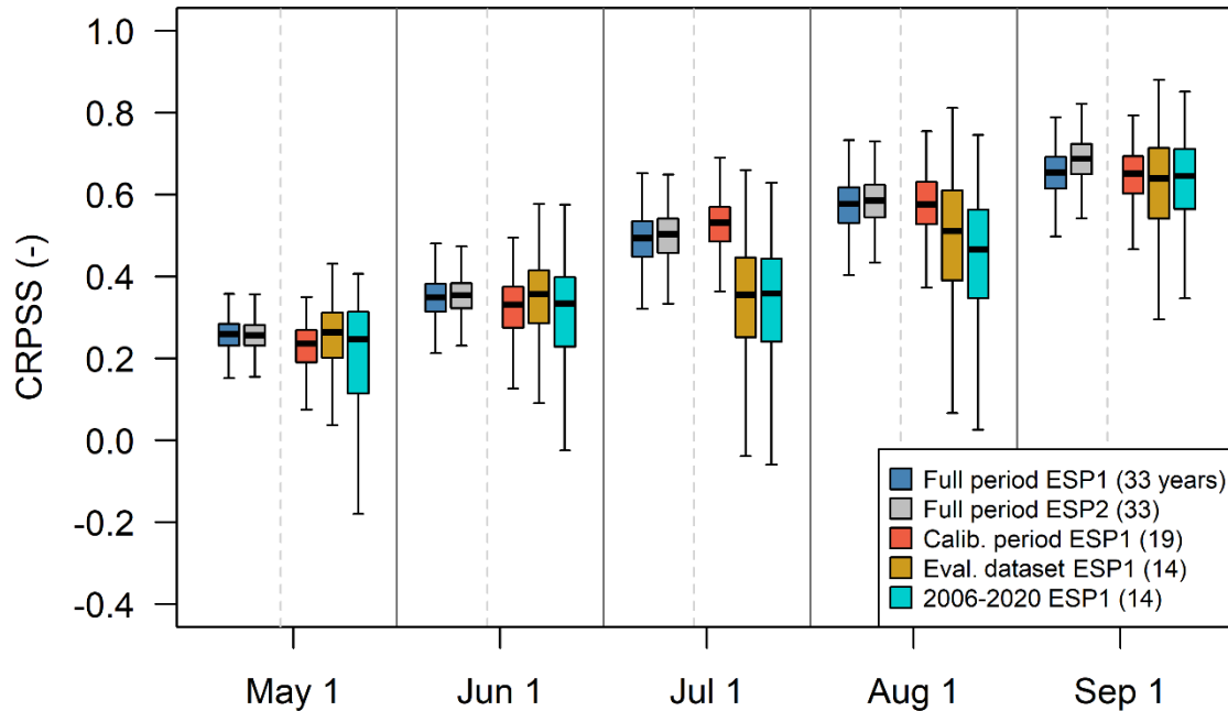
870 Figure 11. Comparison of CRPSS values for seasonal (i.e., September-March) streamflow hindcasts produced at the Maipo River basin with the TUW model and KGE(Q)+NSE(\log(Q)) as calibration metric. Each box comprises results from 1000 bootstraps with replacement applied to different verification sample sizes (i.e., number of hindcast-observation pairs): (a) full period (i.e., 33 WYs) using the same parameter set, obtained by calibrating the model with data from the period April/1994 – March/2013 (blue); (b) full period, using parameter sets re-calibrated with all data except the hindcasted year (i.e., 33 parameter sets to produce 33 seasonal hindcasts, gray); (c) 19 WYs (calibration periods), using a single parameter set obtained with data from the same period (red); (d) 875 14 WYs (i.e., evaluation data set April/1987 – March/1994 and April/2013 – March/2020), using the same parameter set as in case (c) (orange); and (e) 14 WYs (April/2006 – March/2020), using the same parameter set as in case (c) (cyan). The boxes correspond to the interquartile range (IQR, i.e., 25th and 75th percentiles); the horizontal line in each box is the median, and the whiskers extend to the \pm 1.5 \cdot IQR of the ensemble.
