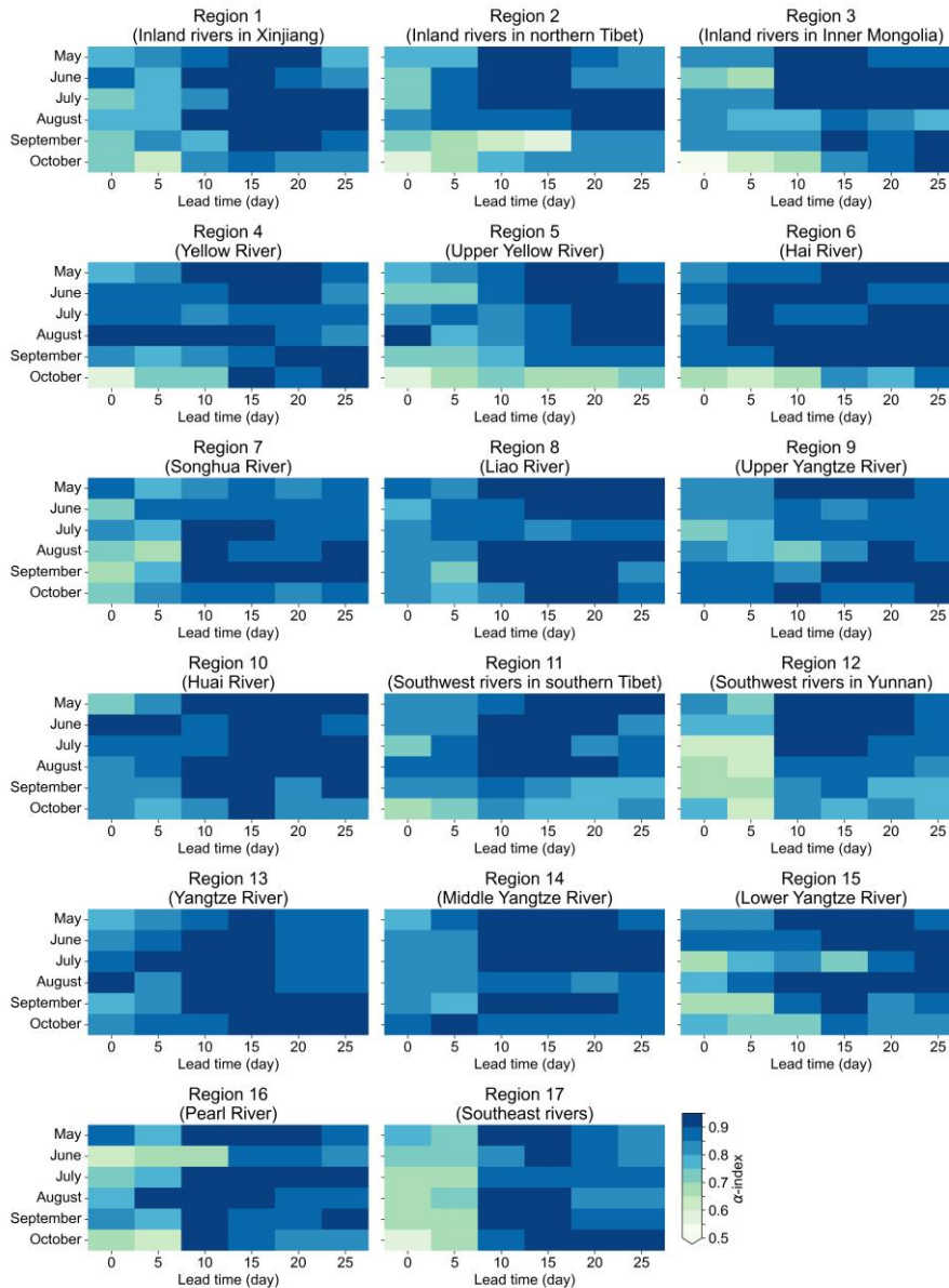
Figure 910. Same as Figure 9, but for \alpha -index.
