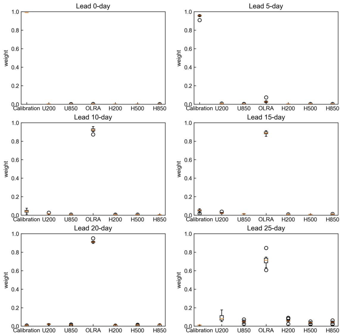
Figure 78. Box plots showing the distribution of model weights at different lead times in cross-validation for Region 1 (Inland rivers in Xinjiang) in May.
