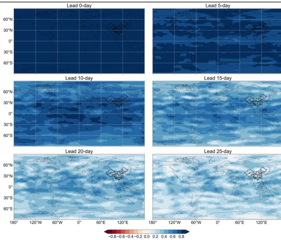
320 Figure 4. Temporal correlation coefficient (TCC) of the ensemble mean of U200 intraseasonal signals derived from the ECMWF model compared to the ERA5 reanalysis data in May. Correlation coefficients that are statistically significant at the 5 % level are shaded.
