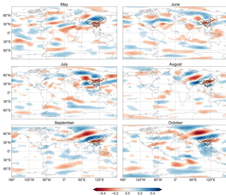
300 Figure 2. Correlation coefficient between pentad mean 10–60 d signals of U200 and precipitation over Region 1 (inland rivers in Xinjiang) in different months. Correlation coefficients that are statistically significant at the 5 % level are shaded.
