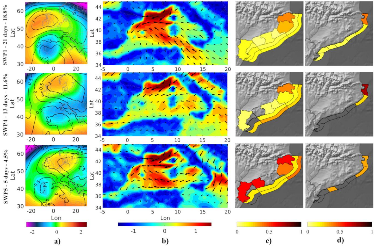
Figure 7. Compound SWP associated with P_{24} > 200\text{mm} and coastal storms of C \geq IV and H_s \geq 4\text{ m} . (a) z500 anomaly (colormap) overlaid with mslp anomaly (contours). (b) Wind anomaly. (c) Probability of P_{24} \geq 100\text{ mm} (land) at each basin; probability of storm power content of class \geq IV (internal coastal band) and probability of H_s \geq 4\text{m} (external coastal band) at each coastal sector. (d) Spatial distribution of multivariate severe events of P_{24} \geq 100\text{mm} with a coastal storm of class \geq II and H_s \geq 4\text{m} .
