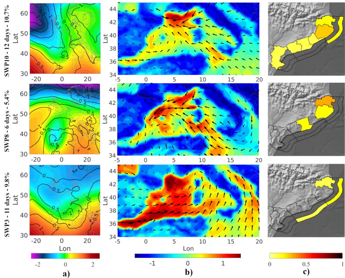
435 Figure 10. Compound SWP associated with 100 \text{ mm} \leq P_{24} \leq 200 \text{ mm} coastal storms of \text{II} \leq \text{C} \leq \text{IV} with H_s \geq 4 \text{ m} . (a) z_{500} anomaly (colormap) overlaid with mslp anomaly (contours). (b) Wind anomaly. (c) Probability of P_{24} \geq 100 \text{ mm} (land) at each basin; probability of storm power content of class \geq \text{IV} (internal coastal band) and probability of H_s \geq 4 \text{ m} (external coastal band) at each coastal sector. Please note that none of the SWPs were linked to severe multivariate episodes; therefore, the panels for such cases are not displayed.
