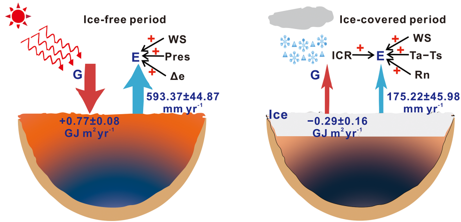
Figure 6. E and G in QHL during IFP and ICP. WS, Pres, \Delta e , T_a - T_s , R_n , and ICR are the wind speed, air pressure, vapor pressure difference, difference between T_a and T_s , net radiation, and ice coverage rate of the lake, respectively. The red plus sign indicates a positive effect of the variable on E .
