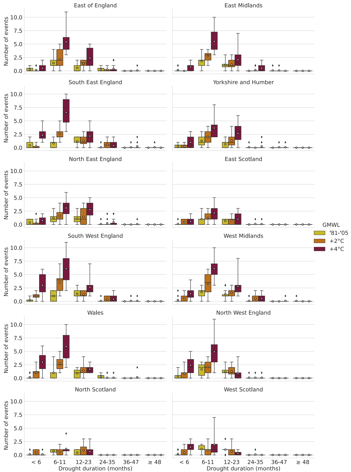
Figure S1. As Fig. 10, but for SPI6 < -2 (extreme drought).
