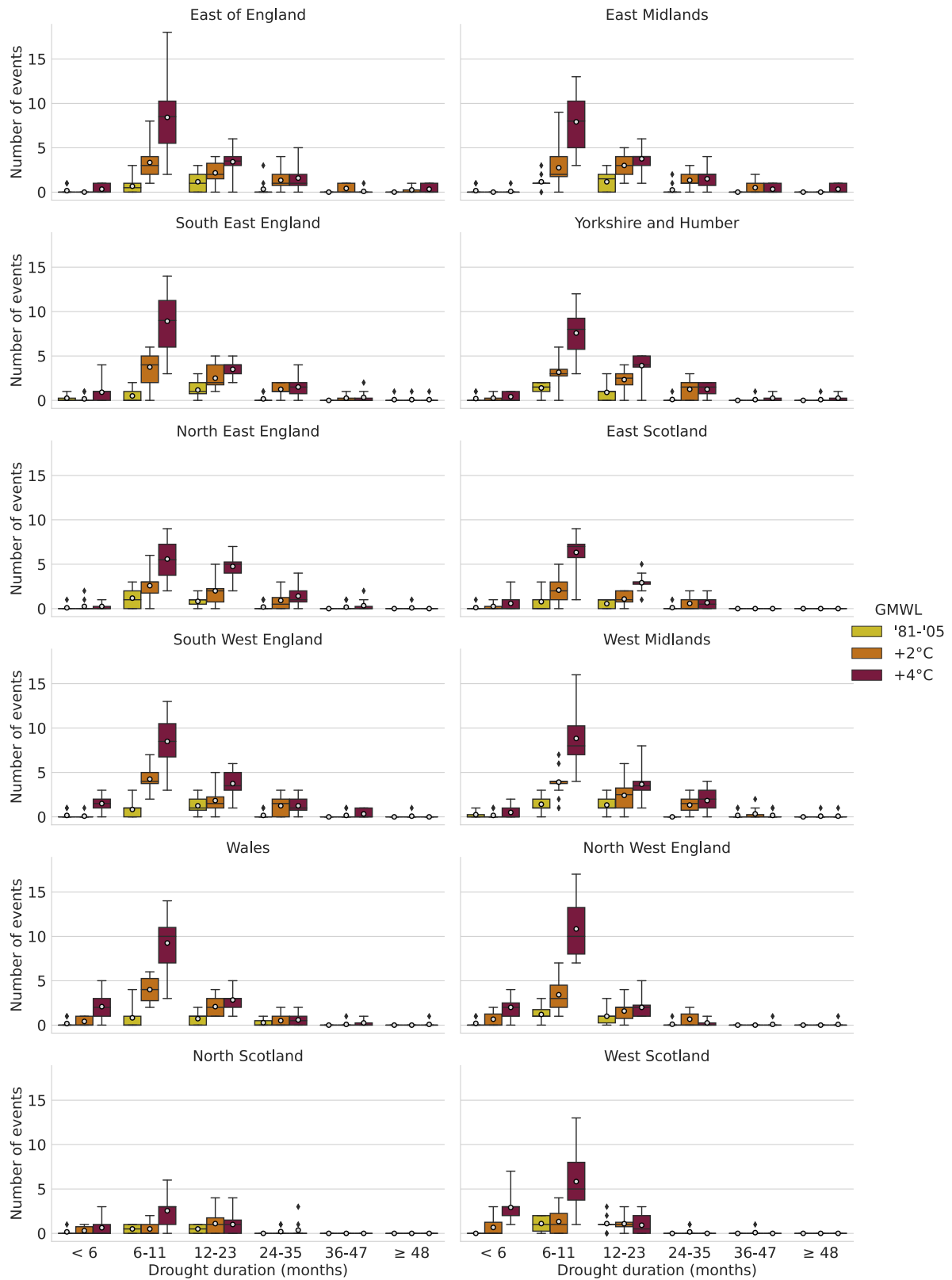
Figure S2. As Fig. 10, but for SPEI6 < -2 (extreme drought).
