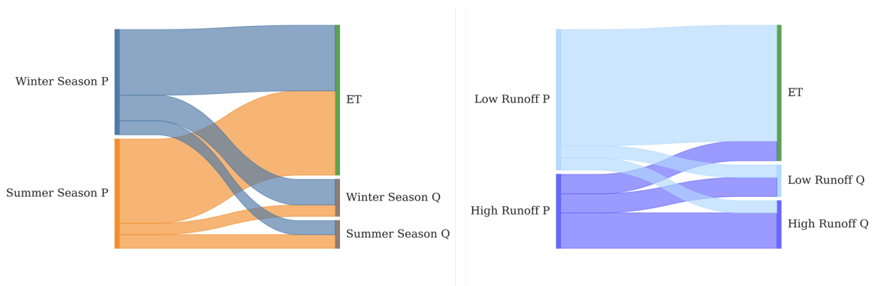
Figure 7 Left: Winter and summer season rainfall split into evapotranspiration (ET) and winter and summer season discharge (Q), respectively, based on Endmember splitting analyses (reading the diagram from left to right). Endmember mixing results, showing the source water for ET, winter and summer season Q, respectively (reading from right to left). Right: Similarly to the right, but splitting and mixing according to high flows (top 20%) and lower flows instead of season.
