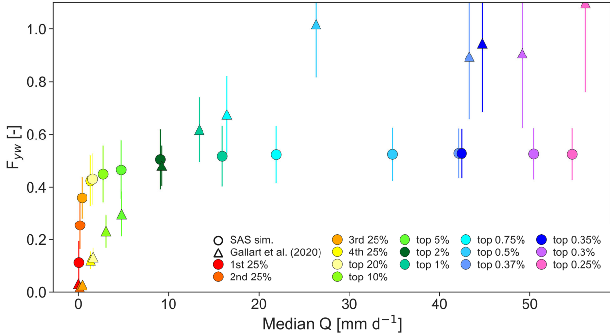
Figure 8 Comparison between the young water fraction, F_{yw} , as presented by Gallart et al. (2020) (diamondstriangles) with the fraction of stream water younger 45 days as simulated by the SAS model (pointscircles), as a function of increasing discharge quantiles (color code). The error bars represent standard deviations.
