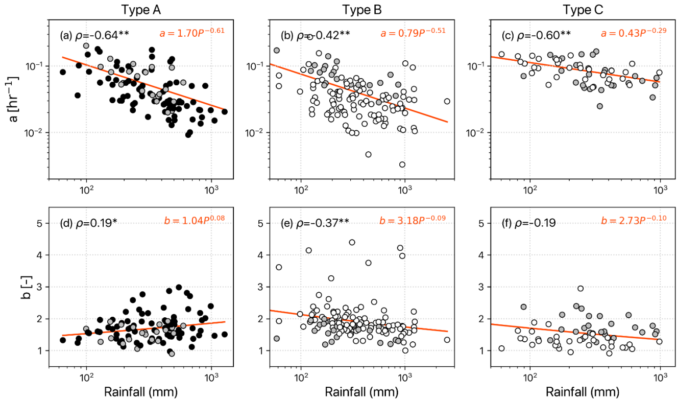
555 Figure 8: Scatter plots of recession parameters against total rainfall for recession segments at different catchment types. Type A are large catchments (area > 500 km 2 ), B are small catchments with low L/G ratios, and C are small catchments with high L/G ratios. Black, gray, and white dot colors represent the low, medium, and large L/G catchments, respectively. The orange line is the power-law fit curve with Spearman correlation coefficients in the upper-left corner of each panel (* and ** denote statistical significance at the 90% and 99% level of confidence, respectively).
