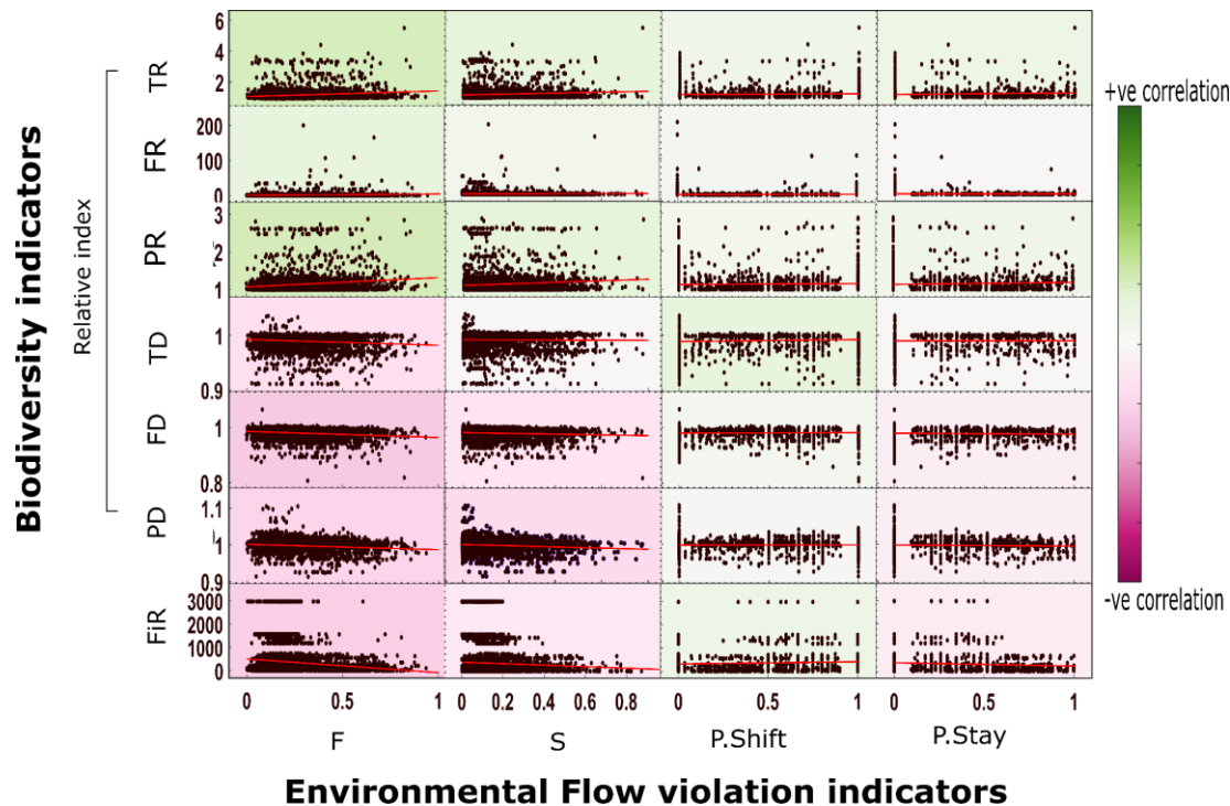
Fig. 3 Scatter between EF violation indices and biodiversity indices with linear fit and corresponding R value at globally aggregated scale.
