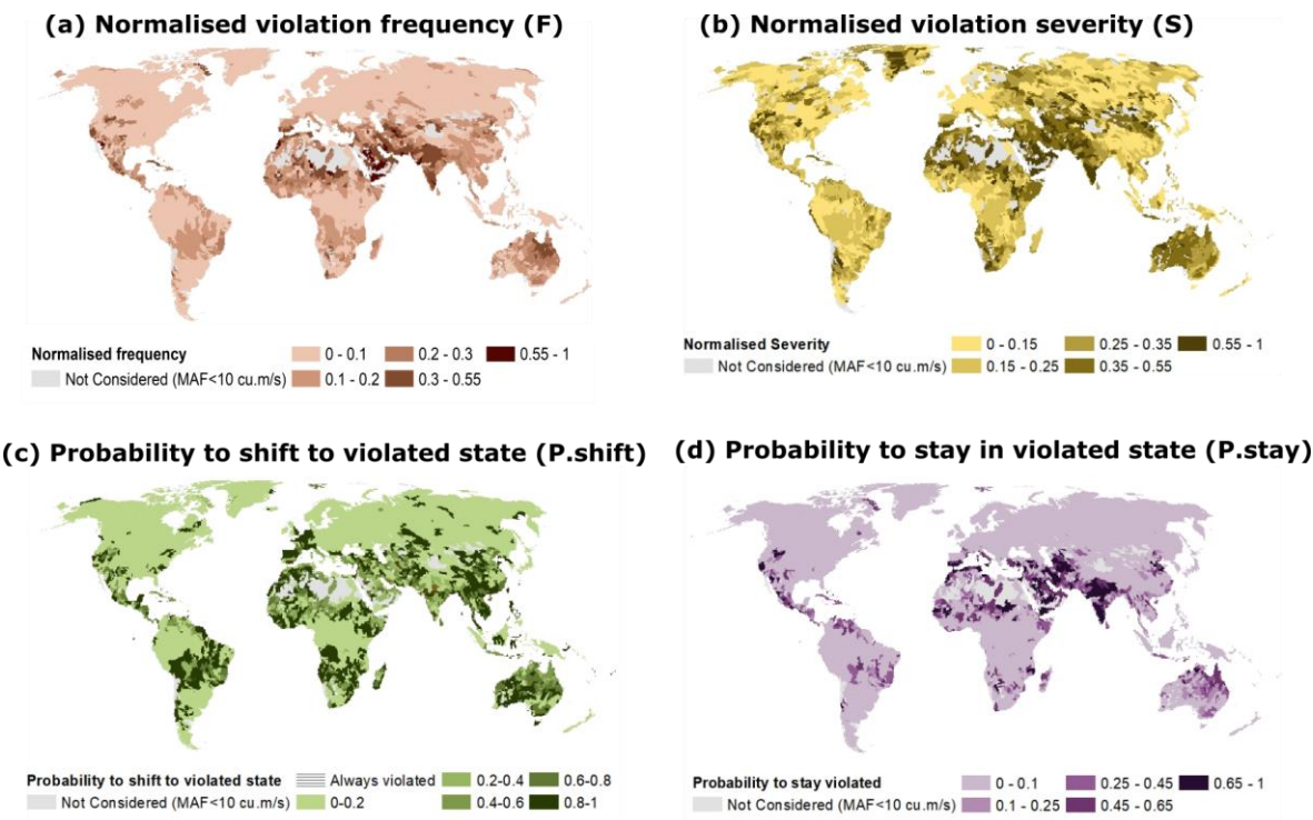
Fig. 2 Four measures of Environmental Flow Envelope (EFE) lower or upper bound violation estimated using ensemble median of four Global hydrological models; a) Normalized frequency of violation, b) Normalized severity of violation, c) Probability to shift to a violated state from a non-violated state and d) Probability to stay violated once shifted to a violated state.
