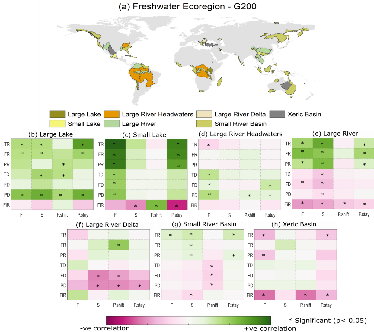
Fig.4 (a) Spatial distribution of different G200 freshwater ecoregions and (b-h) the correlation between EF violation indices and freshwater biodiversity indicators for different G200 freshwater ecoregions.
