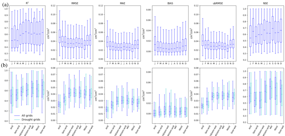
Figure 8: The accuracy metrics of 10-cross validation for R^2 , RMSE, MAE, BIAS, ubRMSE and NSE: (a) is averagely obtained on a month basis, and (b) is averagely obtained for each climate region and for the drought grids.
