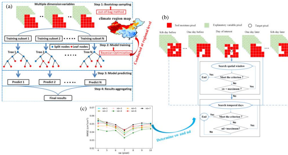
Figure 4: (a) The flowchart of the random forest model implemented for a multidimensional dataset. (b) The flowchart of spatiotemporal window determination strategy for random forest regression. (c) The results of the sensitive analysis regarding two maximum values, i.e., the size of the spatial window ( sw ) and the number of temporal days ( nd ), for terminating the searching process.
