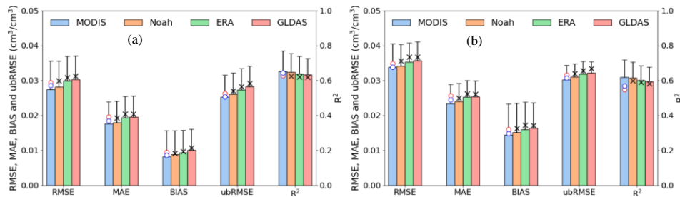
520 Figure 12: The accuracy metrics of models using different DTRs for (a) Northern China (NC) and (b) Southern China (SC). Error bars denote 1 \sigma errors. The symbol ‘x’ represents the accuracy metrics of the models without DTR correction procedure. The symbol ‘o’ in red represents the accuracy metrics of the models using GLEAM SM to replace ERA SM, and the symbol ‘o’ in blue represents the accuracy of the models using Noah SM to replace ERA SM.
