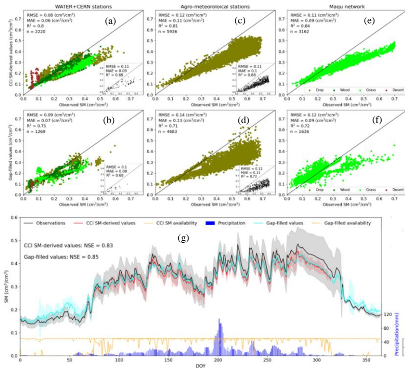
Figure 7: The evaluations of model results. (a), (c) and (e) are the scatter plots of 1-km CCI SM-derived values against field measures regarding WATER/CEERN, agro-meteorological stations, and Mauqu network, respectively, and (b), (d) and (f) are the scatter plots of 1-km gap-filled SM-derived values against field measures. The sub-figures in the upper corner of (a)-(d) are the scatter plots under extremely dry conditions. (g) are the time series of average CCI SM-derived values against site measures in the Mauqu region. The shaded area in (g) denotes \pm 1 standard error.
