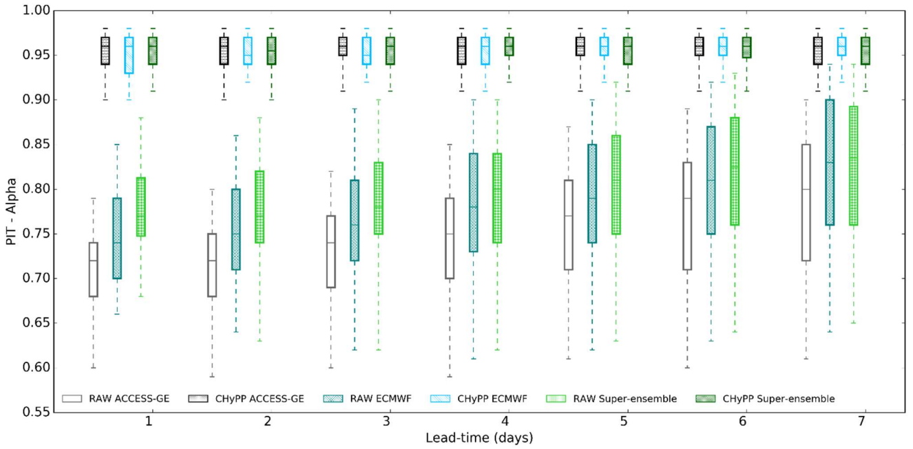
400 Figure 5. Reliability (PIT-alpha) of different rainfall products (raw and calibrated using CHyPP), ACCESS-GE2, ECMWF, and the super-ensemble for the 100 catchments.
